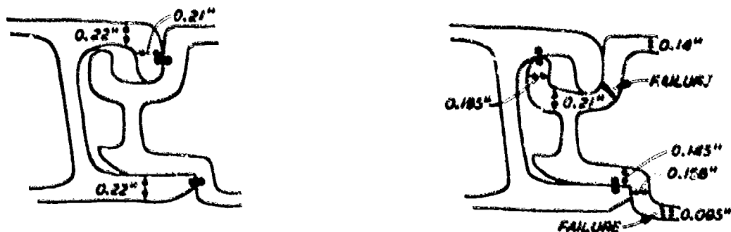
Figure 8 Configurations of joints in compressed and buckled positions
