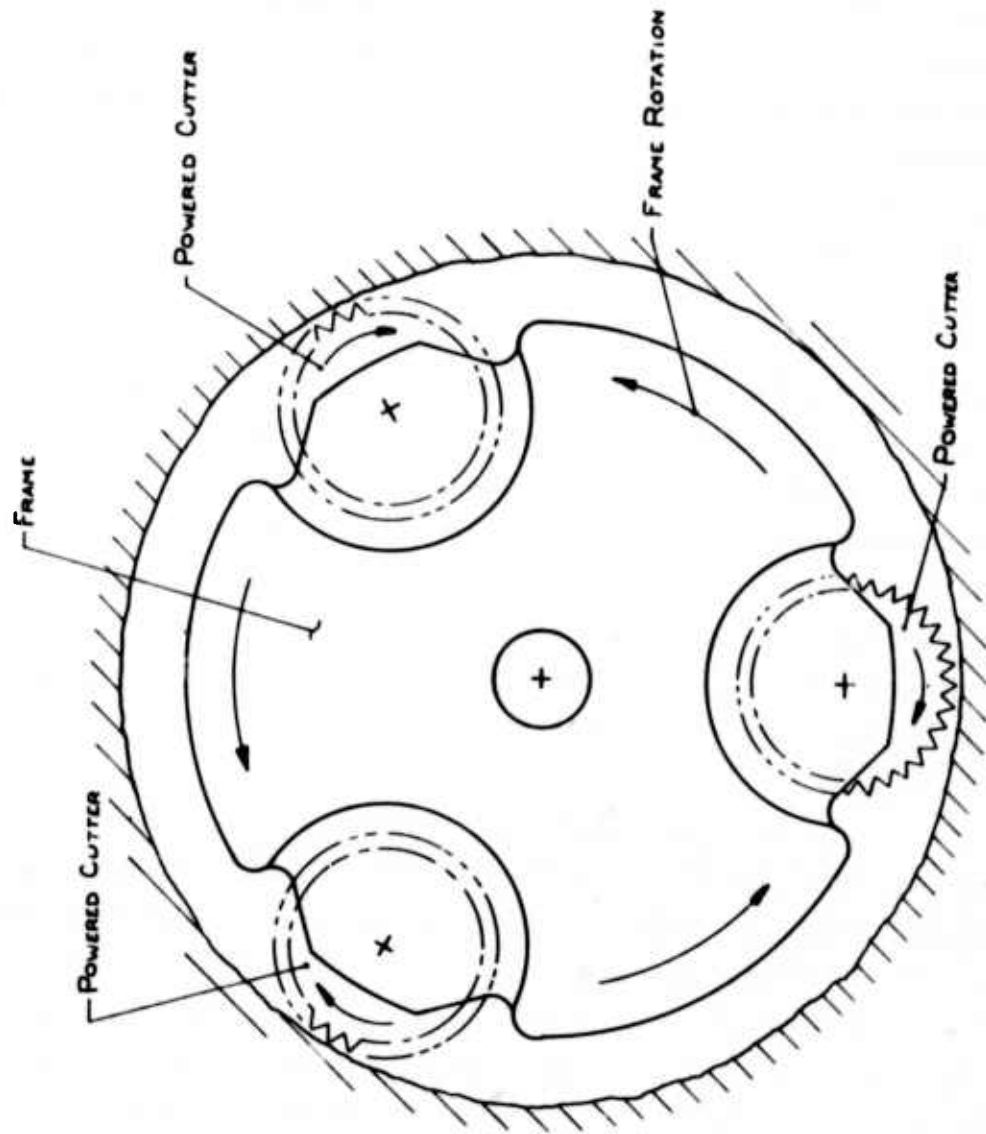
Torqueless Rotary Drive from Frame-Mounted Motors
