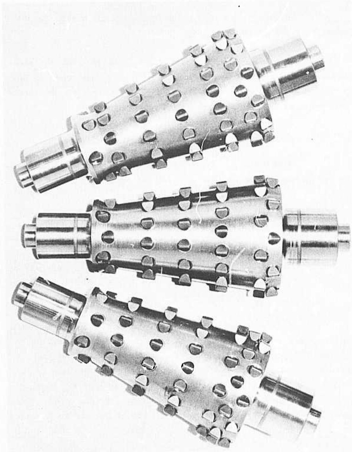
Completed Roller Cutters
