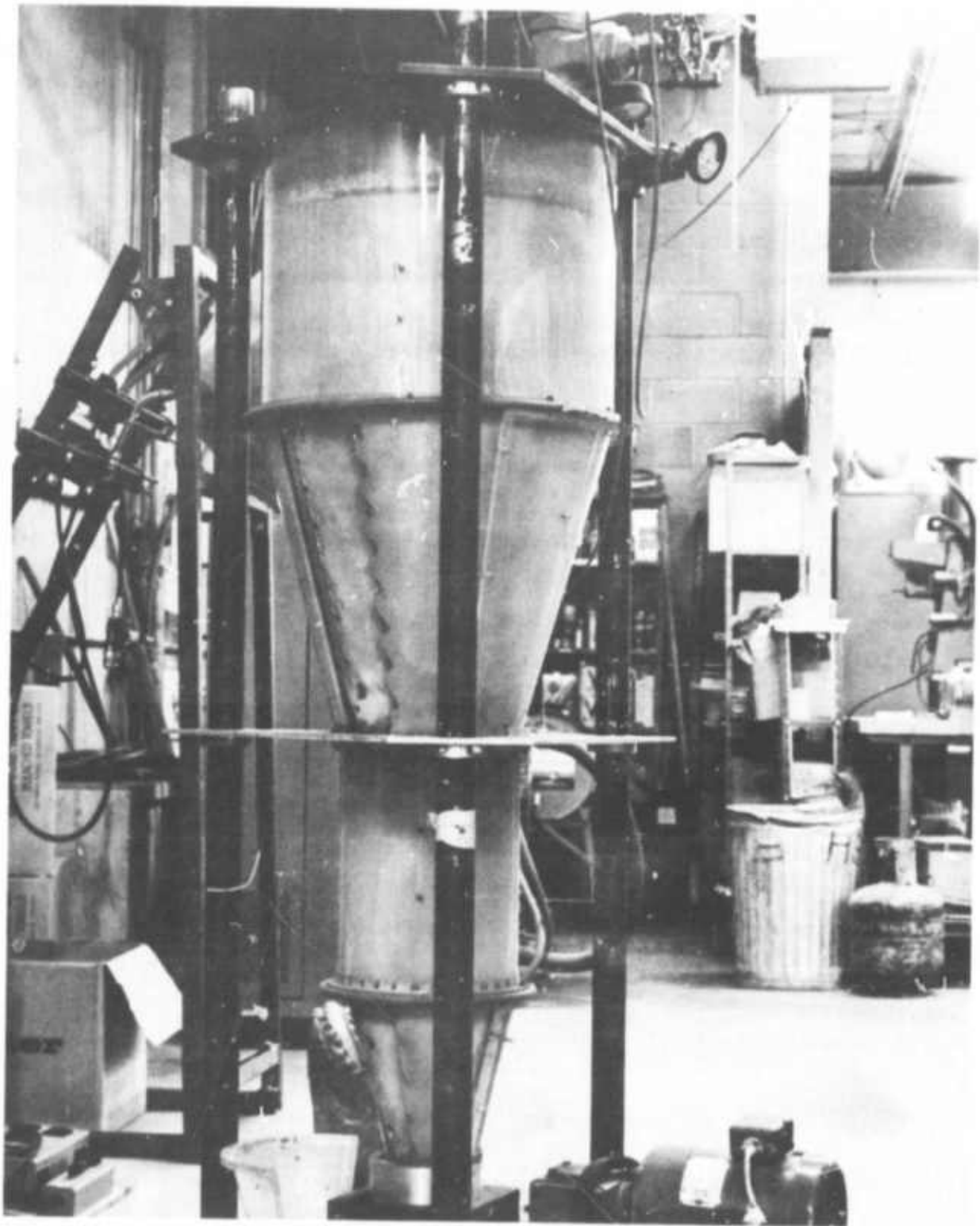
Photograph of Mucking System Model
