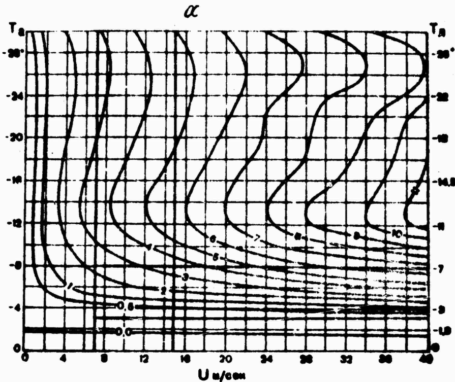
Fig. 8. Amount of Ice (g/hr) Which Can Form on 1 Sq Cm of Surface During Icing of a Ship. a- flat surface, T_w = 1.7^\circ ; S = 34^\circ/\text{oo} ; L_{3am}^* = 4.0 ; L_{ncn}^{**} = 601 + 700 ; C_i = 0.6 - 36.5 . b- cylindrical surface, T_w = -1.7^\circ , S = 34^\circ/\text{oo} ; L_{3am} = 4.0 ; L_{ncn} = 601 + 700 ; C_r = 0.6 + 30 . c- flat surface, T_w = -1.7^\circ ; S = 34\% ; L_{3am} = 4.0 ; L_{ncn} = 601 + 700 ; C_r = 1.0 + 36.5 . d- flat surface, T_w = 2^\circ , S = 34^\circ/\text{oo} ; L_{3am} = 4.0 ; L_{ncn} = 601 + 700 ; C_r = 0.6 + 36.5 . * [Here and elsewhere, subscript "3am" = "freezing"] ** [ " " " " "ncn" = vaporization.]
