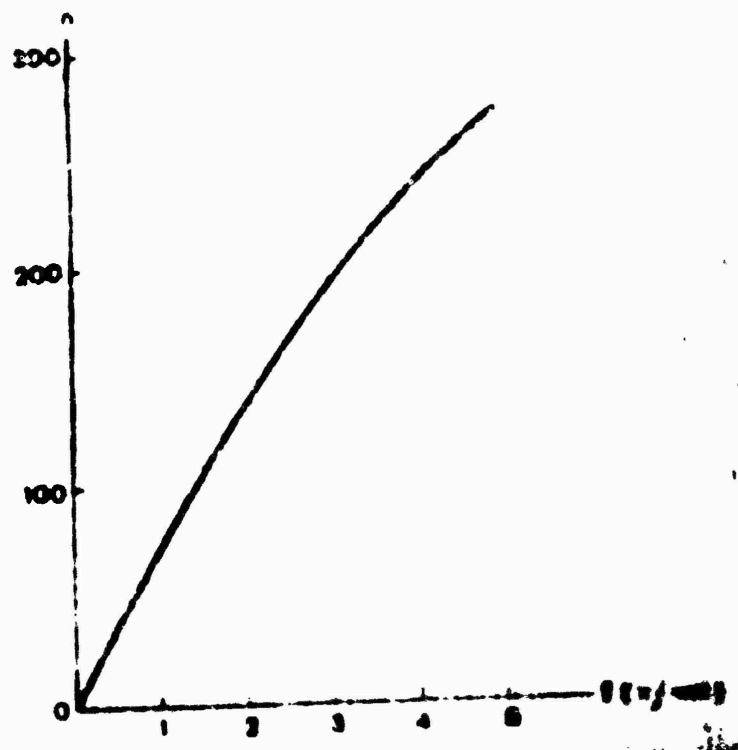
Fig. 14. Curve Showing Dependence of Icing Rate of Ships of MFT Type and of Ships Having Similar Dimensions, on n-Value.
