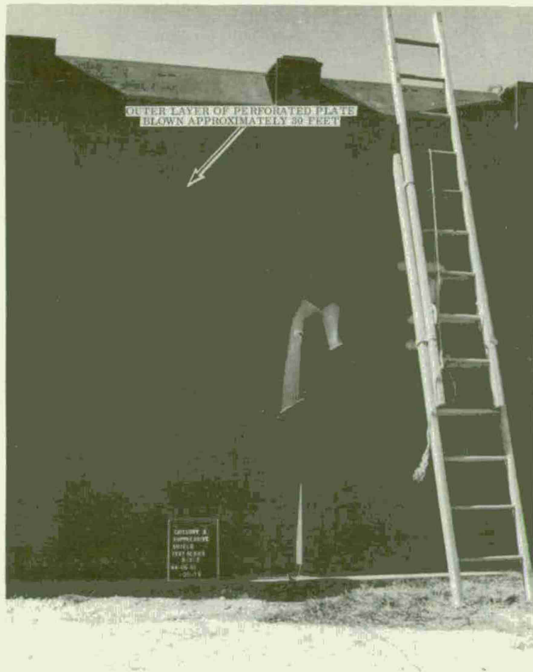
Figure 14. Category 3 S/S Damage From Test B3-2, Right Side
