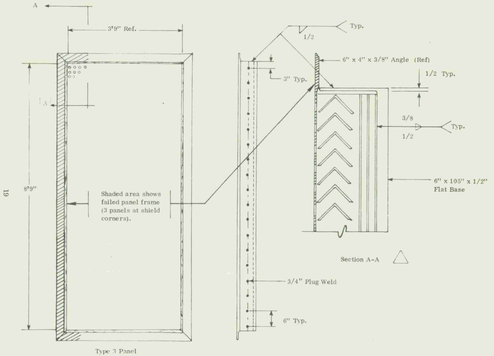
Figure 7. Category 3 Test B3-1 Proof Pressure Test - Diagram of Panel Frame Failure
