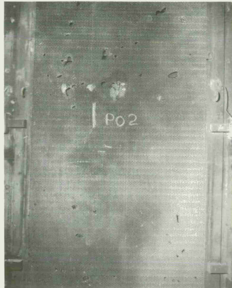
Figure 26. Category 3 Test B2-1, Typical Fragment Damage
