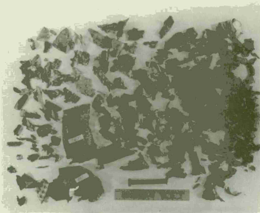
Figure 23. Category 3 16-Gauge Stainless Steel Hopper Fragmentation Threat
