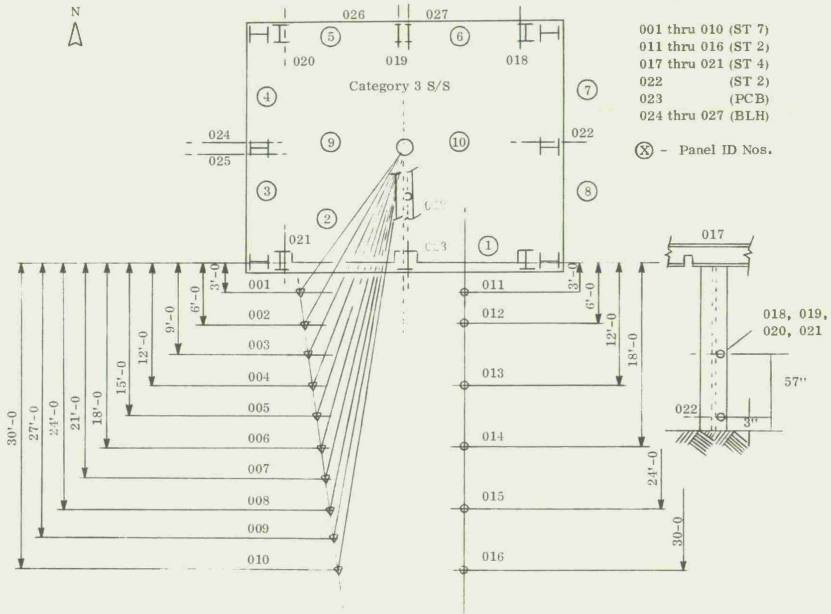
Figure 5. Category 3 Transducer Locations Tests B2-2 and B3-2
