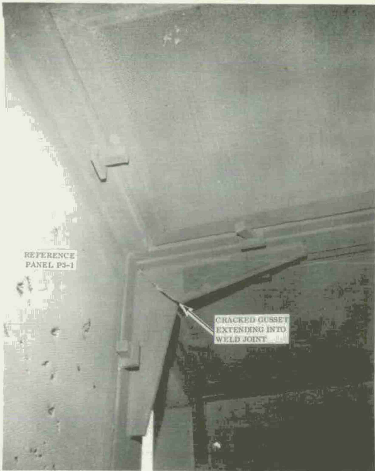
Figure 10. Category 3 Test B3-1 Proof Pressure Test - Damaged Gusset in Wall Column to Roof Beam Intersection
