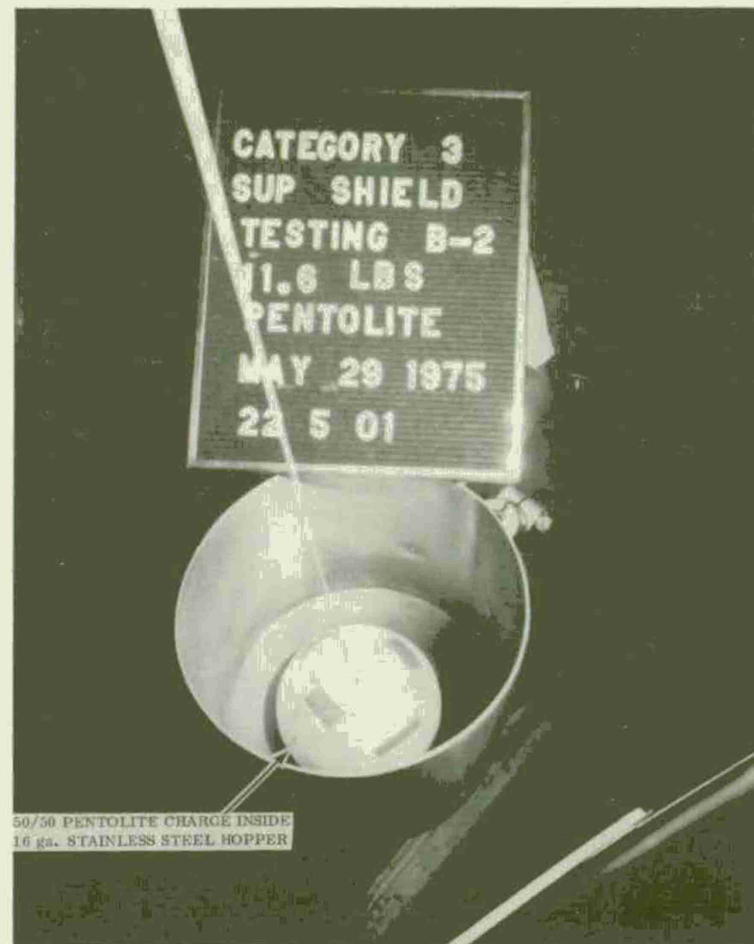
Figure 2. Category 3 Candidate Operation Test B2-1. Pentolite Charge Suspended in 16-Gauge Stainless Steel Hopper From Press-Pelletizing Operation at Lonestar Army Ammunition Plant.
