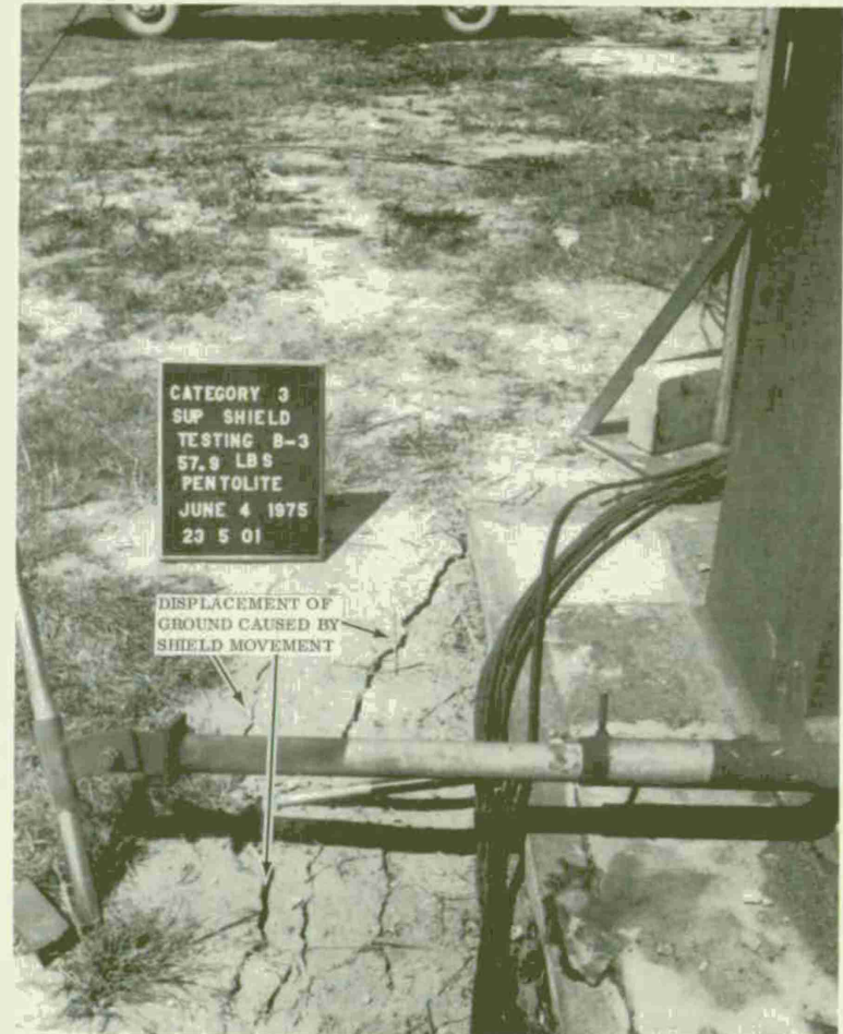
Figure 9. Category 3 Test B3-1 Proof Pressure Test - Relative Horizontal Motion of Structure
