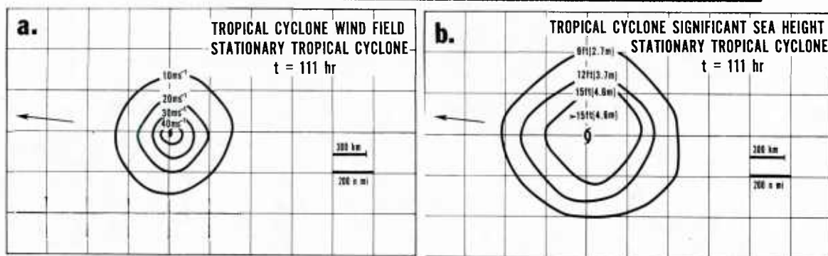
Figure 6. Wind wave model results at t = 111 \text{ hr} for a stationary [(a) and (b)], slow [ 3.2 \text{ ms}^{-1} (6.2 kt)] [(c) and (d)], and fast [ 9.5 \text{ ms}^{-1} (18.5 kt)] [(e) and (f)] tropical cyclone. Tropical cyclone input parameters are also shown. Distributions near the storm center are not shown.
