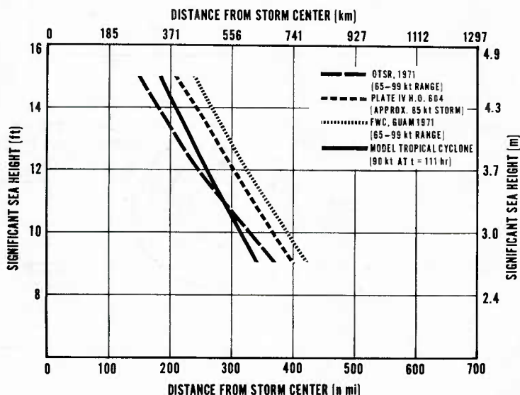
Figure 2. Comparisons of the sea height around tropical cyclones in the western North Pacific for a similar intensity category.
