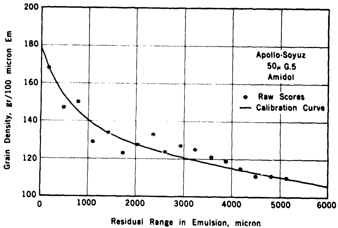
Grain Density/Range Function for Proton Enders in G.5 Emulsion 1B-2 Flown on Apollo-Soyuz
