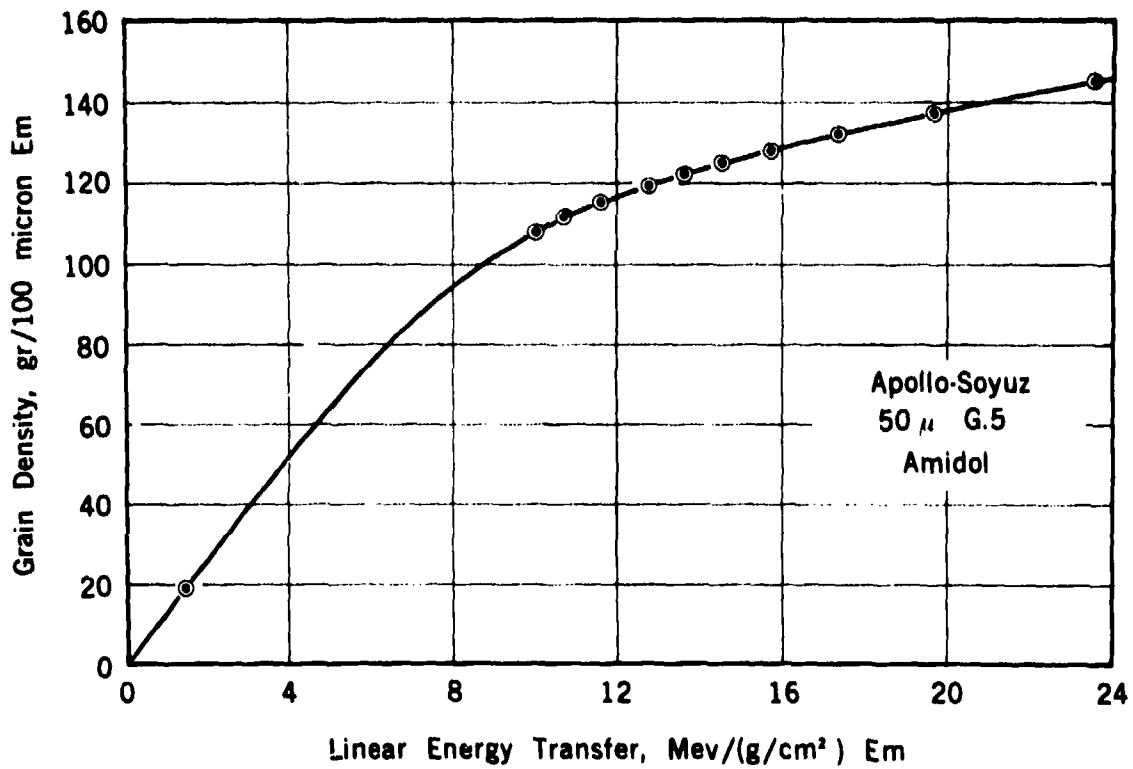
Grain Density/LET Calibration for Emulsion 1B-2 Flown on Apollo-Soyuz
