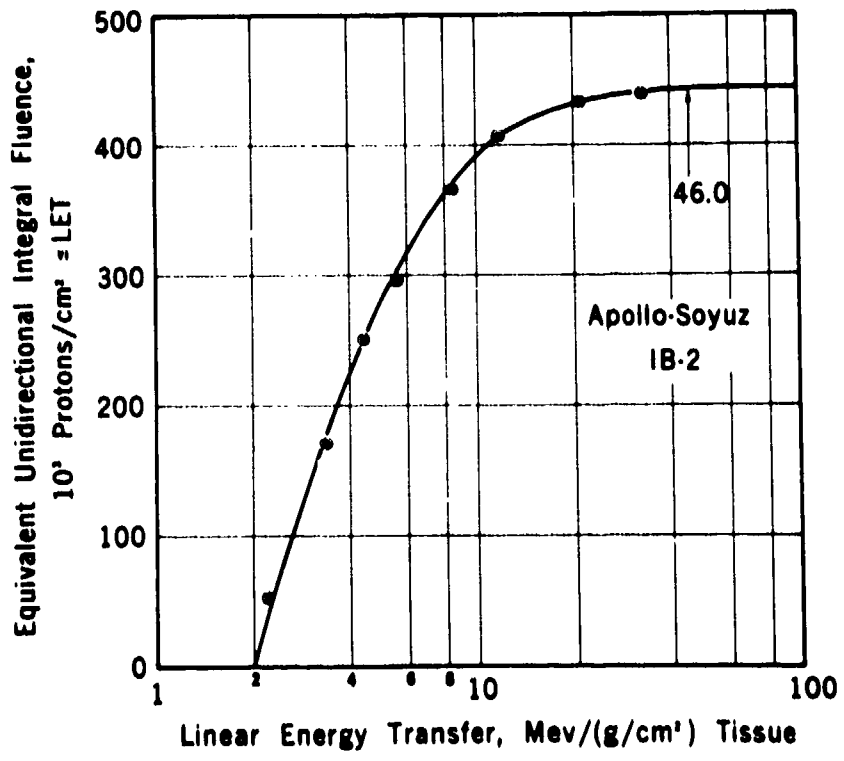
Integral LET Spectrum of Proton Exposure on Apollo-Soyuz
