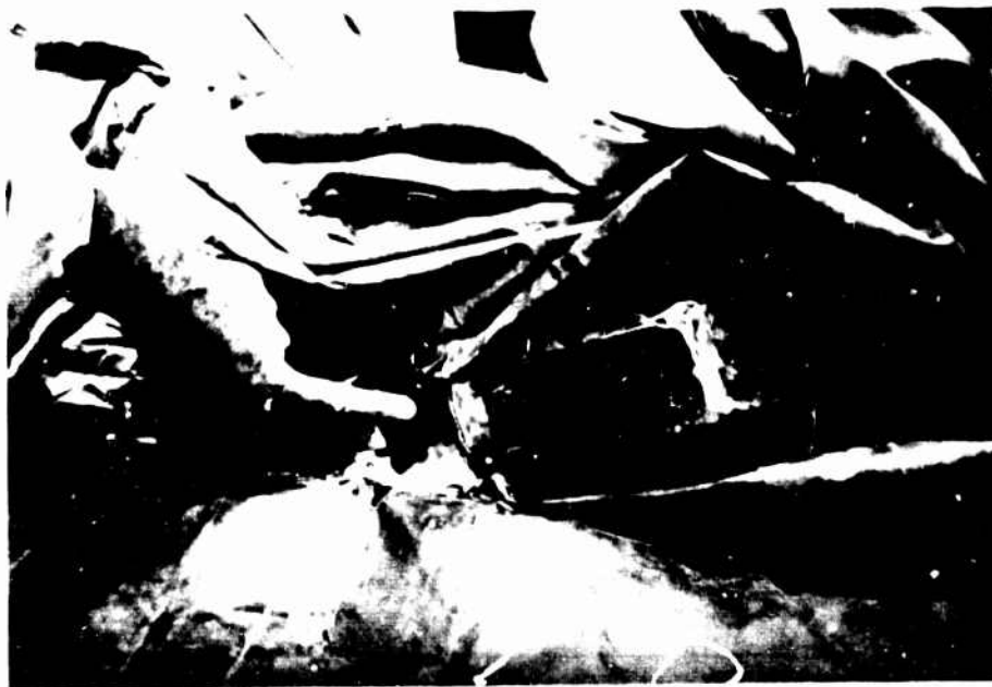
Figure 19. Delamination of Adhesive Bond Joining the Sides and Floor of Shelter Section IP-2
