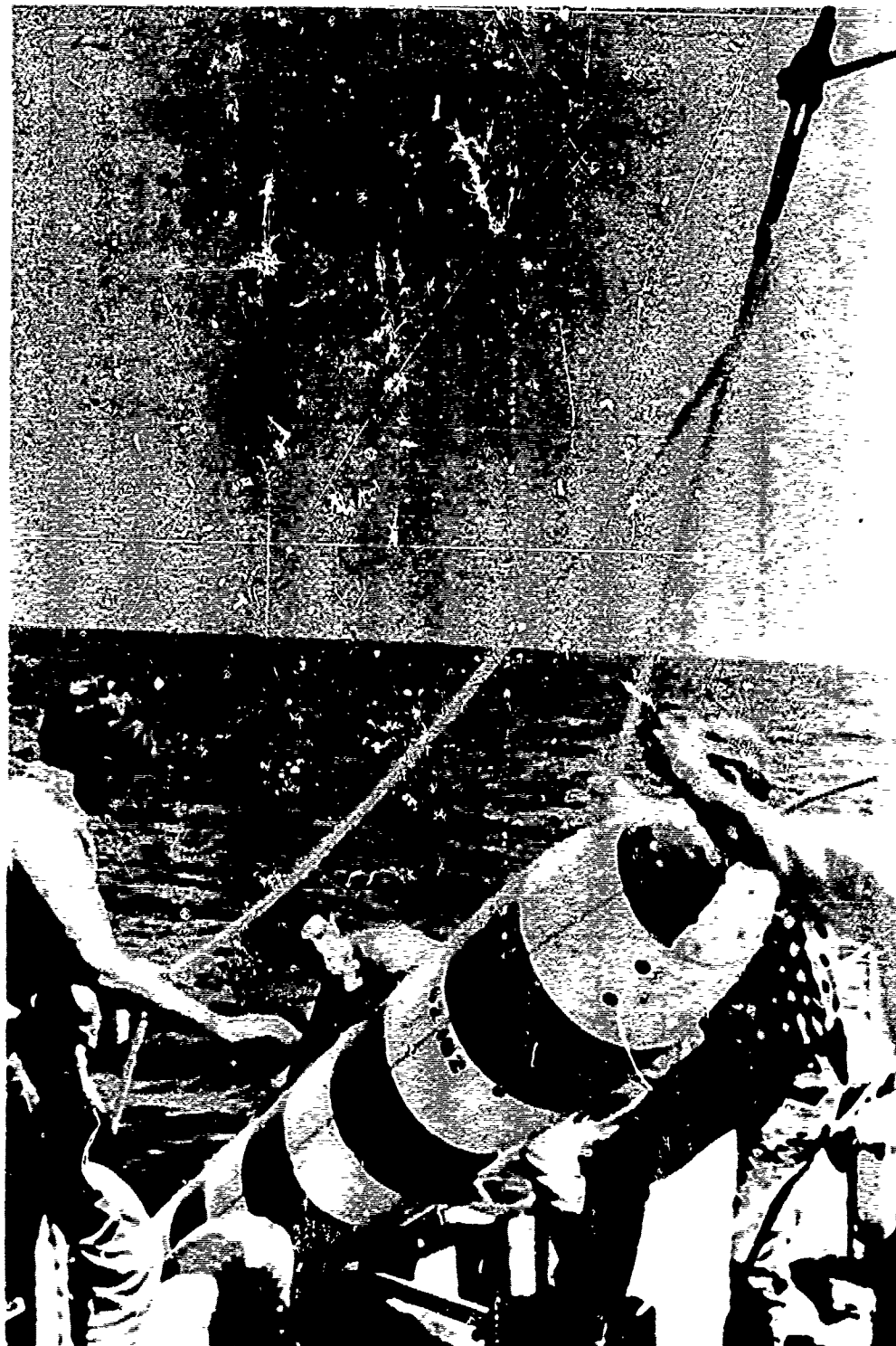
Figure 11. (a) Somochev is a buoyancy-actuated system that measures ambient noise and other environmental parameters at depths to 20,000 feet (6,100 meters).
