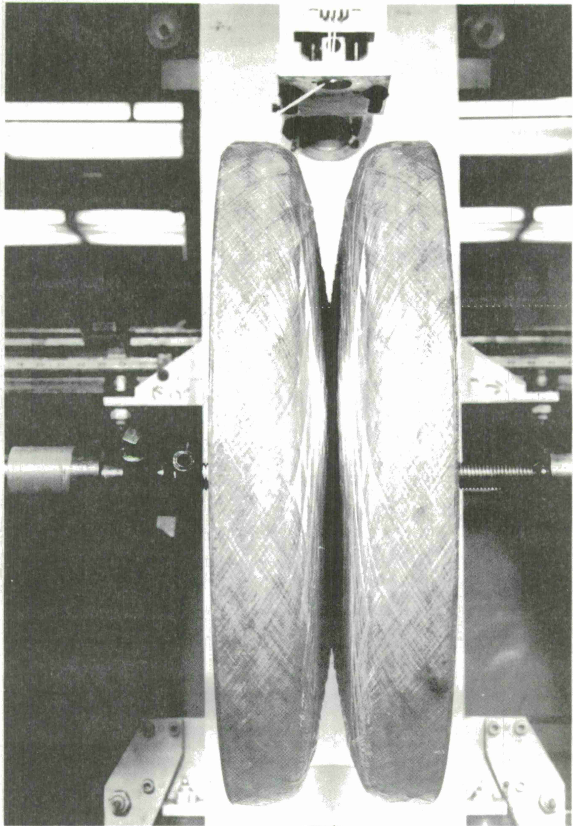
Figure 18. Composite road wheel disks after separation from mandrel and placed back to back for further winding.
