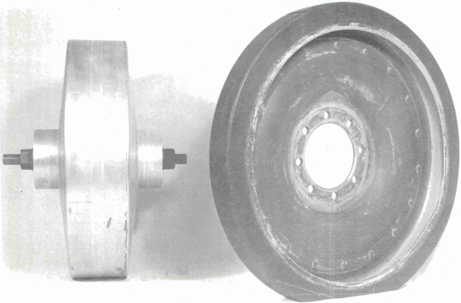
Figure 16. Composite road wheel mandrel and M113 disk.
