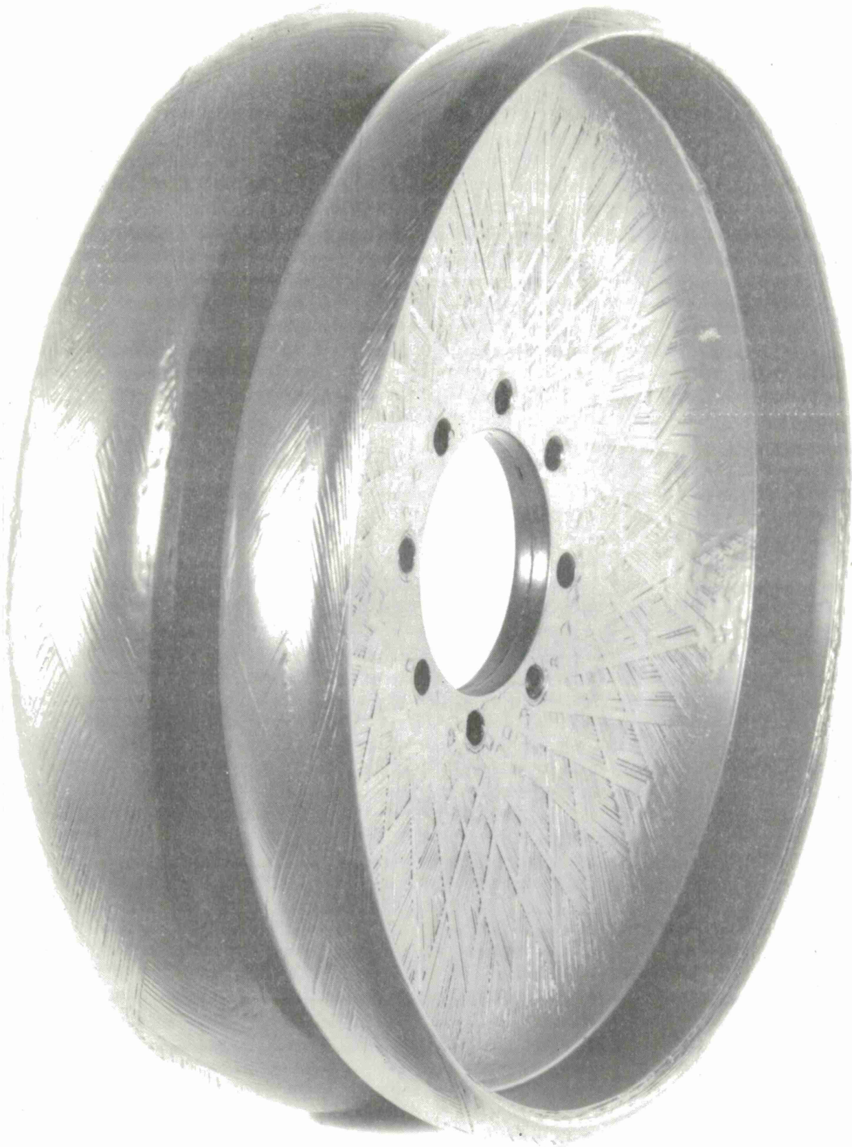
Figure 2. Side view of prototype composite road wheel.
