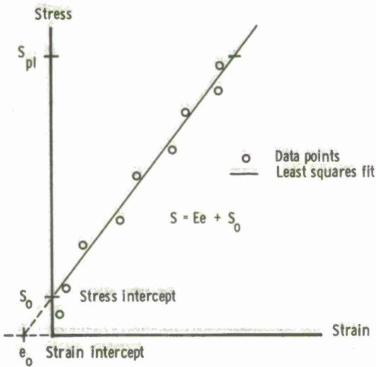
Figure 2. Stress and strain intercepts of least-squares straight-line fit of elastic data (schematic).
