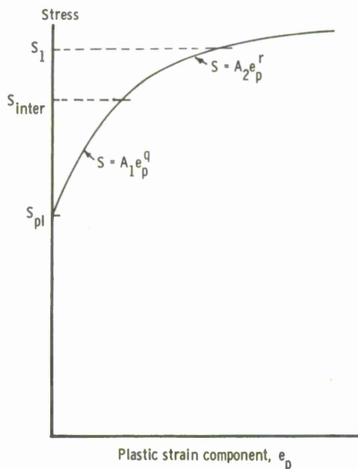
Figure 5. Two-equation analytical description of plastic strain components with a variable intermediate boundary stress (schematic).
