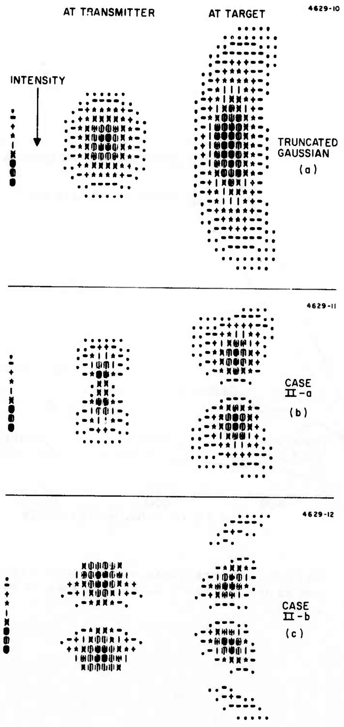
Figure 6. Pseudo-gray sacle plots of transmitter and focal-plane (target) irradiance distributions for the three beams in Fig. 1. A moderate amount of thermal blooming is present in the propagation path.
