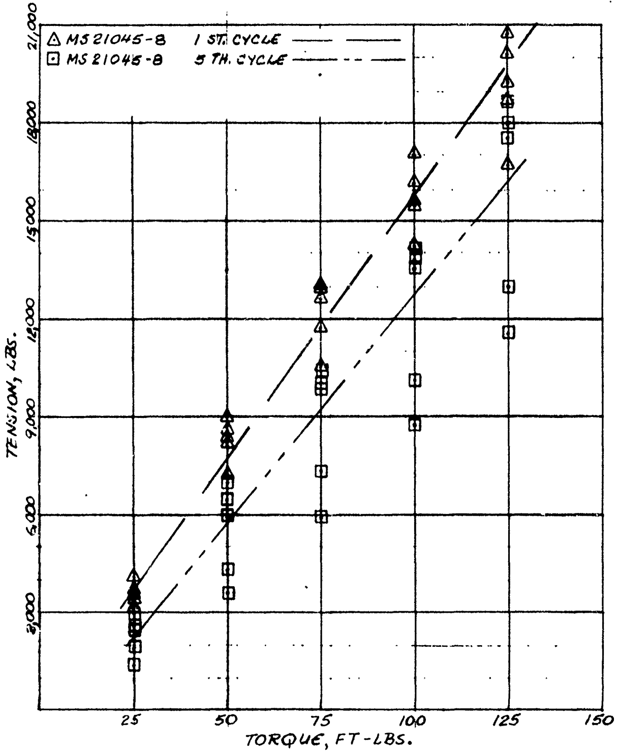
FIGURE 28. TORQUE-TENSION RELATIONSHIP FOR MS 21045-8
