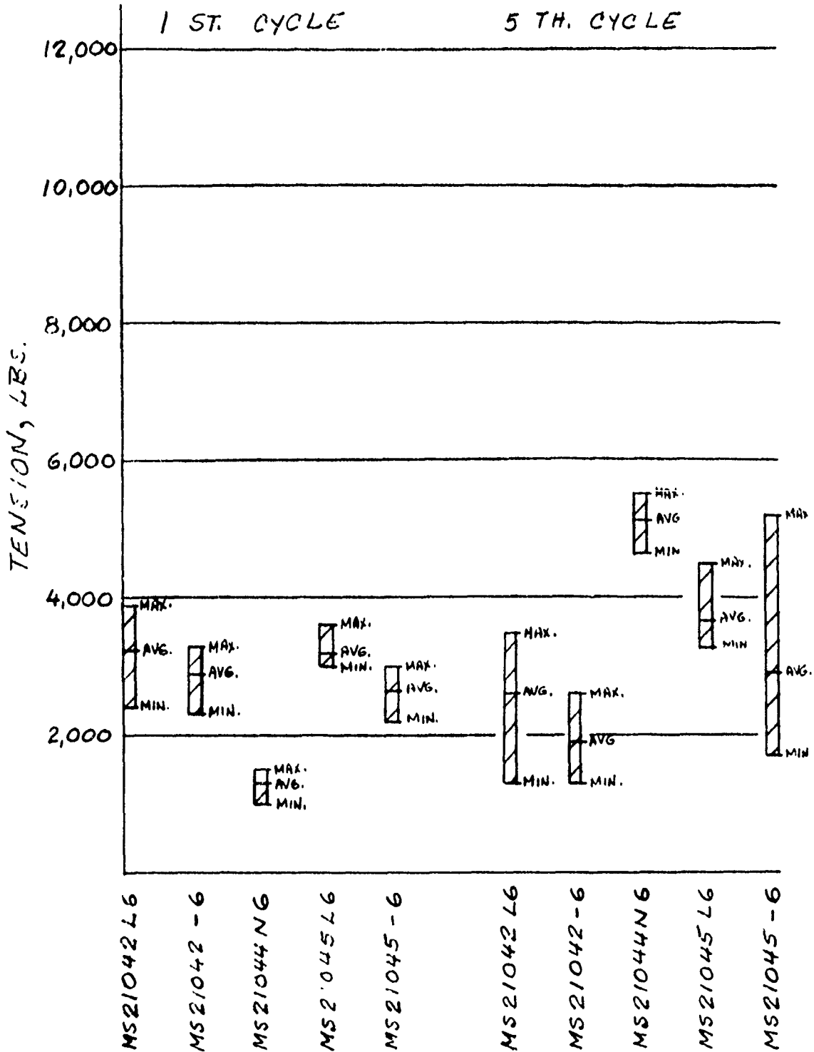
FIGURE #0. COMPARATIVE TORQUE-TENSION RELATIONSHIP FOR 3/8 SIZE NUTS TORQUED TO 200 IN-LBS.
