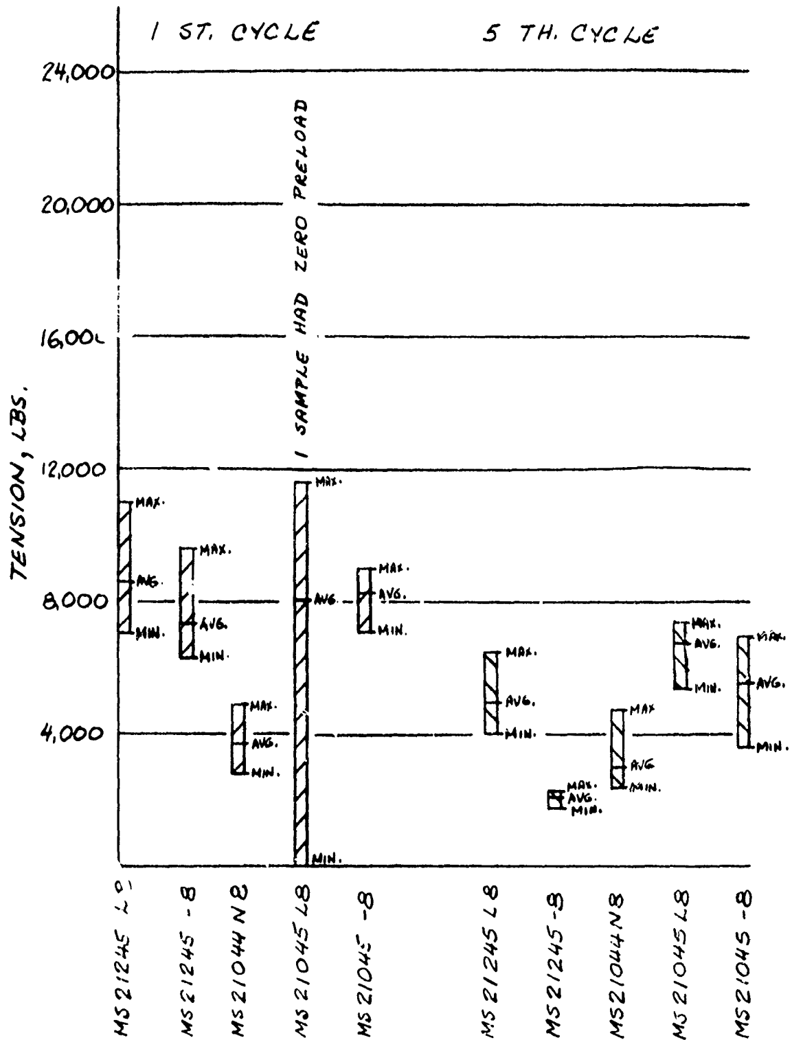
FIGURE 44. COMPARATIVE TORQUE-TENSION RELATIONSHIP FOR 1/2 SIZE NUTS TORQUED TO 50 FT-LBS
