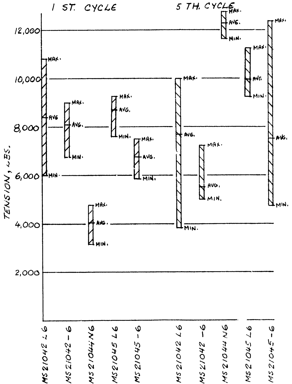
FIGURE 43. COMPARATIVE TORQUE-TENSION RELATIONSHIP FOR 3/8 SIZE NUTS TORQUED TO 500 IN-LBS.
