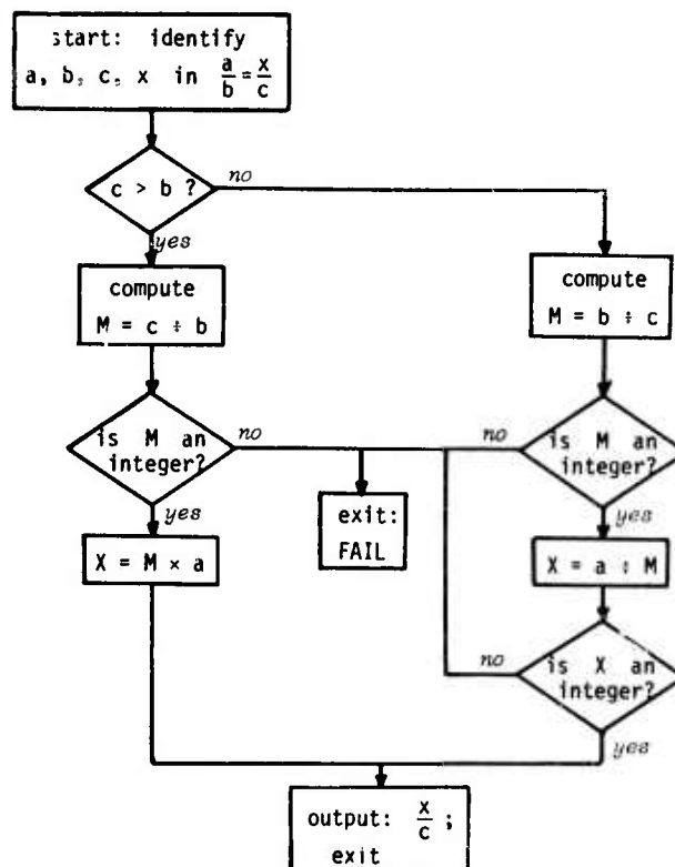
FIG. 7 Procedure for finding equivalent fractions, operating directly on numerical representations.
