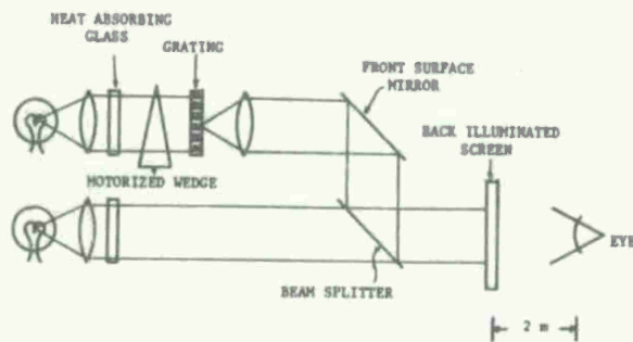
Figure 4. Schematic of Experimental Setup.
