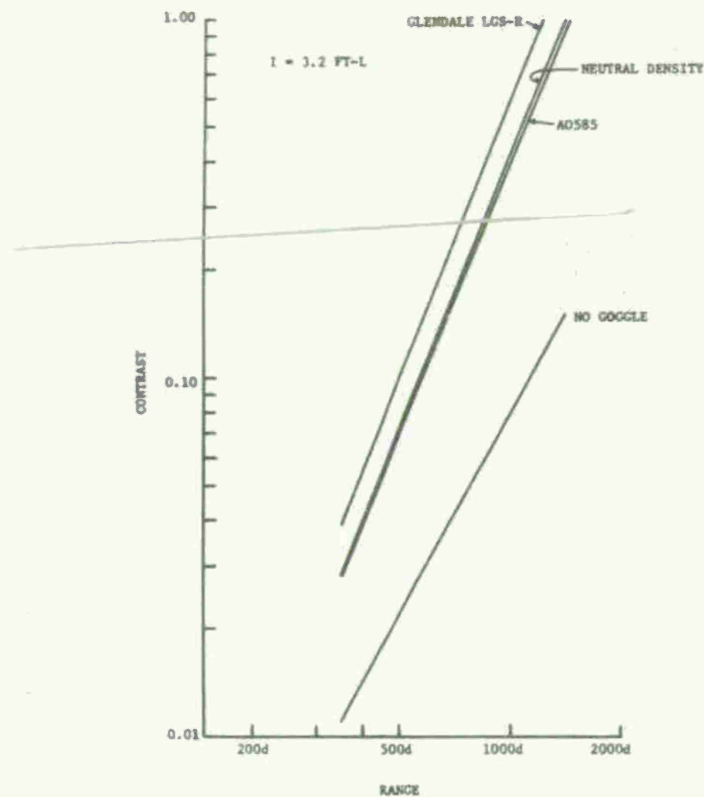
Figure 10. Target-Background Contrast Required for 50% Probability of Detection as a Function of Range and Target Diameter d with Background Luminance of 3.2 FT-L.
