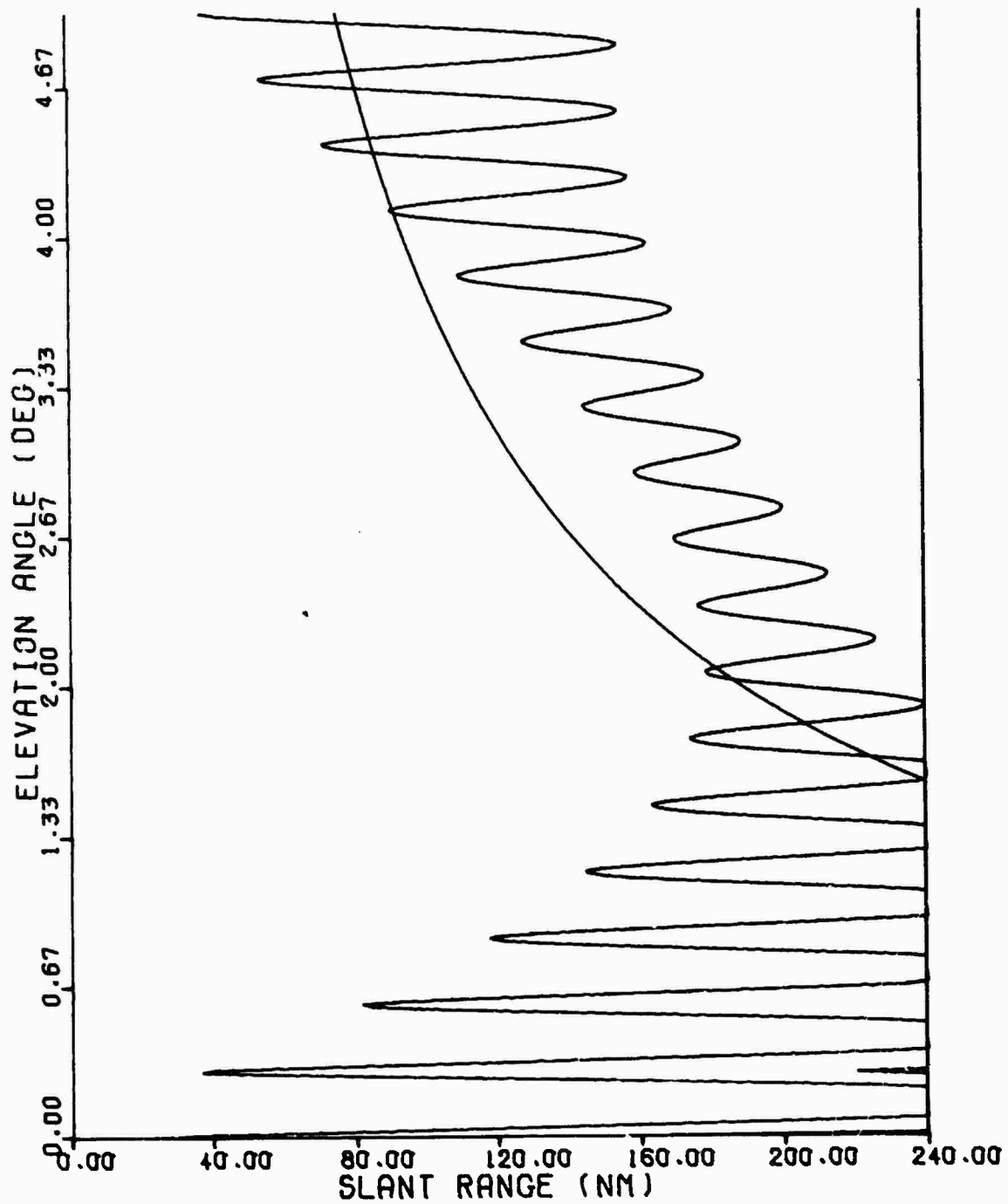
Figure 6.13 Vertical Lobing Contours, System 3
