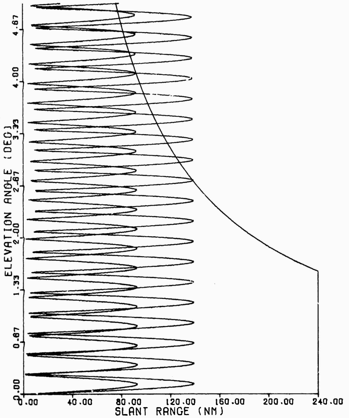
Figure 6.16 False Suppression Contours, System 1
