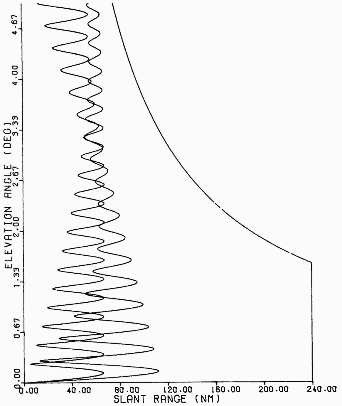
Figure 6.18 False Suppression Contours, System 3
