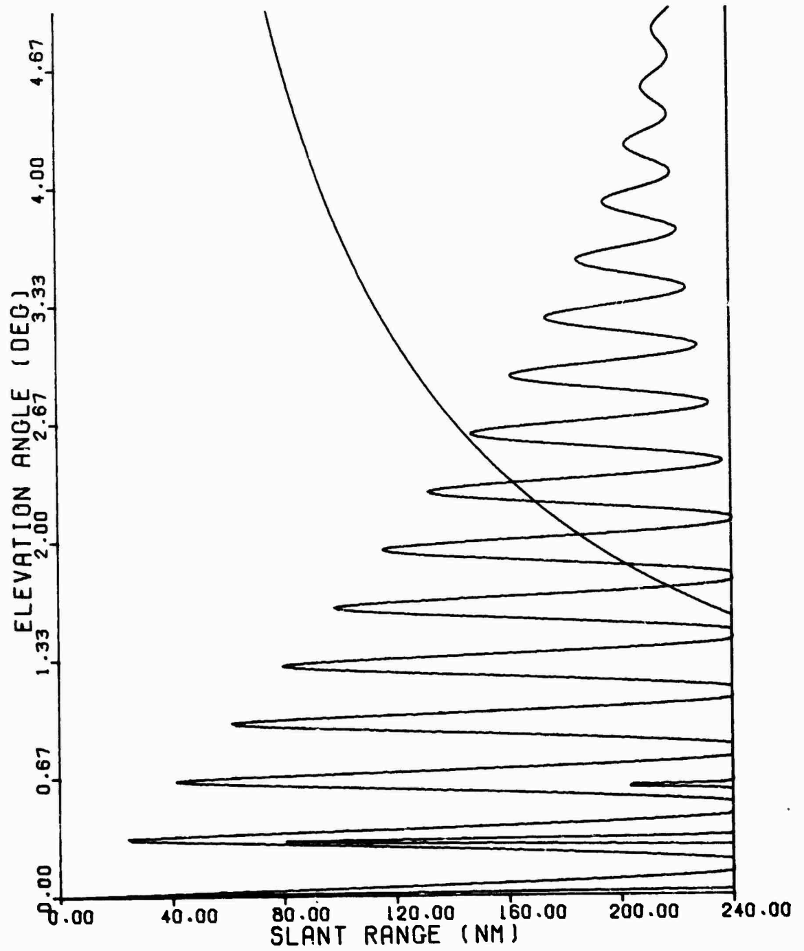
Figure 6.15 Vertical Lobing Contours, System 5
