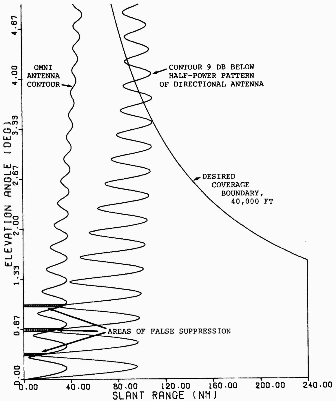
Figure 3.2 False Suppression of a Valid Target
