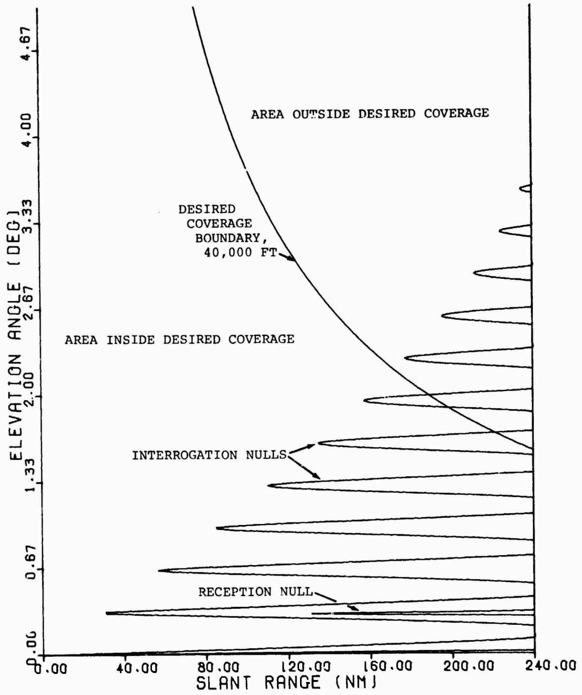
Figure 3.1 Typical Vertical Lobing Contours
