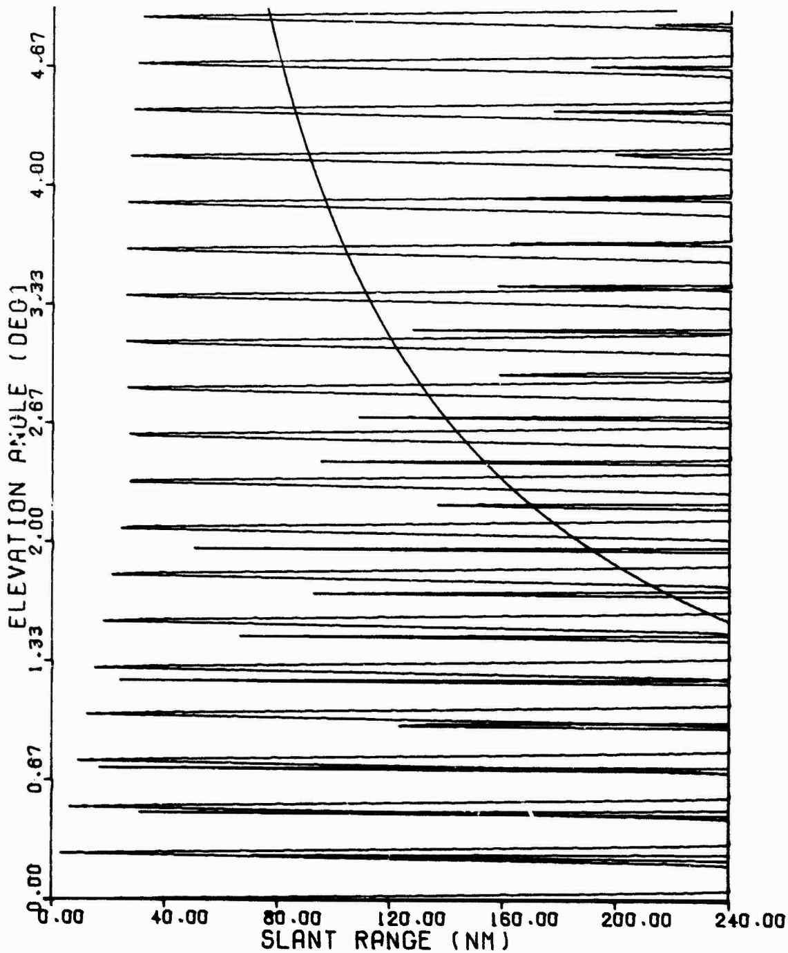
Figure 6.11 Vertical Lobe Contours, System 1
