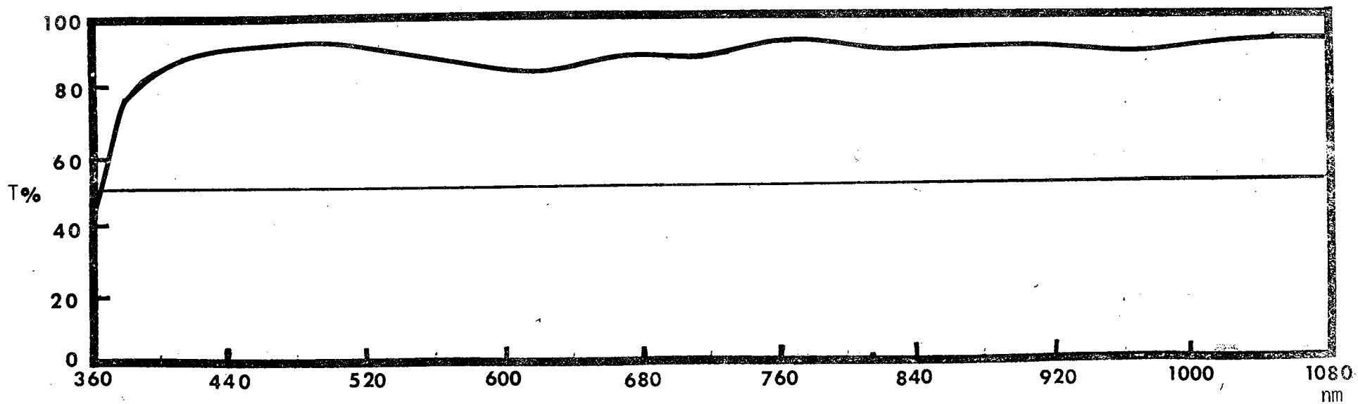
Figure 4: Spectral Transmittance of U8D/U8F (Seminole)
