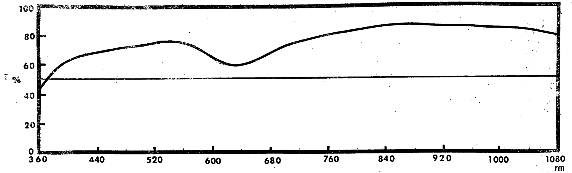
Figure 5: Spectral Transmittance of T-41 (Cessna) formed edge
