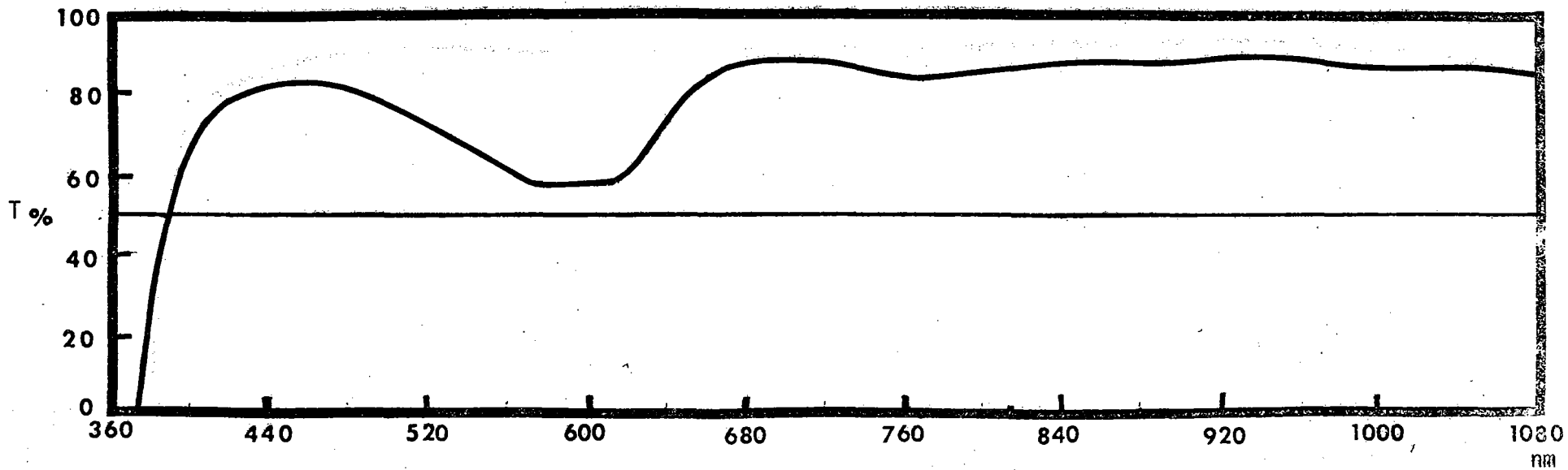
Figure 15: Spectral Transmittance of AH-1G (Hueycobra) (tinted)
