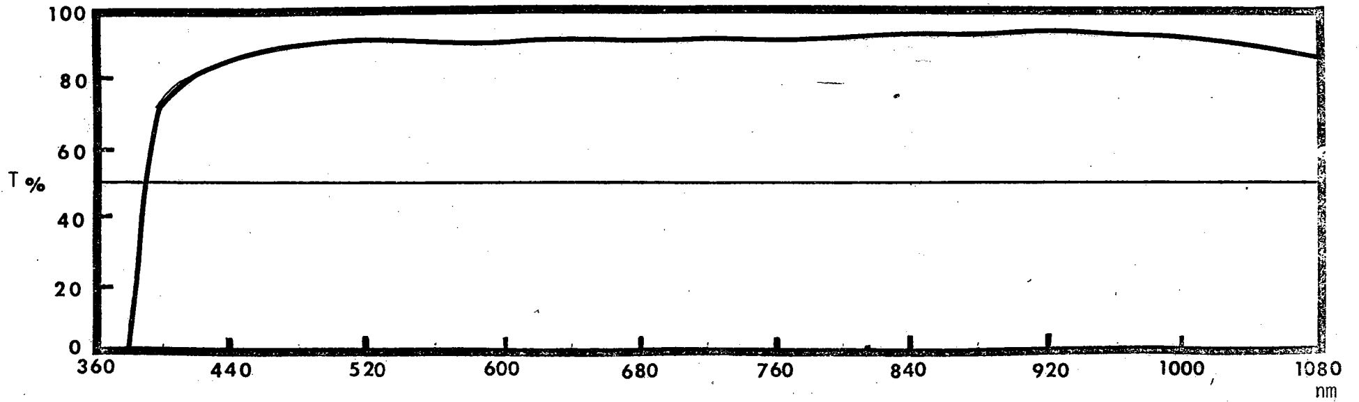
Figure 11: Spectral Transmittance of UH-1 (Iroquois)
