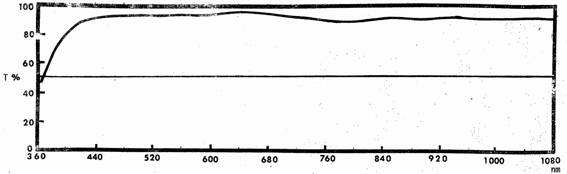
Figure 1: Spectral Transmittance of OI (Bird Dog)
