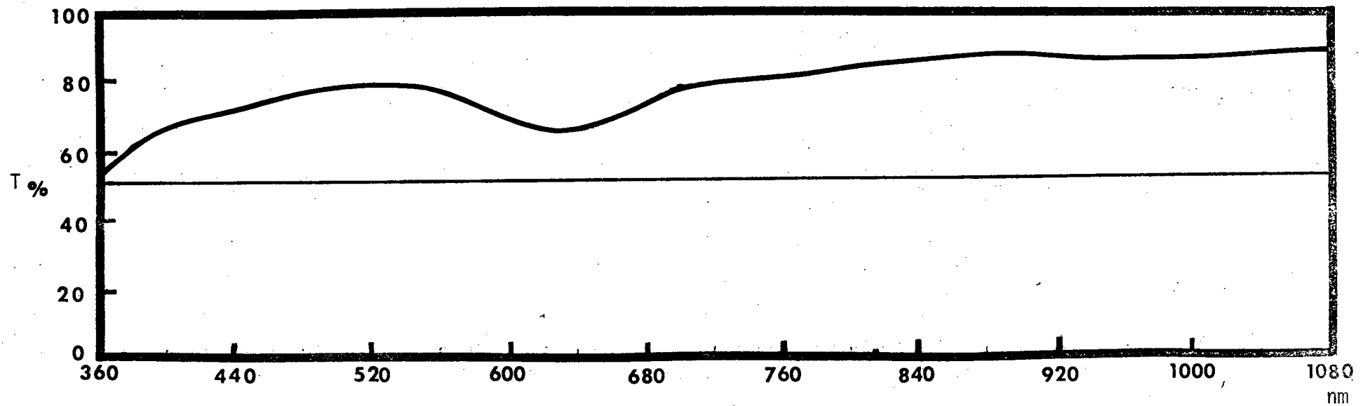
Figure 6: Spectral Transmittance of T-41 (Cessna) flat-unformed edge
