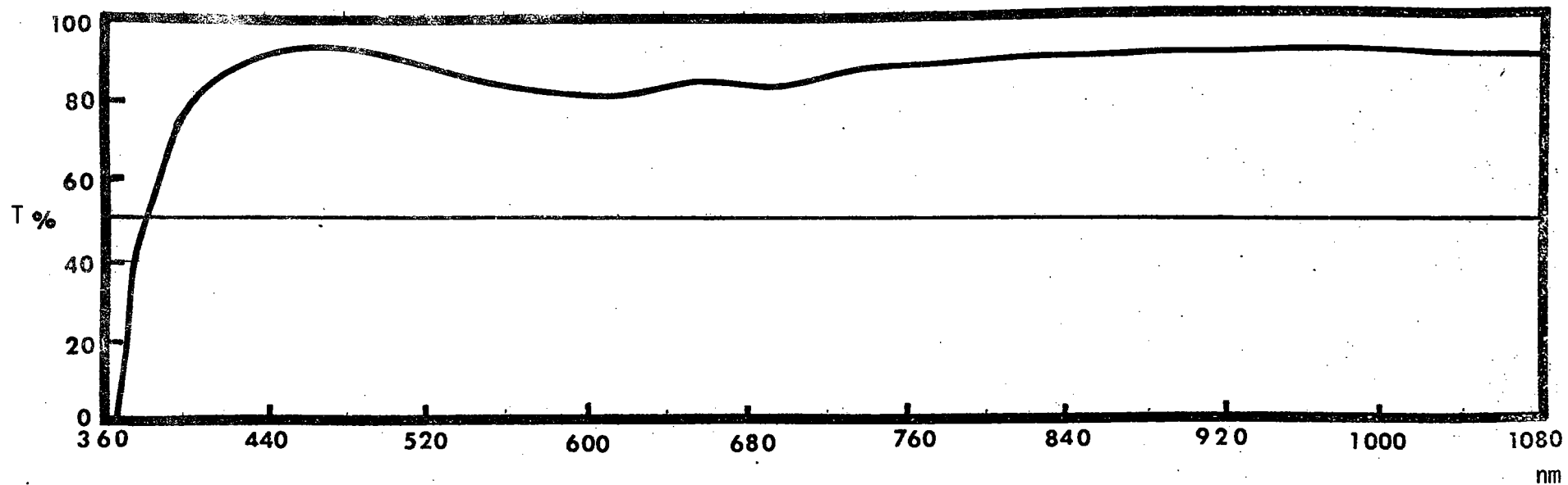
Figure 8: Spectral Transmittance of TH-13 (Sioux)
