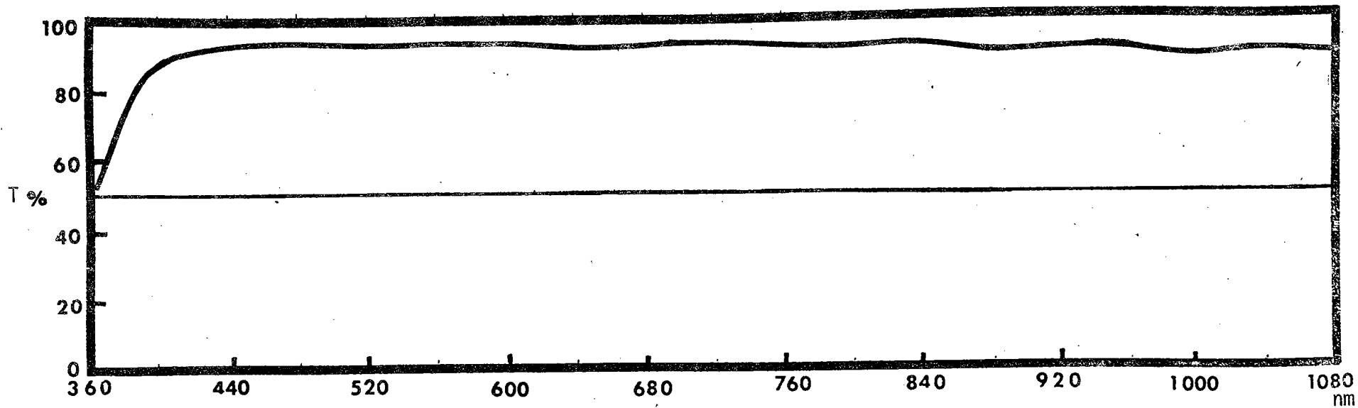
Figure 3: Spectral Transmittance of U6 (De Havilland)
