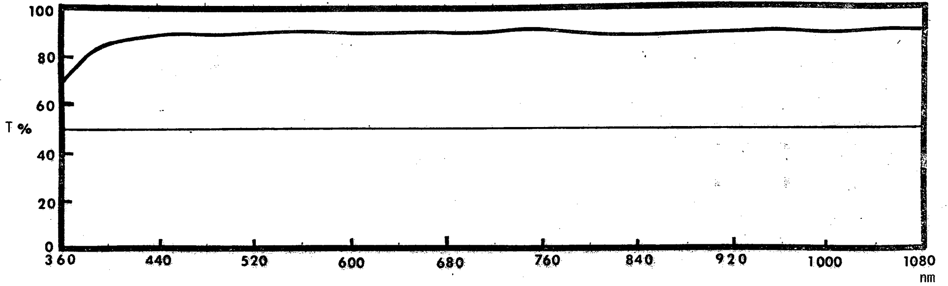
Figure 10: Spectral Transmittance of OH-58 (Kiowa)
