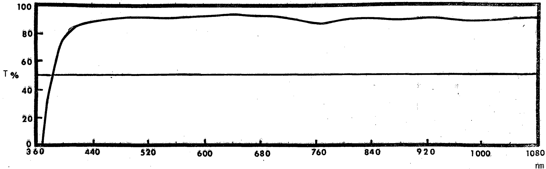
Figure 14: Spectral Transmittance of AH-1G (Hueycobra) (clear)
