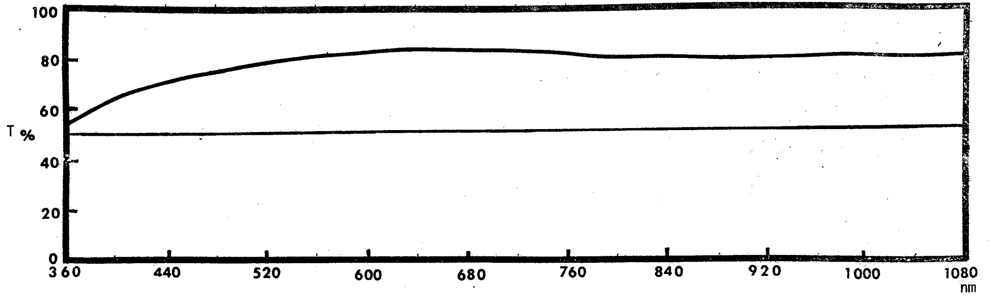
Figure 7: Spectral Transmittance of T-42
