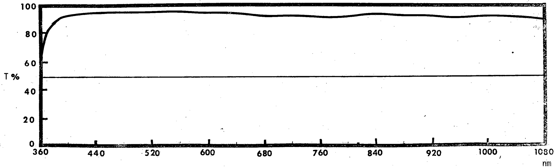
Figure 9: Spectral Transmittance of TH-55/OH6A (Cayuse)
