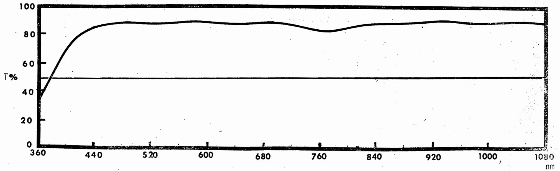
Figure 2: Spectral Transmittance of OV-1 (Mohawk)
