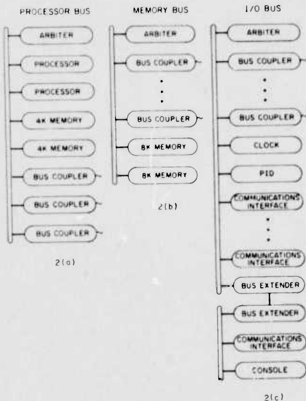
Figure 2 Bus structures
