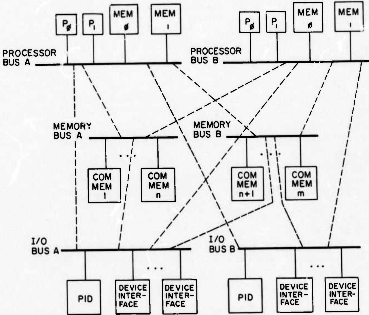
Figure 1 Typical Pluribus System Configuration
