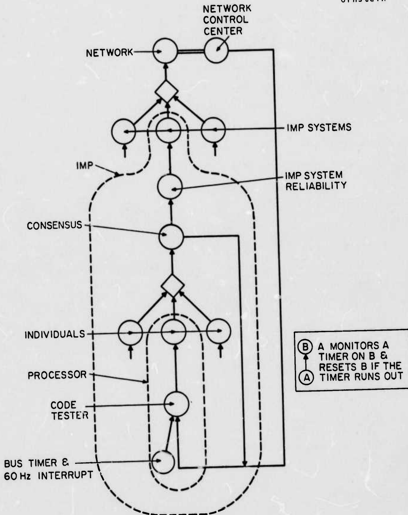
FIGURE 1 RELIABILITY STRUCTURE
