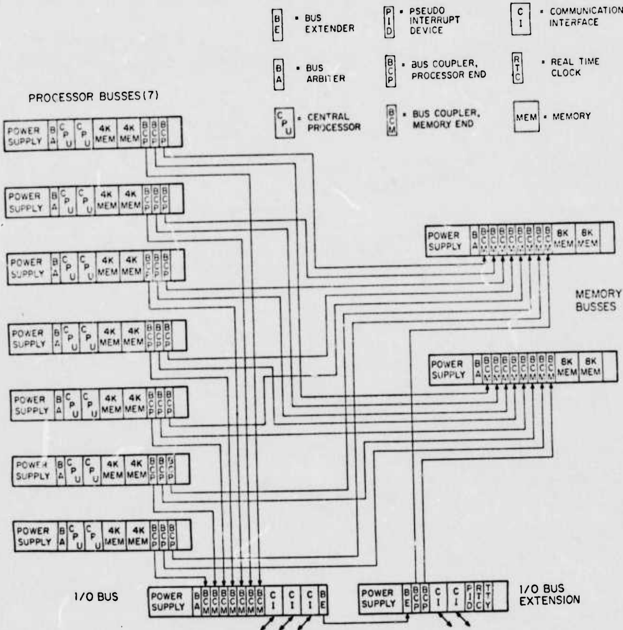
Figure 3—Prototype system
