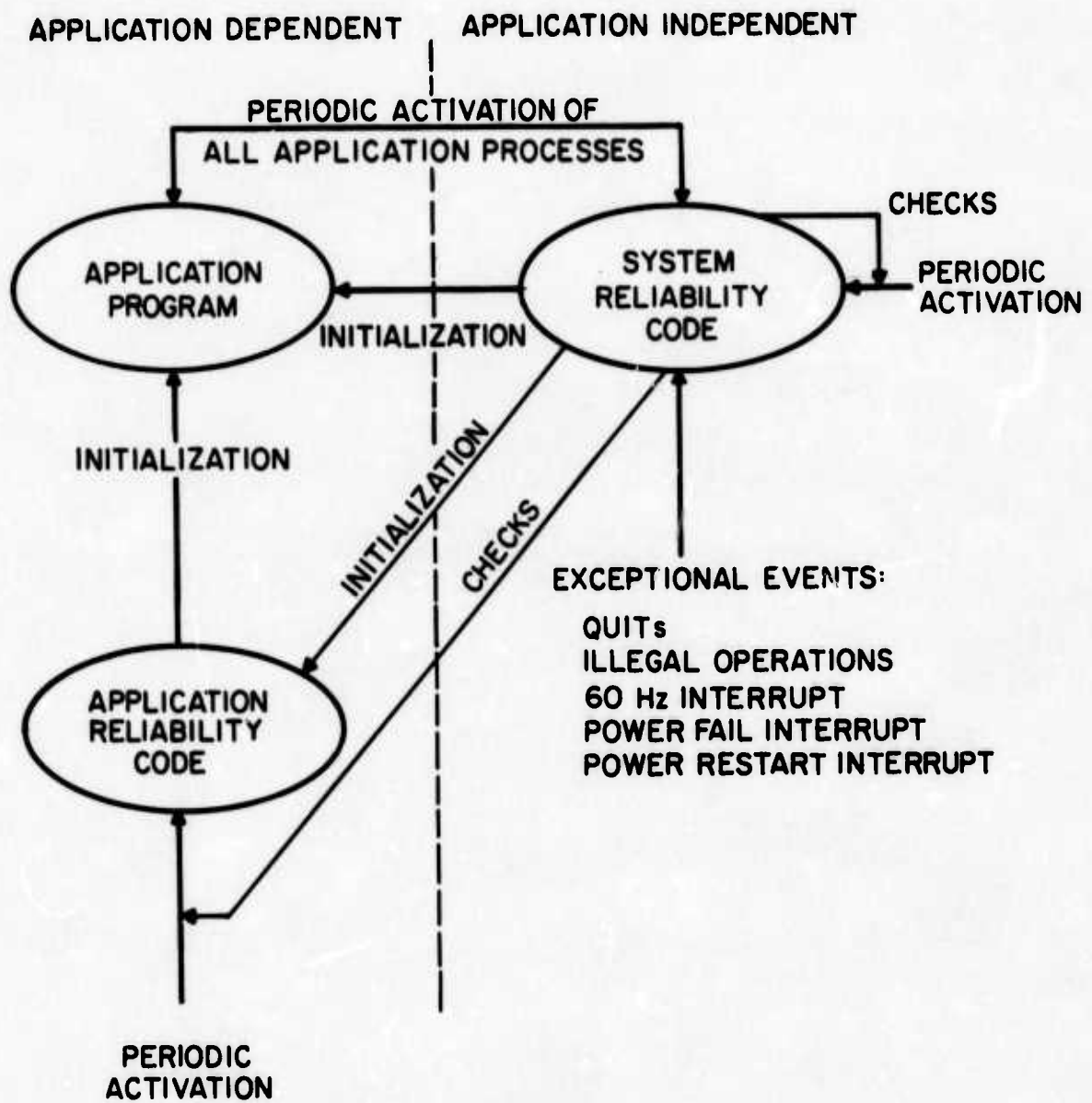
Figure 10 Reliability Software
