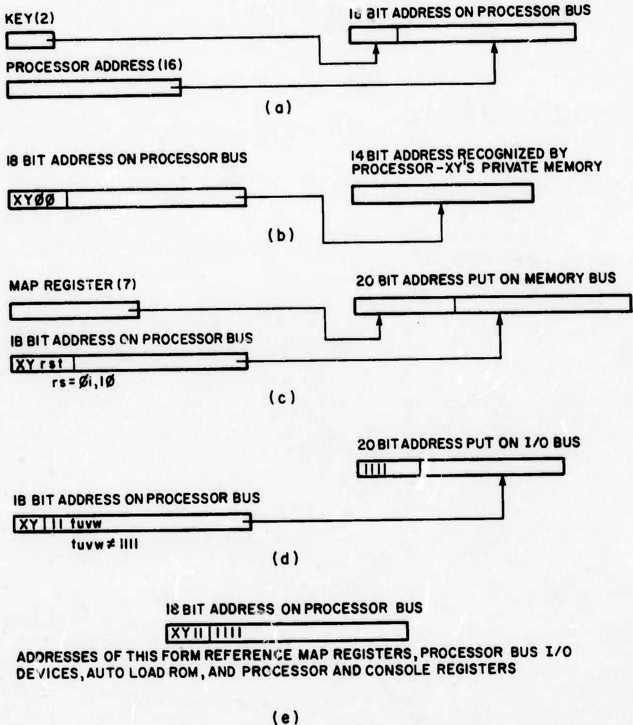
Figure 3 Address Mappings
