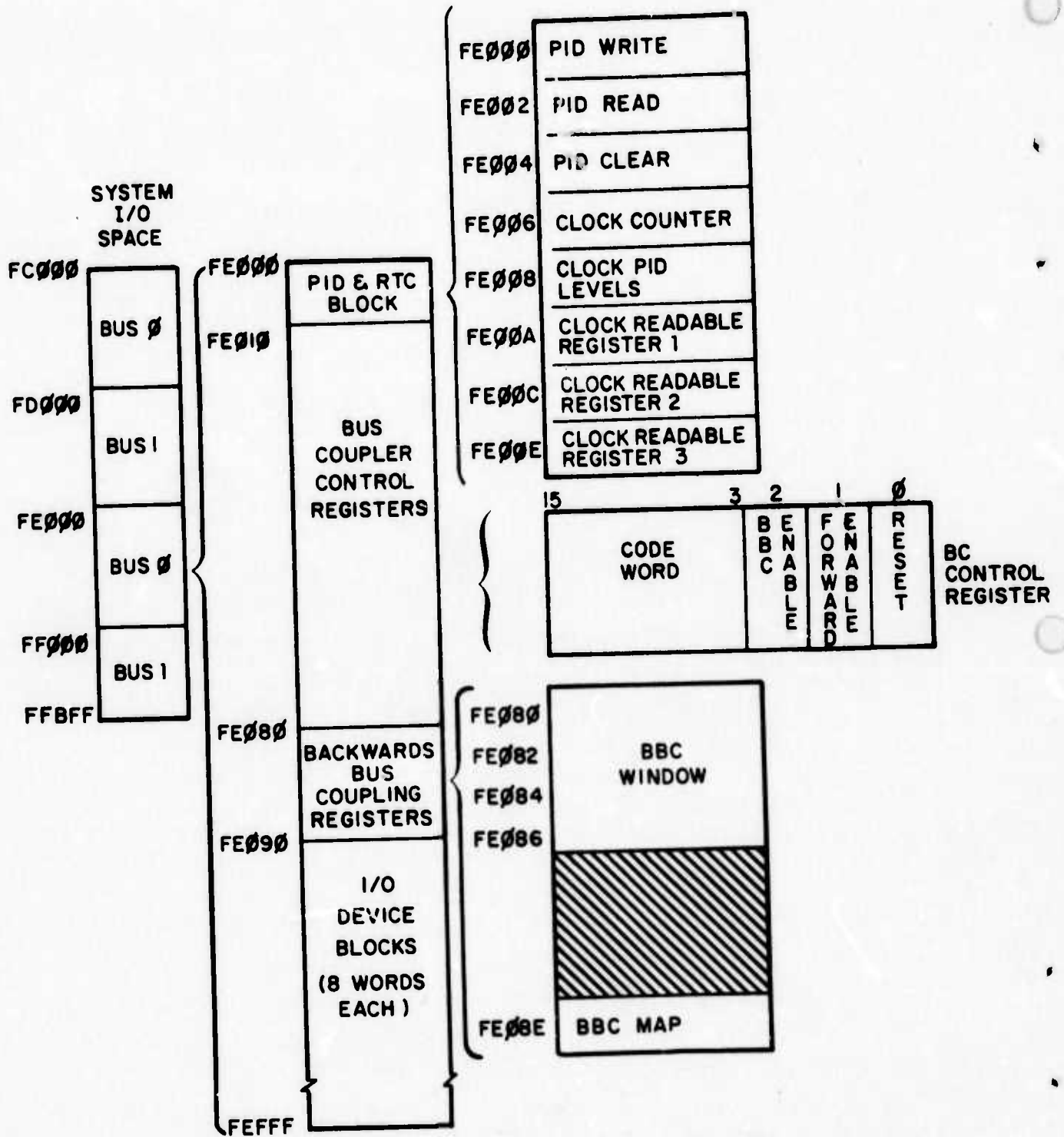
Figure 5 System I/O Space
