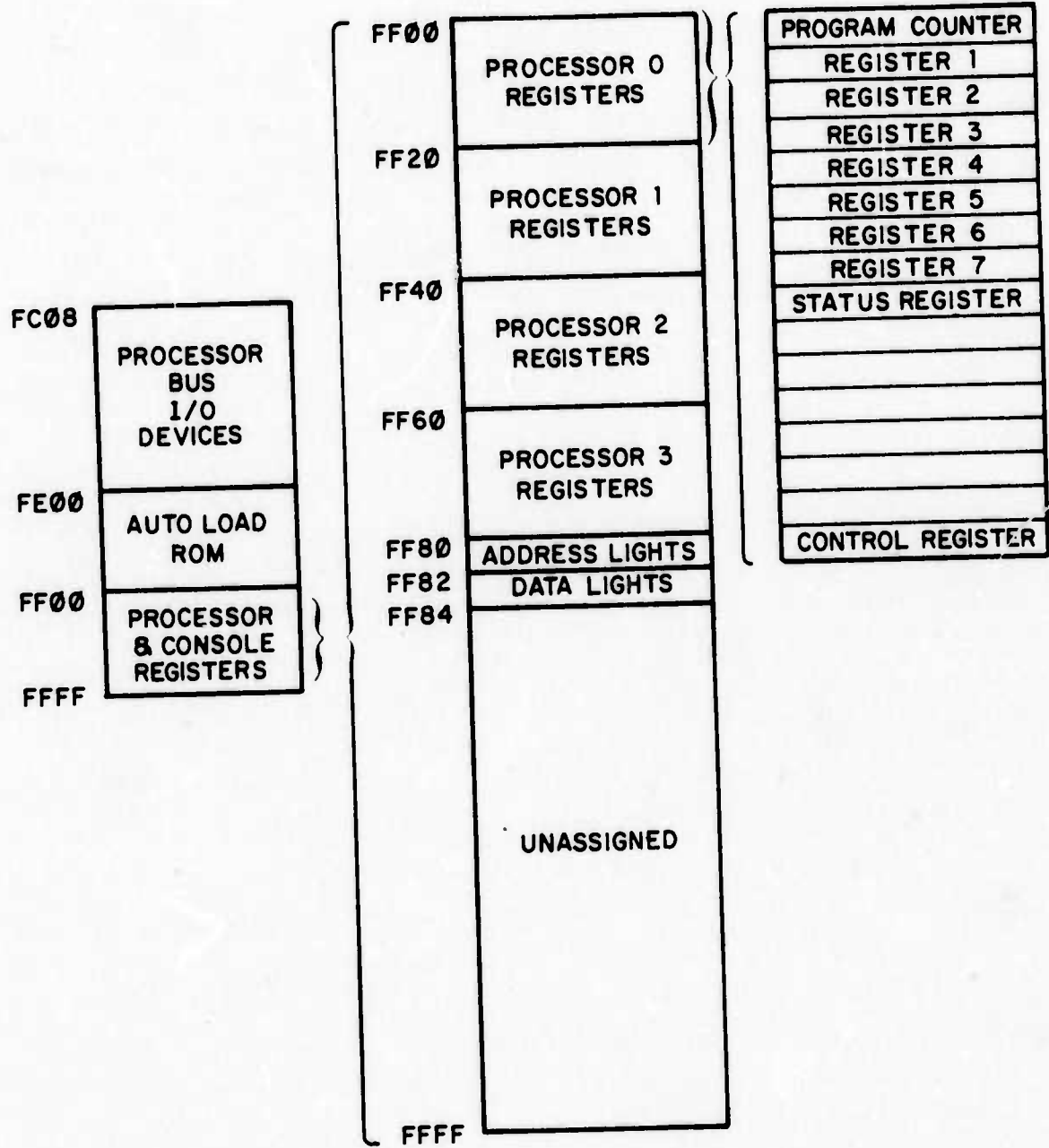
Figure 4 Processor Bus Shared Address Space
