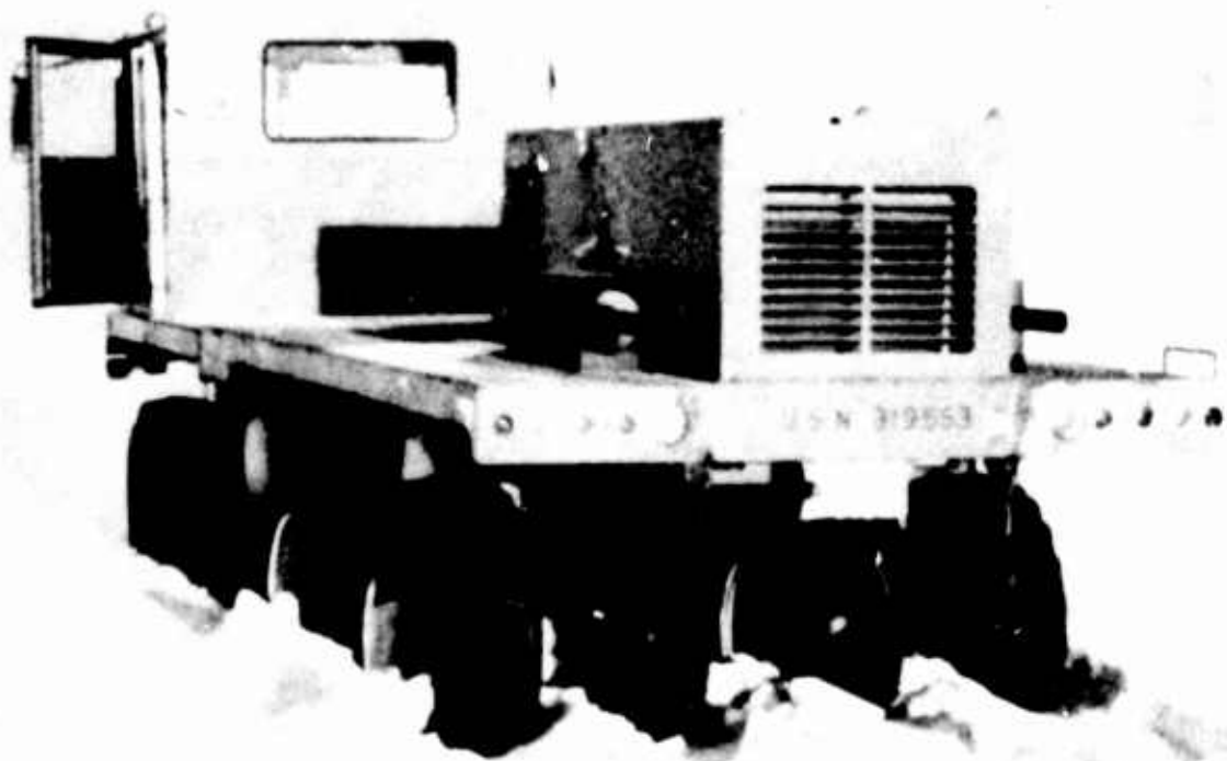
Figure 14. Testing LGPV-16 in 1974 over undisturbed snow on the Ross Ice Shelf, McMurdo, Antarctica
