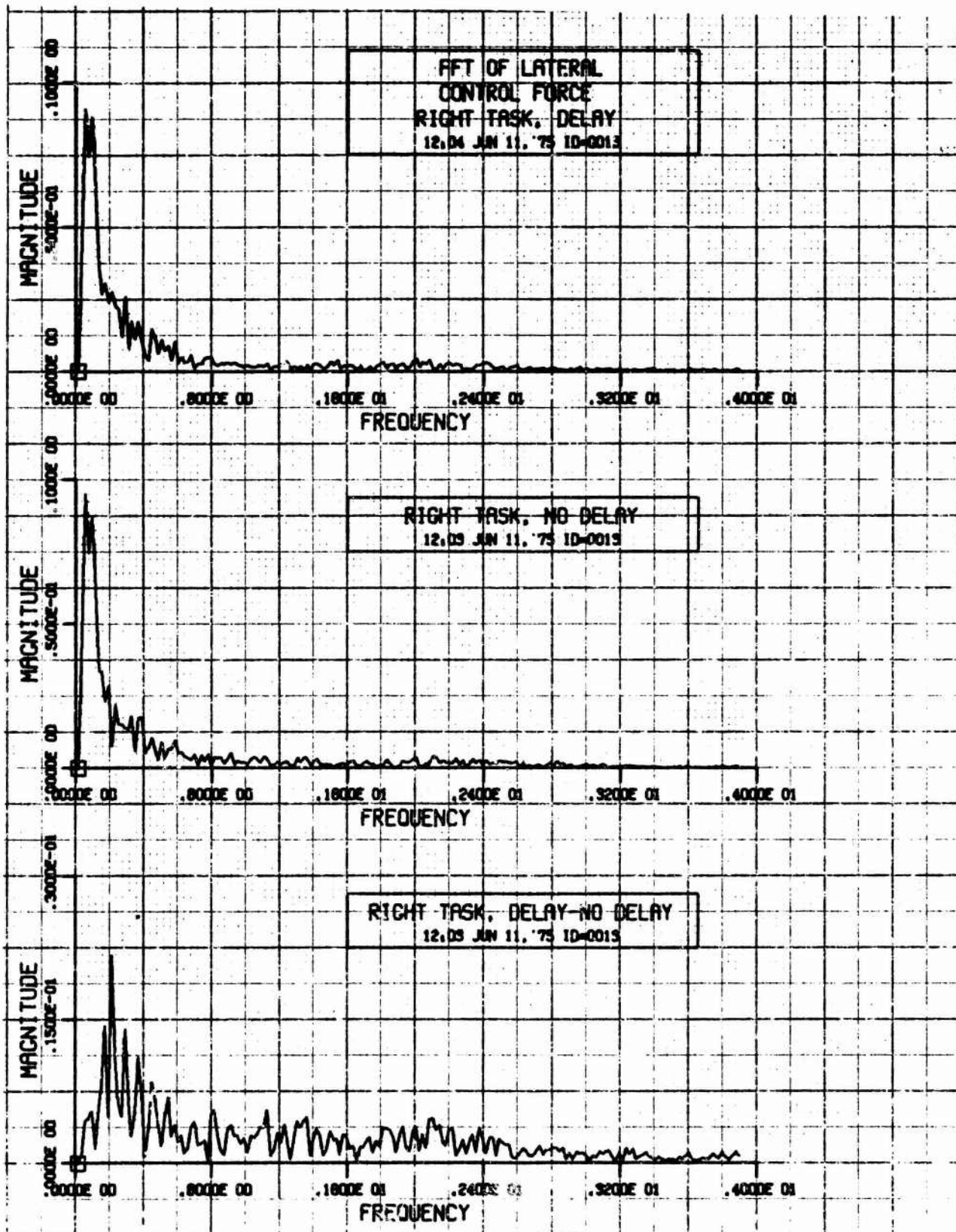
Figure 18. Fast Fourier Transforms of Control Inputs by Task (Continued)
