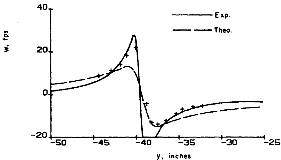
Figure 44. Configuration 3; comparison of measured and computed horizontal and vertical velocities ( x = 100 in., z = 69.1 in.)
