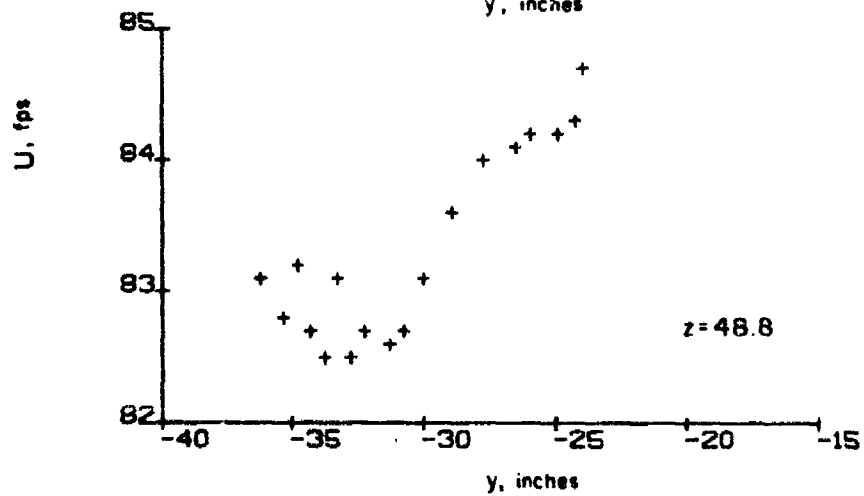
Figure B-4d. Configuration 4; measured axial velocities ( x = 50 in.)
