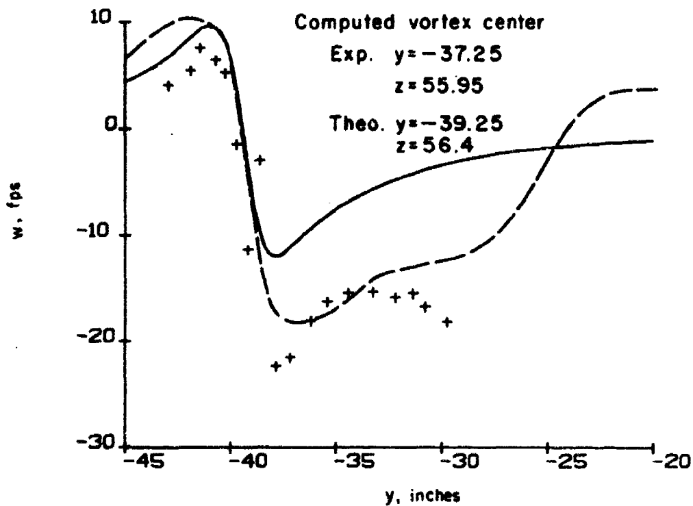
Figure B-3a. Configuration 4; tip vortex. Comparison of measured and computed horizontal and vertical velocities ( x = 50 in., z = 54.5 in.)
