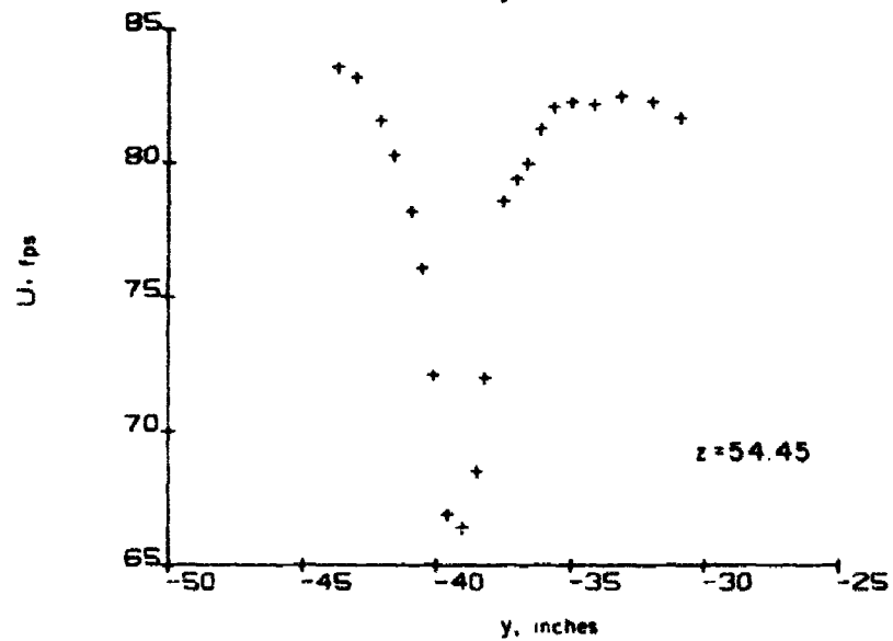
Figure B-3d. Configuration 4; measured axial velocities ( x = 50 in.)
