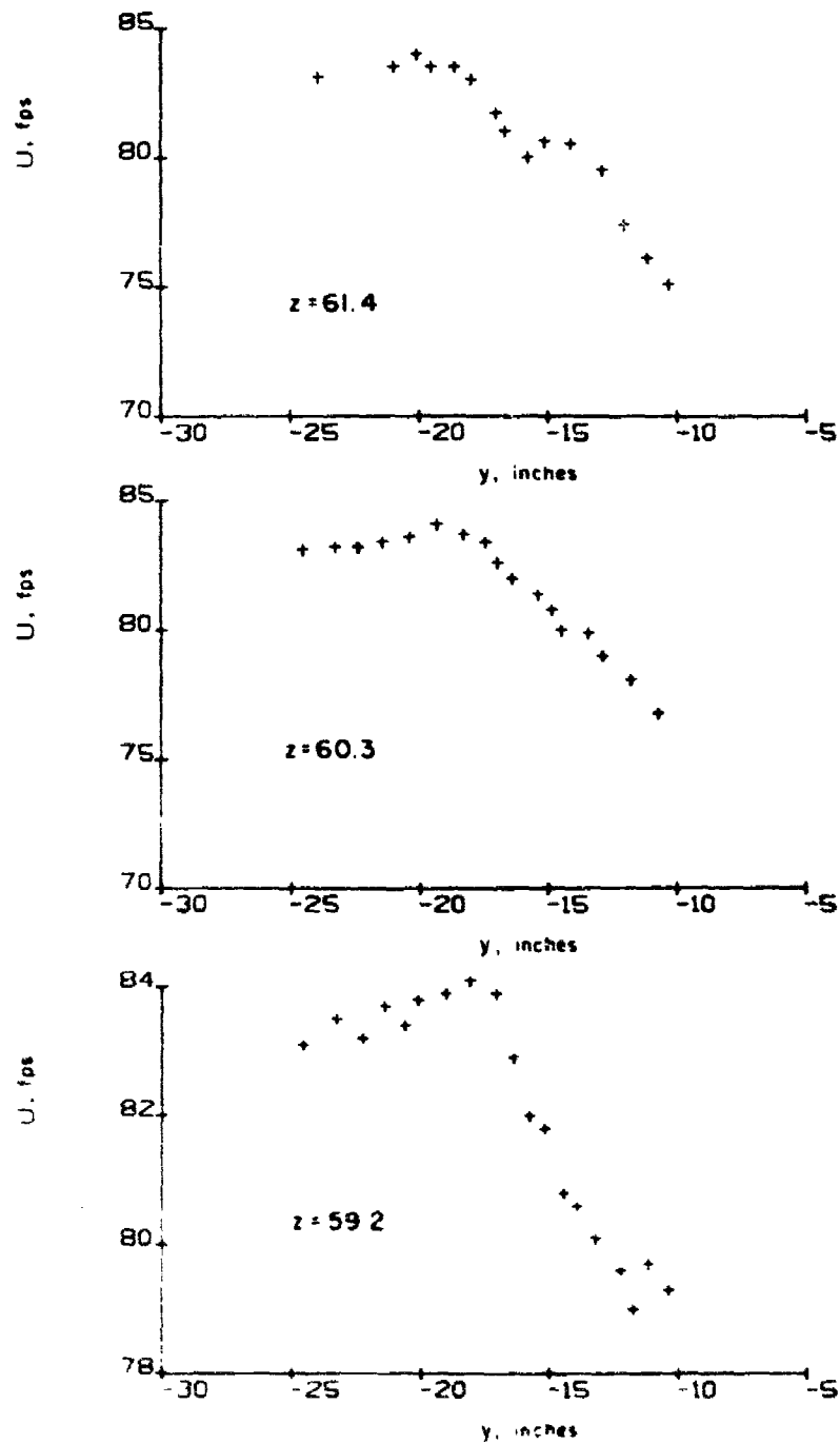
Figure 53. Configuration 2; measured axial velocities ( x = 50 in.)
