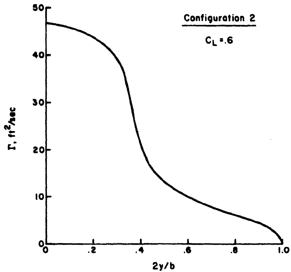
Figure 25. Lift distributions from lifting surface theory
