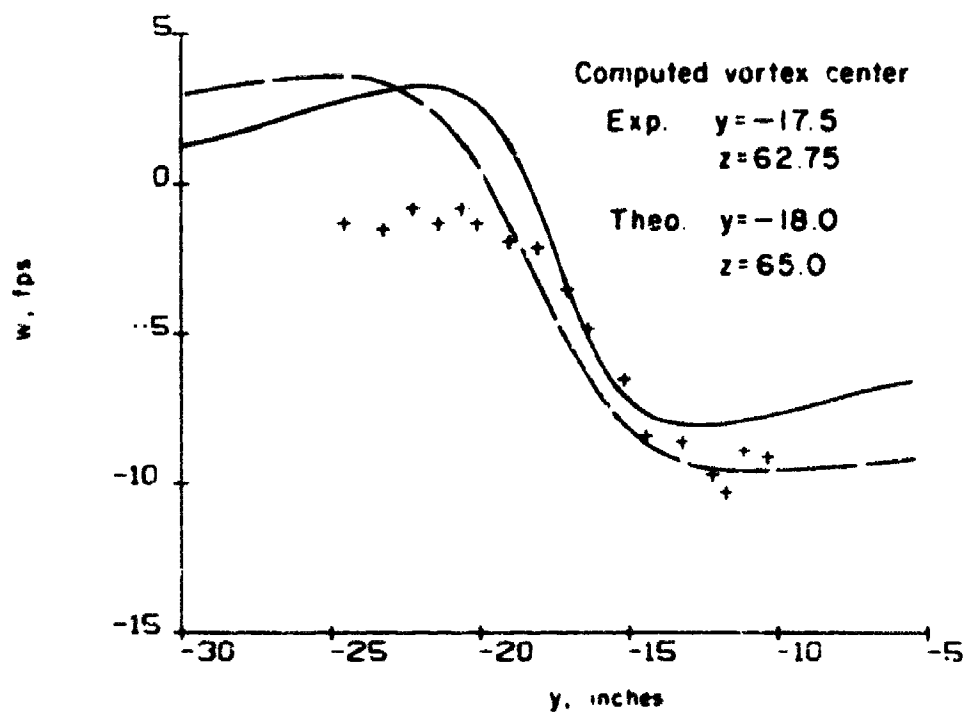
Figure 50. Configuration 2; flap vortex. Comparison of measured and computed horizontal and vertical velocities ( x = 50 in., z = 59.2 in.)
