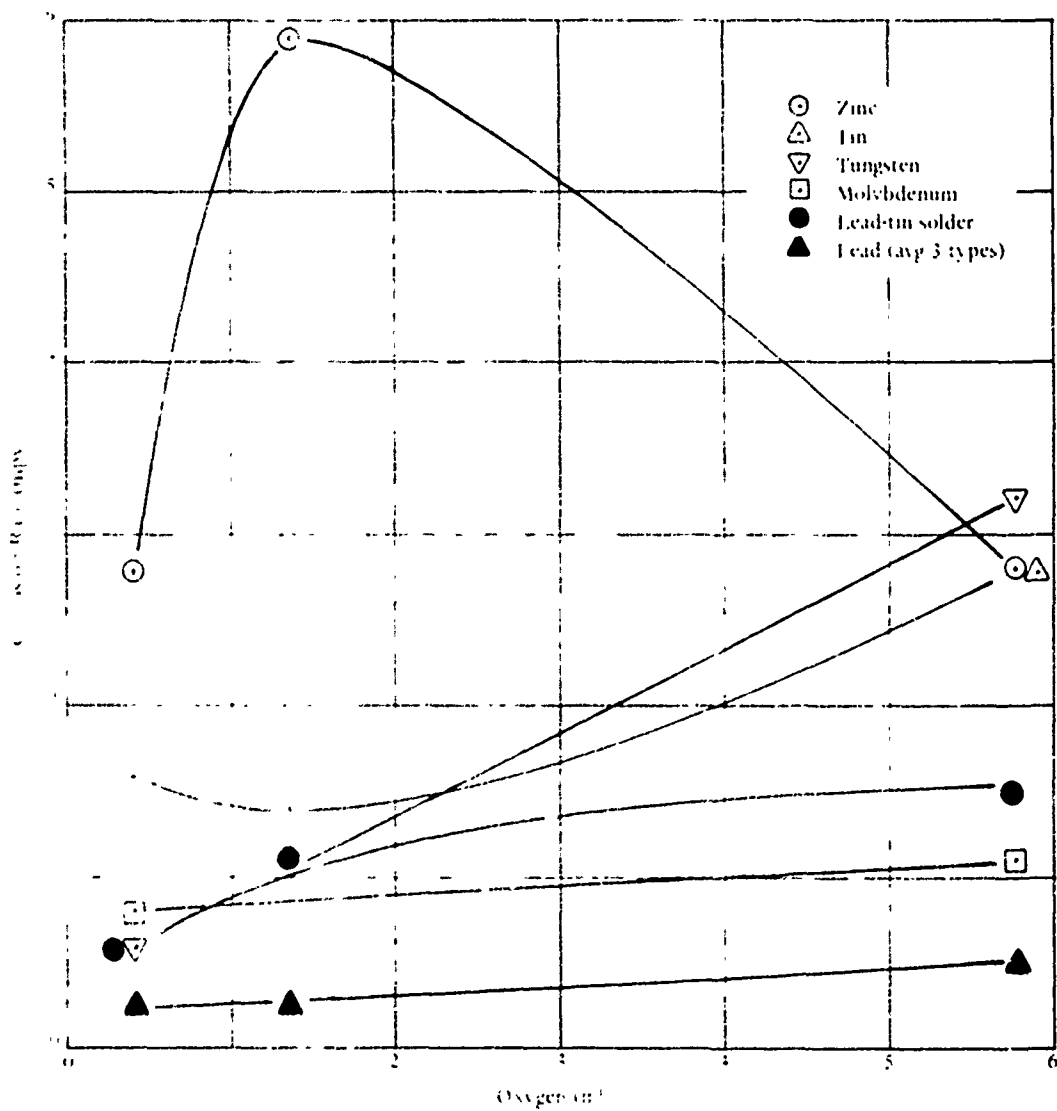
Figure 2. The concentration of oxygen in seawater on the corrosion of miscellaneous alloys after 1 year of exposure.
