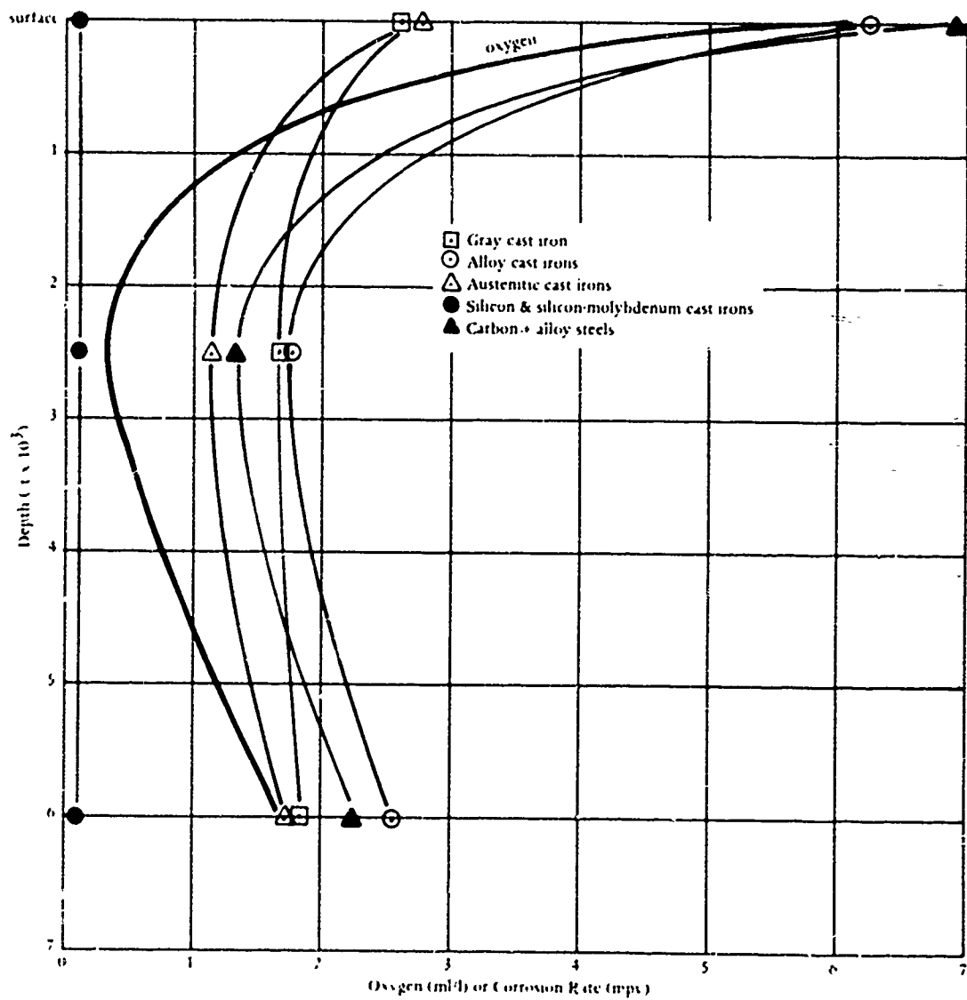
Figure 5. Effect of depth on the corrosion of steels and cast irons after 1 year of exposure in seawater.
