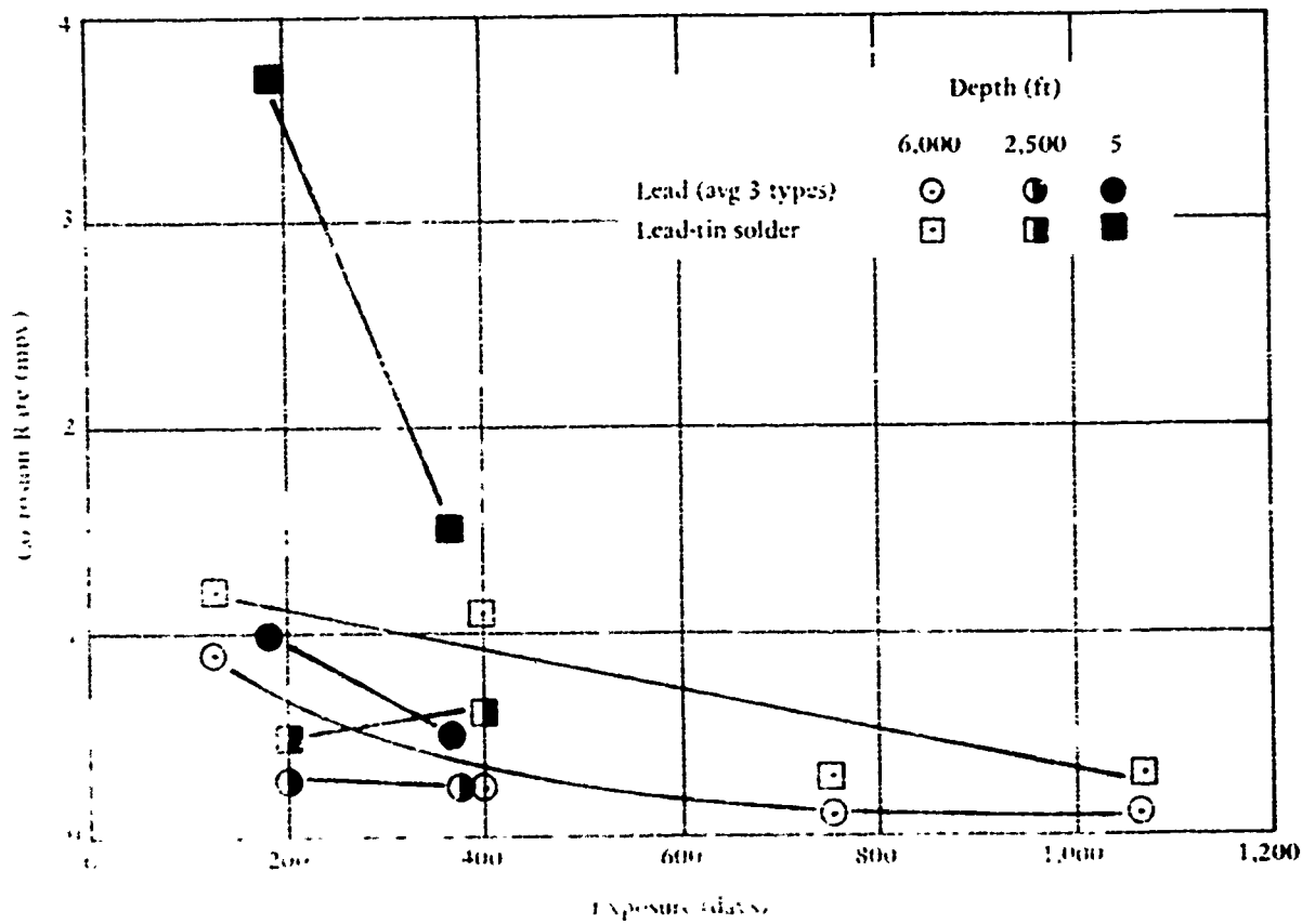
Fig. 1. Effect of duration of exposure in seawater on the corrosion of lead and lead-tin solder at the surface and at depth.
