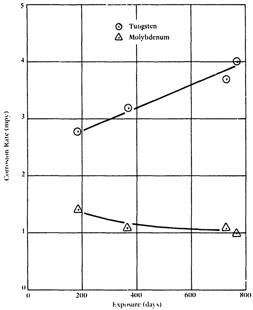
Figure 20. Effect of duration of exposure in surface seawater on the corrosion of molybdenum and tungsten.
