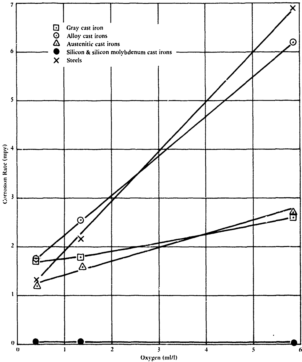
Figure 6. Effect of concentration of oxygen in seawater on the corrosion of steels and cast irons after 1 year of exposure.
