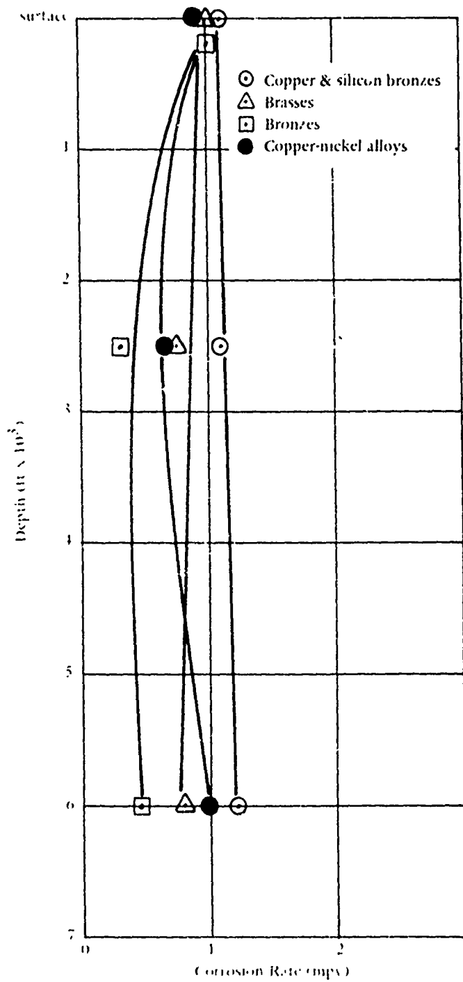
Figure 9 Effect of depth on the corrosion of copper alloys after 1 year of exposure in seawater.
