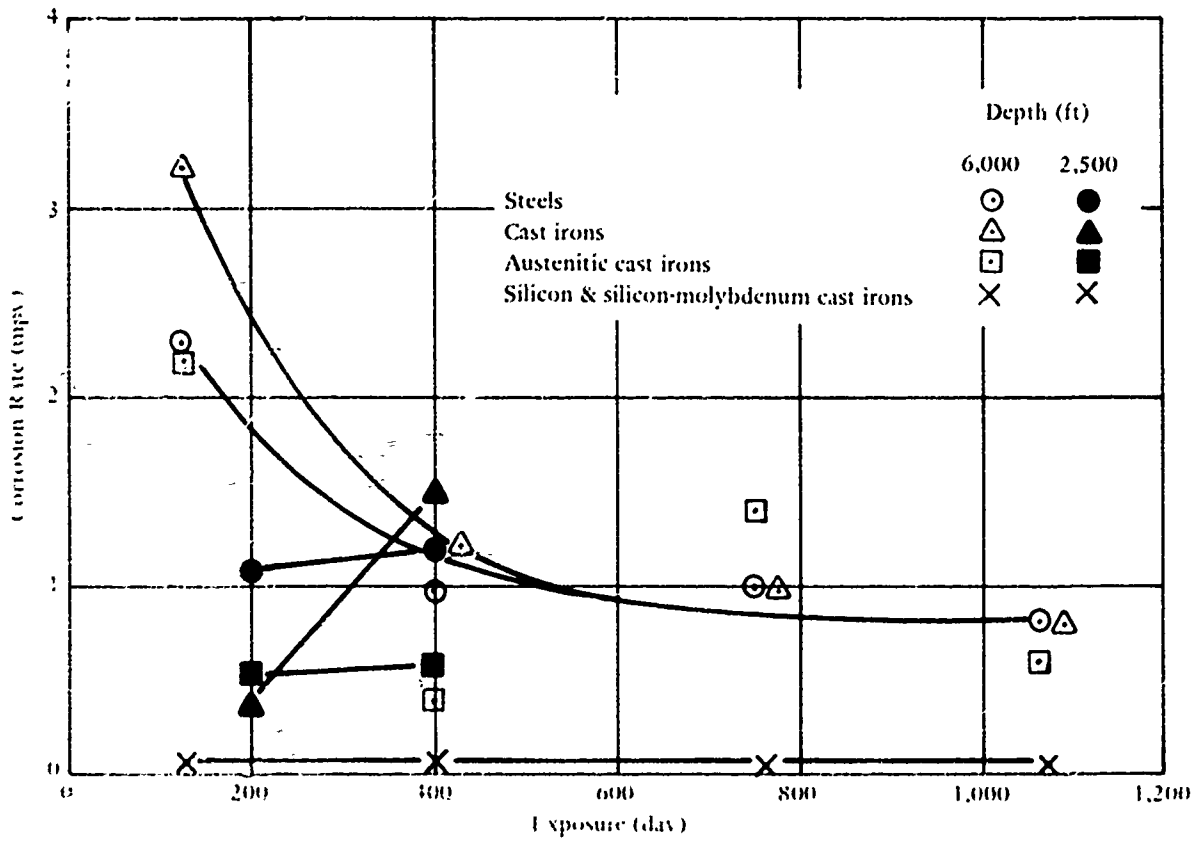
Figure 4. Effect of duration of exposure on corrosion of steels and cast irons in bottom sediments.
