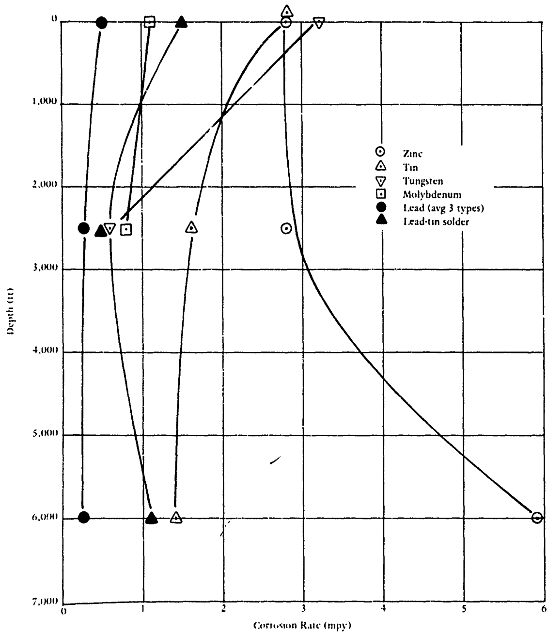
Figure 21. Effect of depth on the corrosion of miscellaneous alloys after 1 year of exposure.
