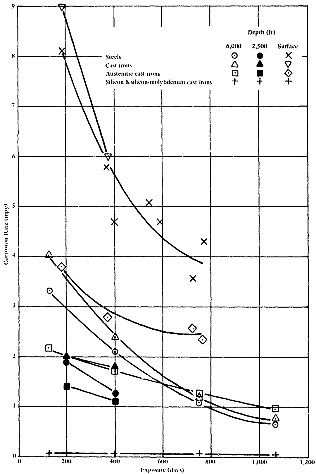
Figure 3. Effect of duration of exposure on corrosion of steels and cast irons.
