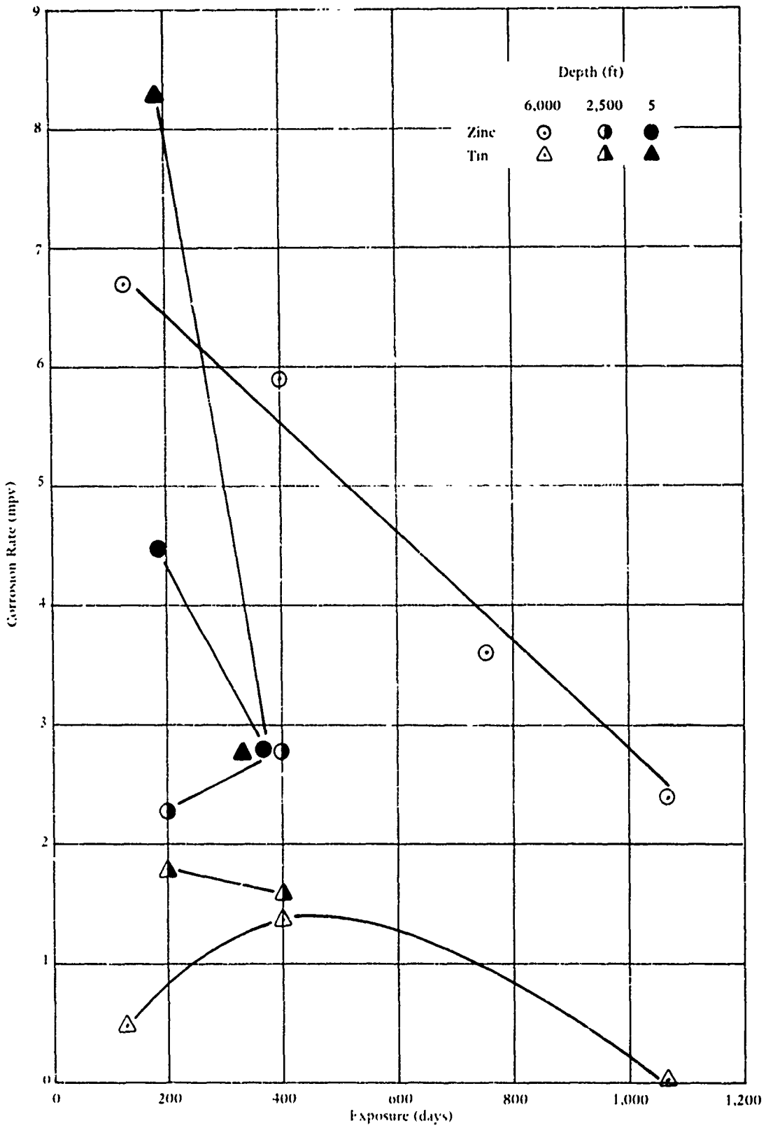
Figure 19. Effect of duration of exposure in seawater on the corrosion of tin and zinc at the surface and at depth.
