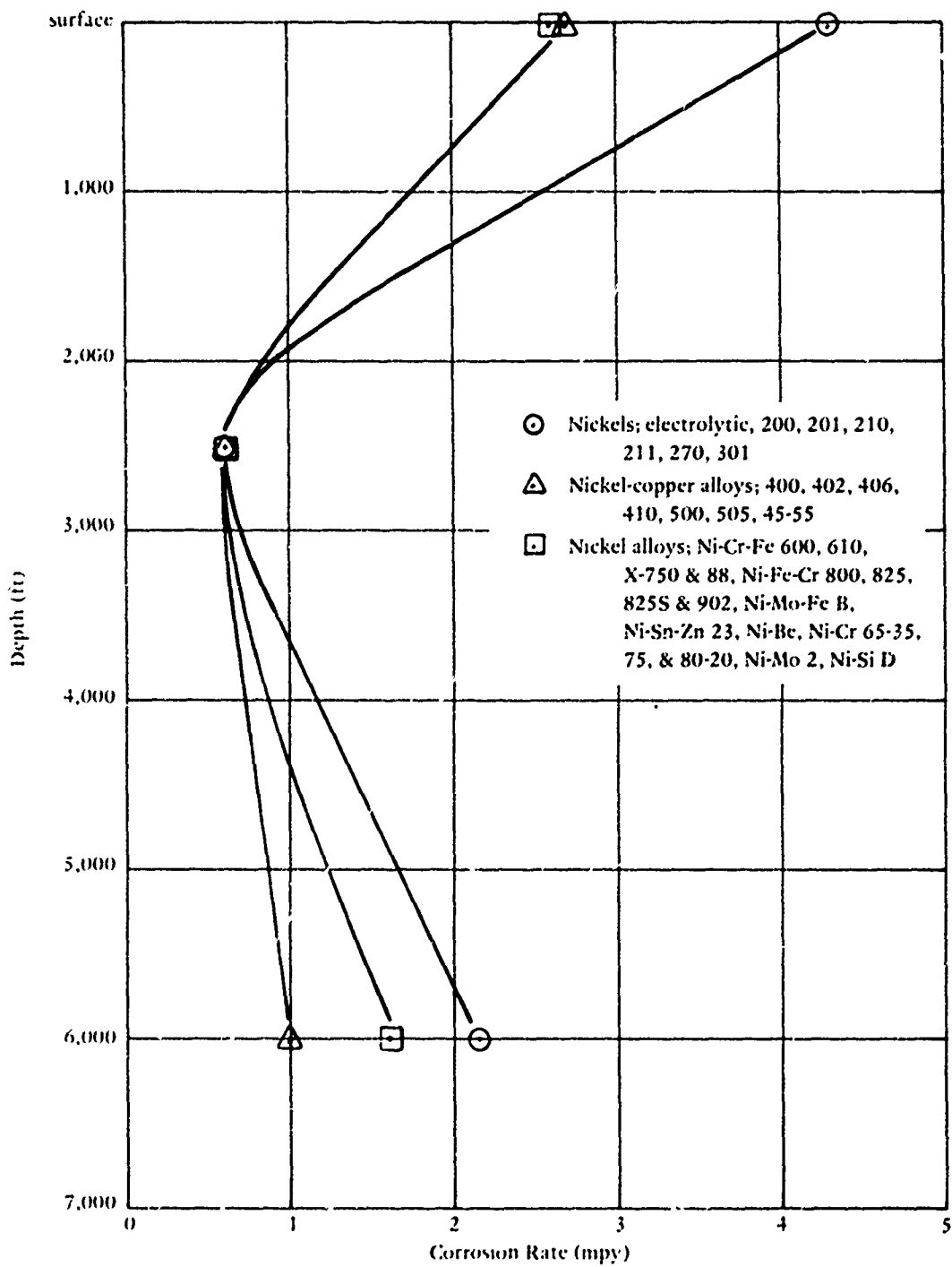
Figure 16 Effect of depth on the corrosion of nickel alloys after 1 year of exposure.
