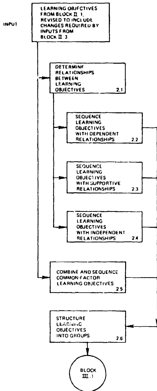
FIGURE II.9: Flowchart of Block II.4: DETERMINE SEQUENCE AND STRUCTURE
