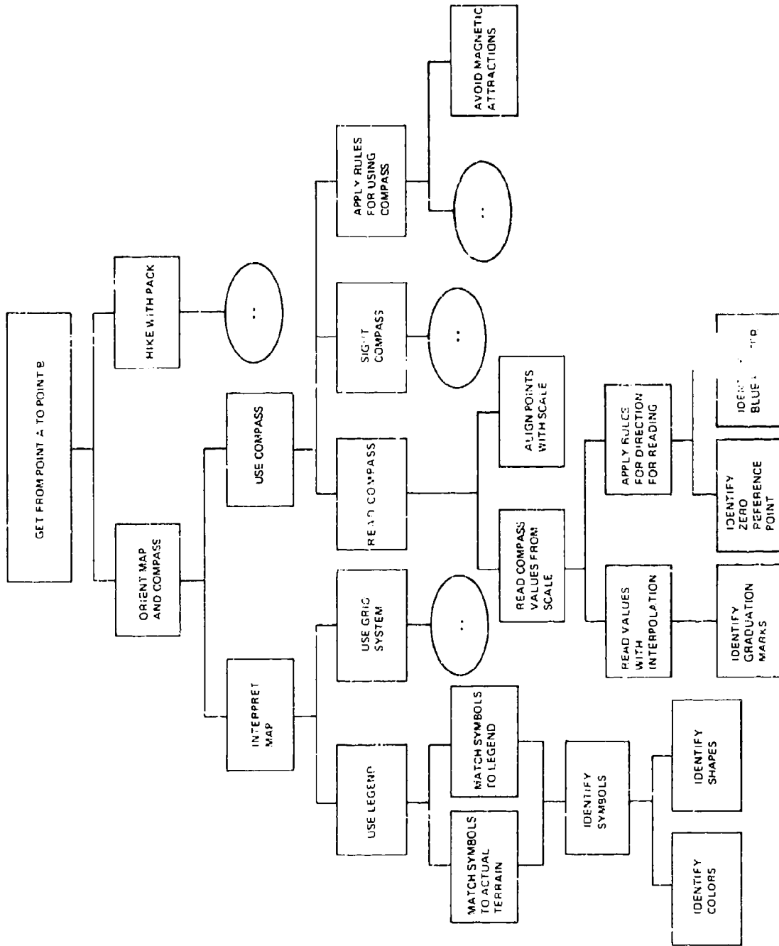
FIGURE II.10: Learning Analysis
