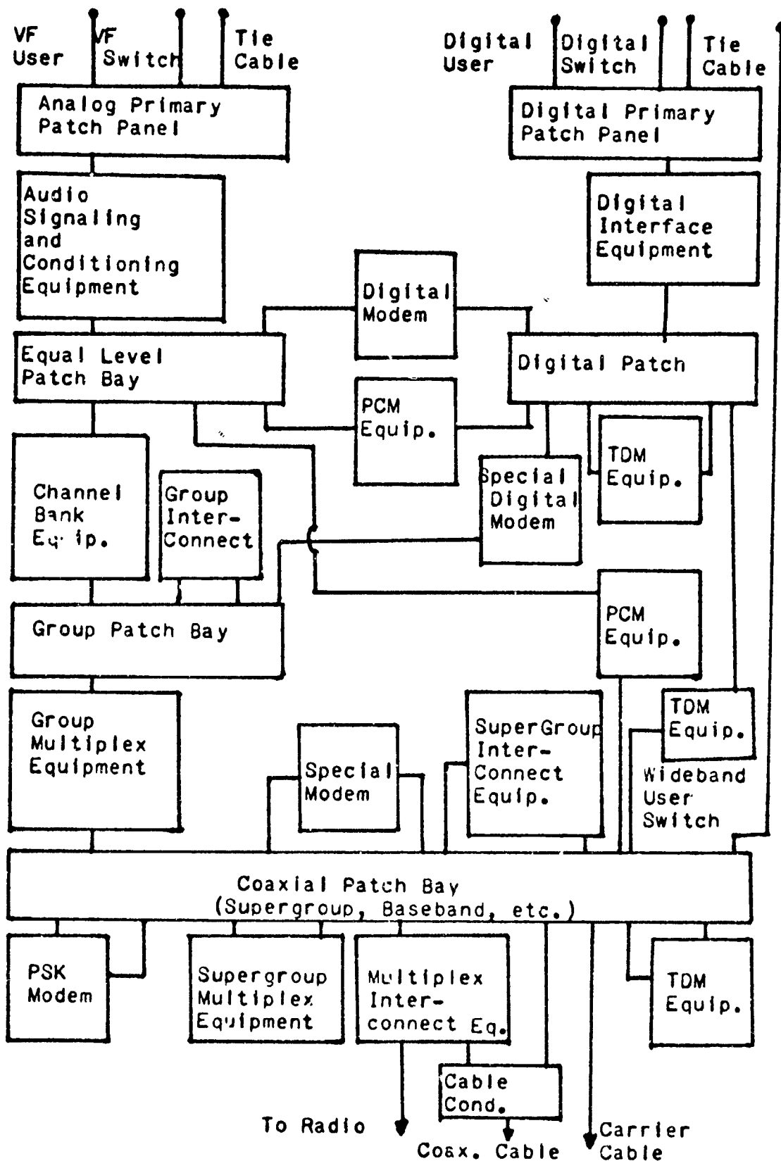
Figure 46- Technical Control Facility Block Diagram
