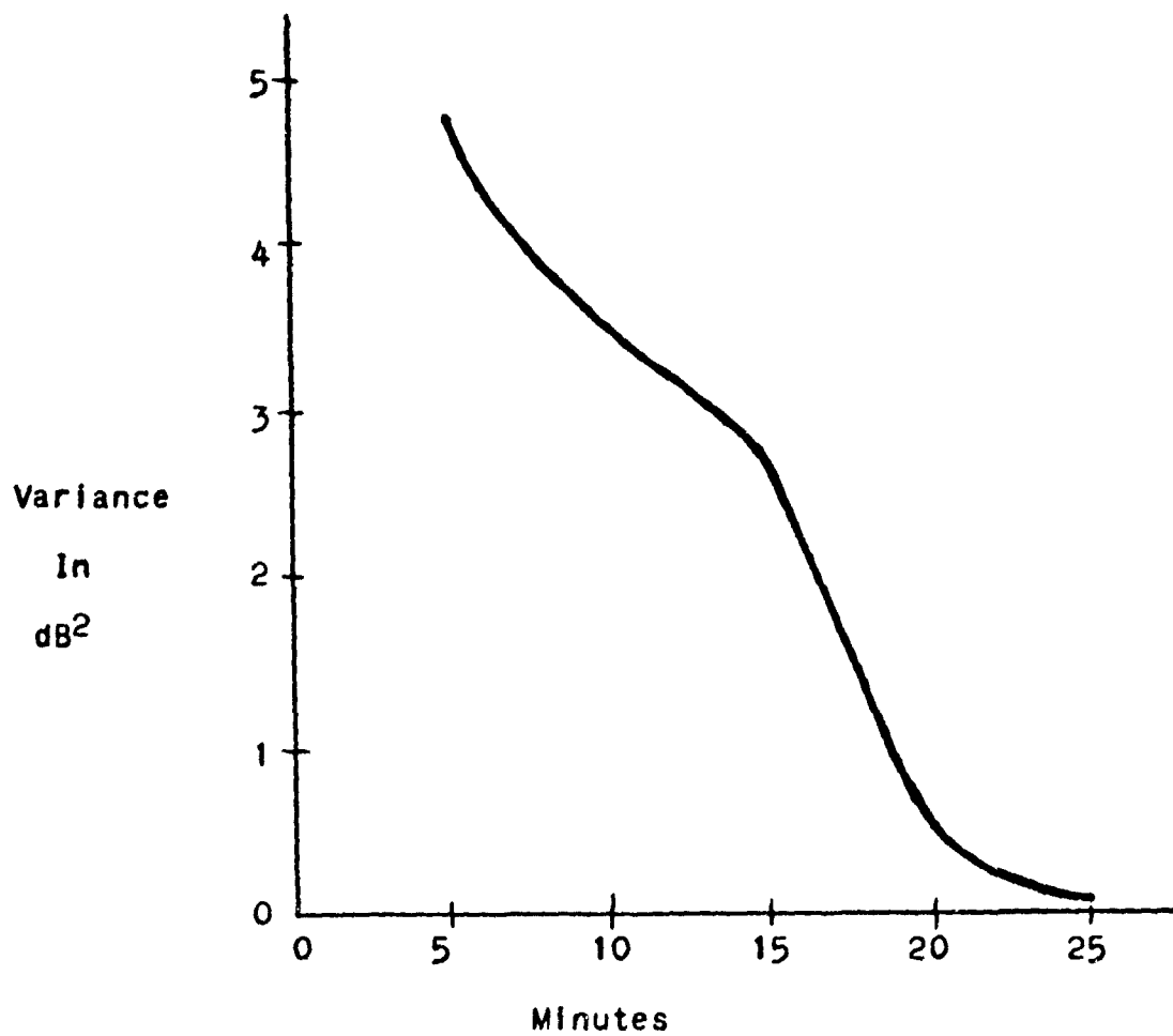
Figure 23- Variance of Estimated Impulse Noise Levels In Increments From 5 to 25 Minutes When Compared With A 30 Minute Estimate. (Radio Facility Example)
