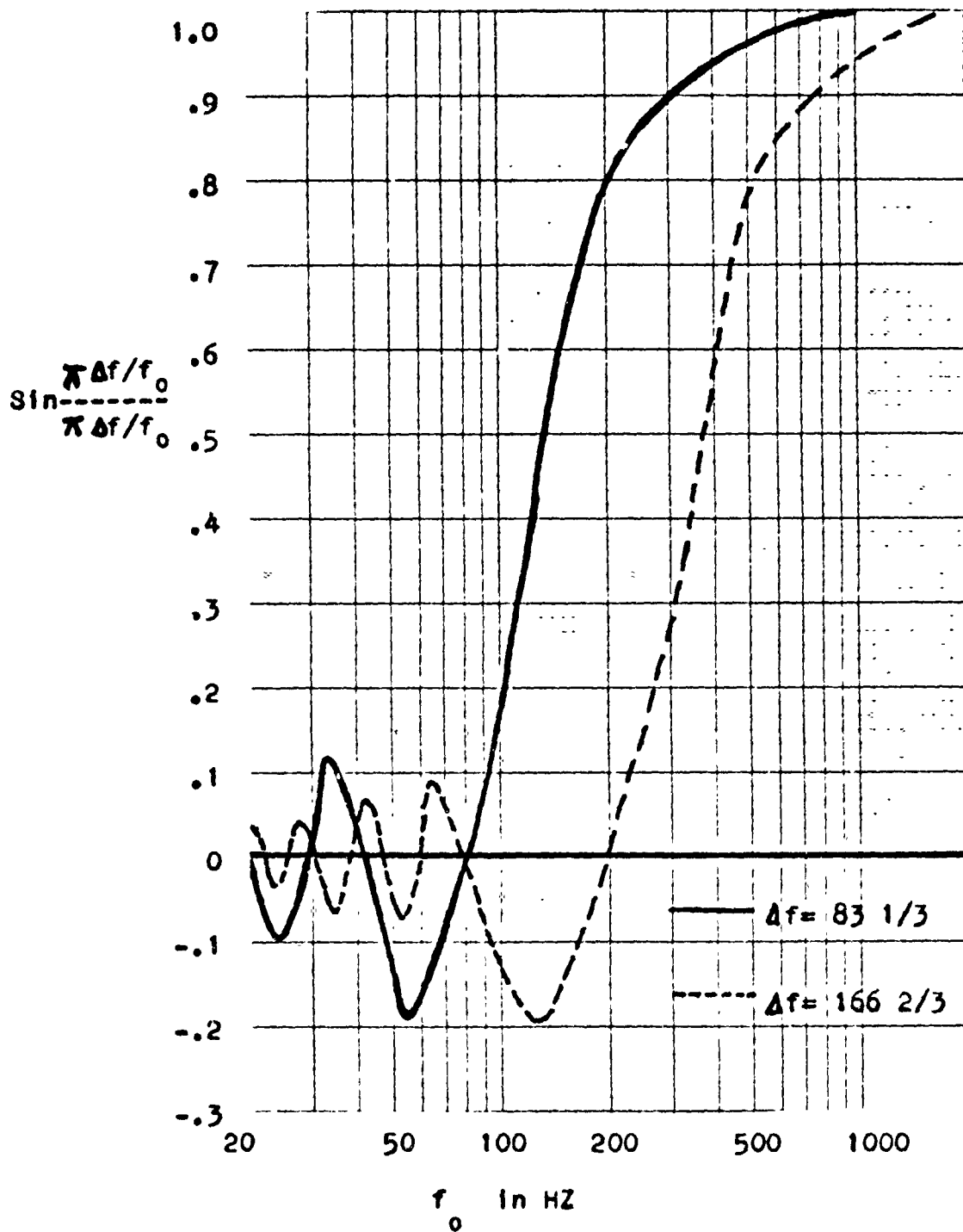
Figure 27- Response Of Two Envelope Delay Test Sets To Ripples In The Phase Characteristic Of A Transmission Line.
