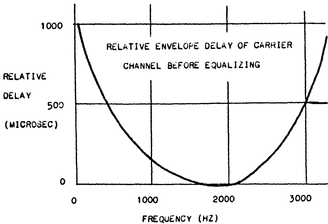
Figure 13- Typical Envelope Delay
