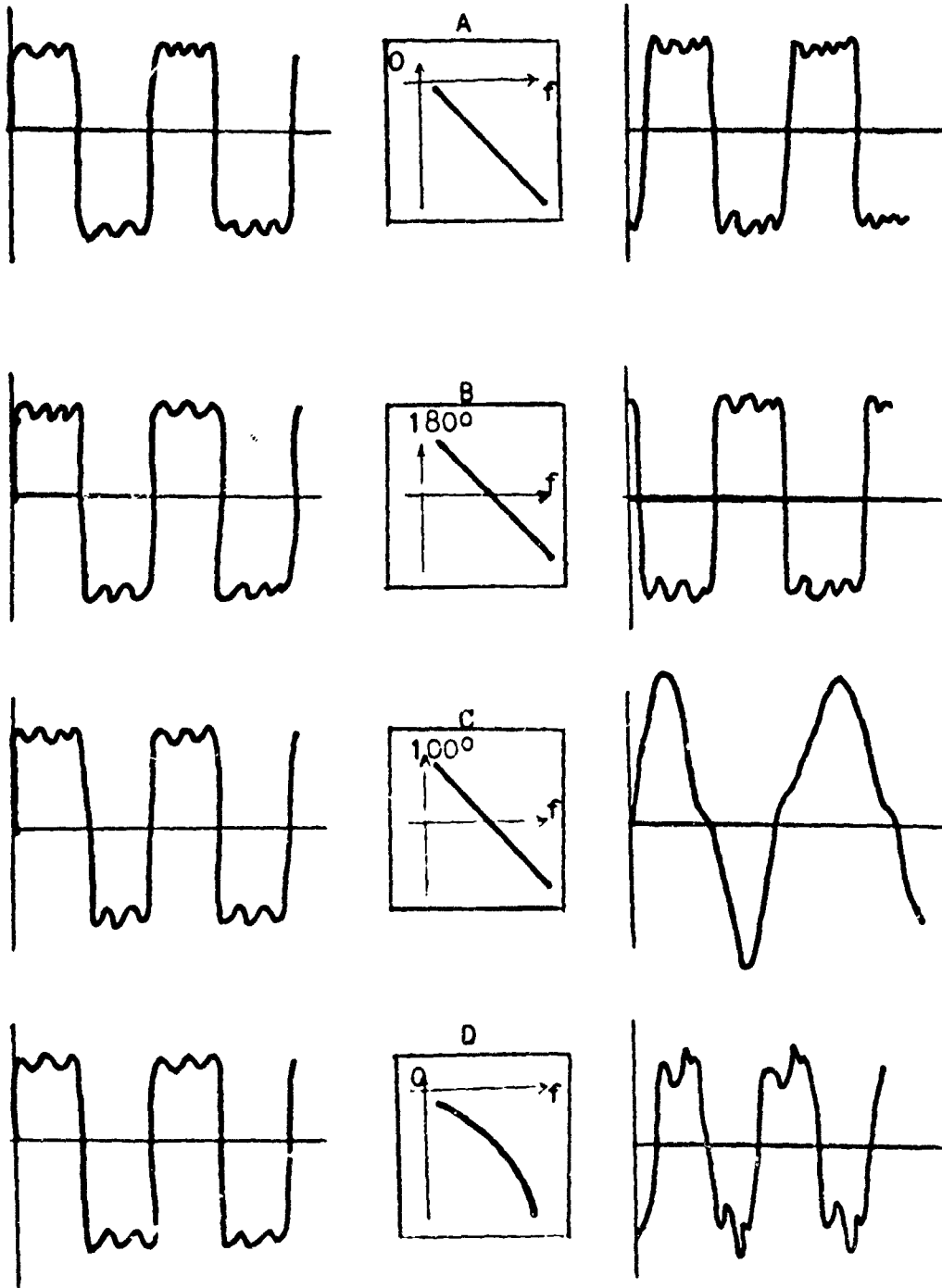
Figure 11- Effects of Various Phase-Frequency Relationships on a Complex Signal
