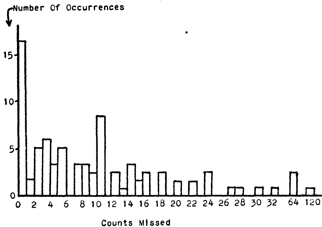
Figure 25- Number Of Impulses Missed In A 30 Minute Period By Electromechanical Counters. Threshold Always Adjusted To Produce Exactly 30 Counts In 30 Minutes On Counters.
