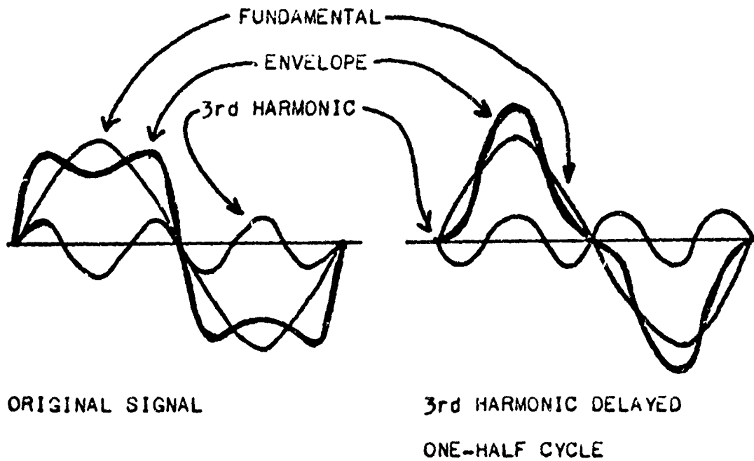
Figure 9- Effect of 3rd Harmonic Delay on Resultant Envelope of Signal
