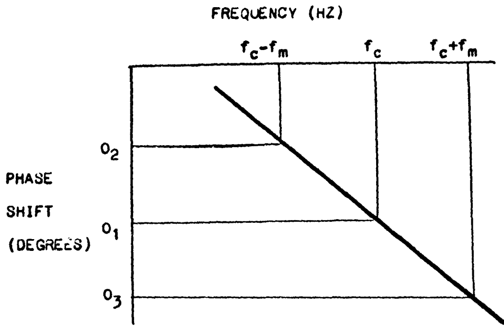
Figure 12- Phase Shift vs. Frequency Chart
