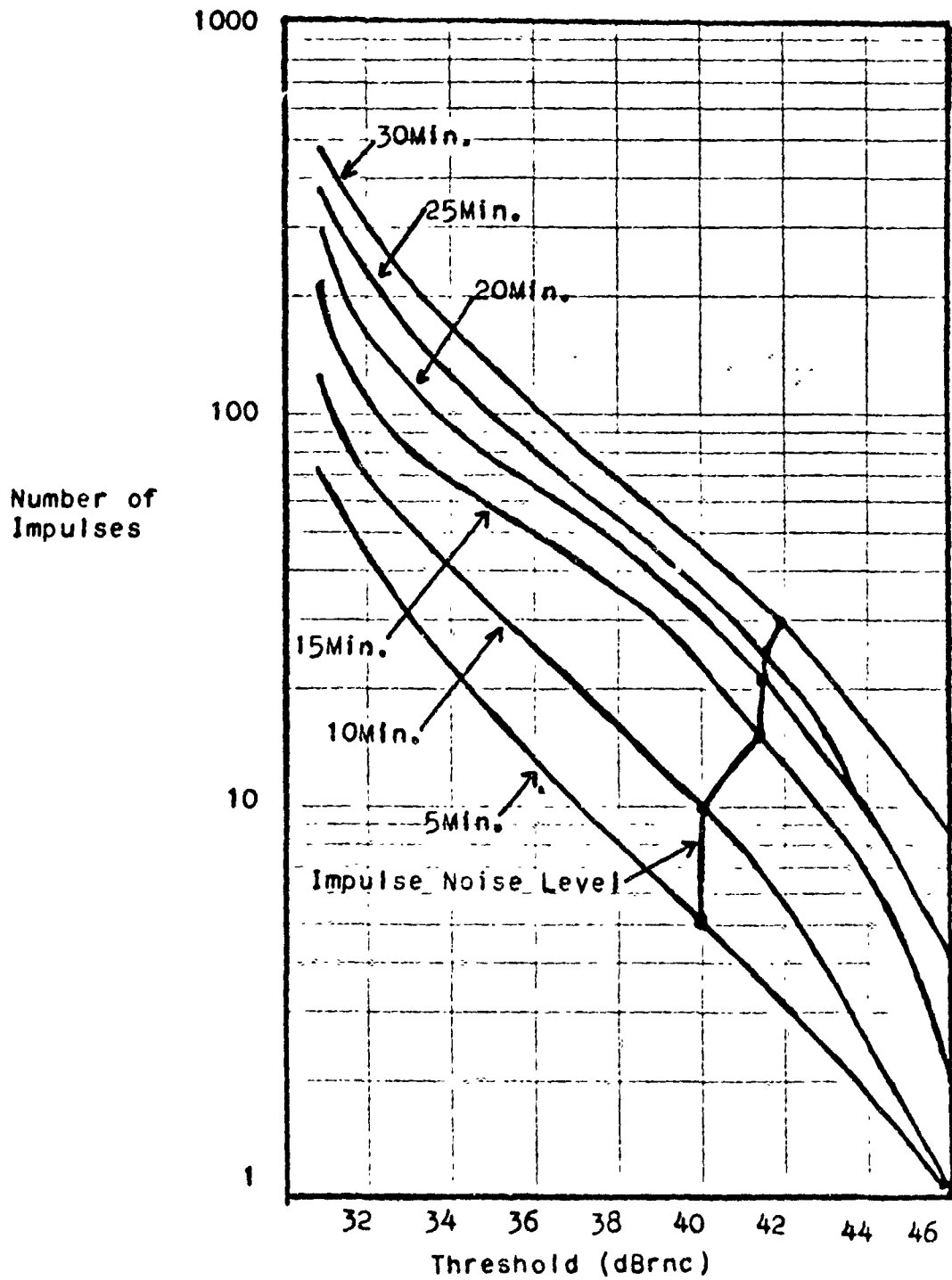
Figure 20- Cumulative Distributions of Impulse Noise Peaks In Successive Intervals From 5 to 30 Minutes.
