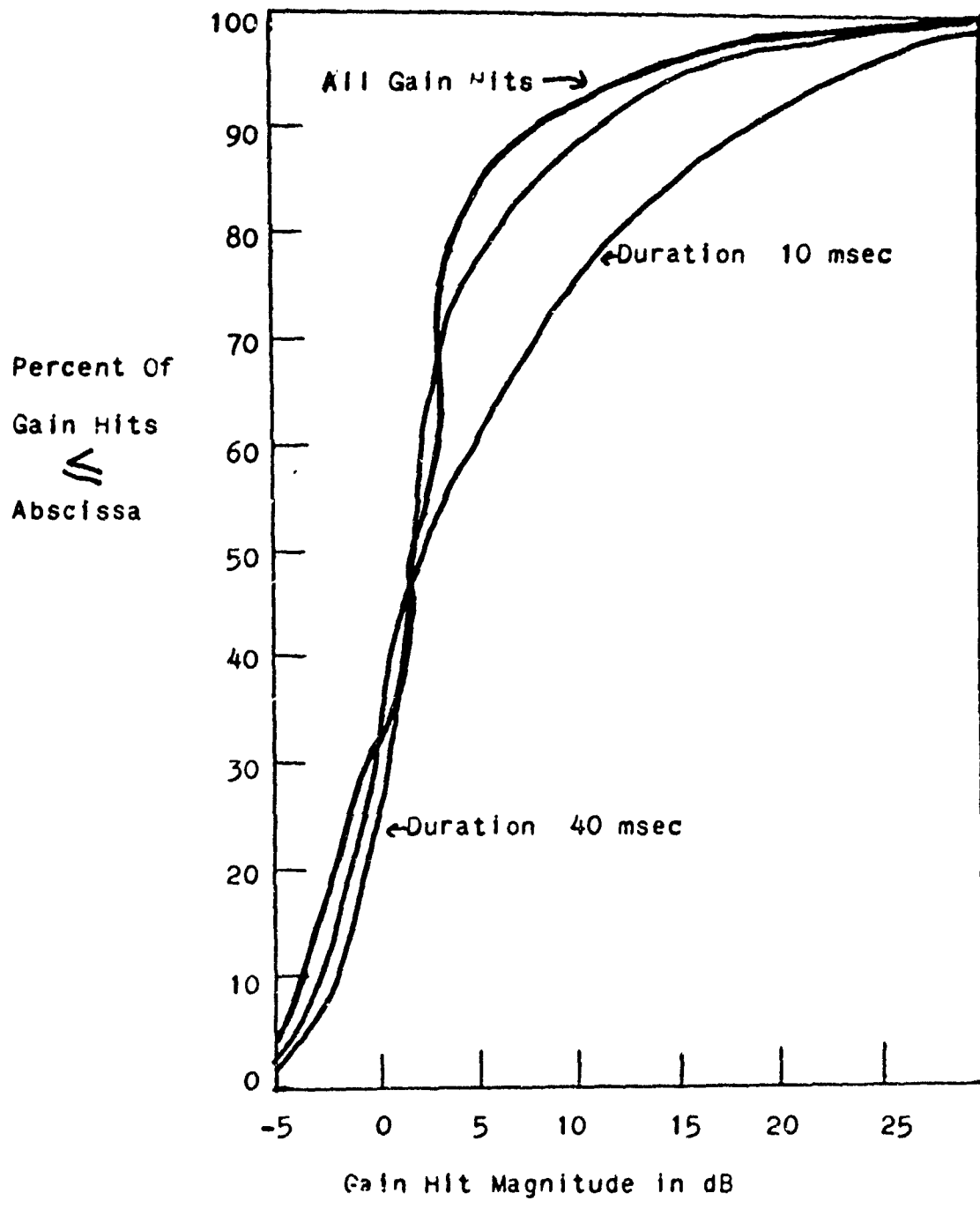
Figure 42- Distributions of Magnitudes Of Gain Hits.
