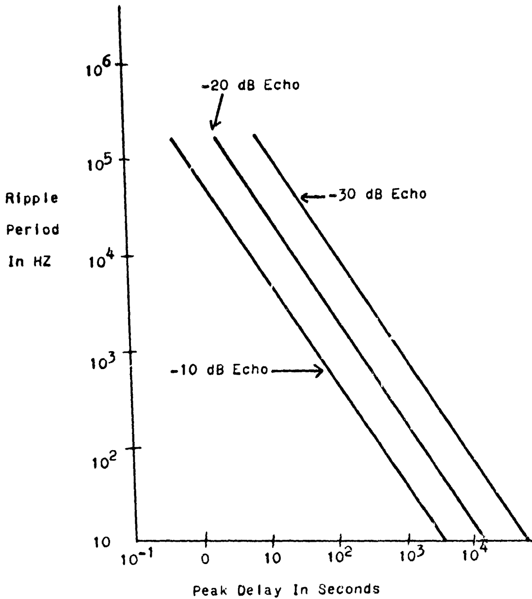
Figure 26- Peak Delay For Single Sinusoidal Ripple With Constant Echo Magnitude.
