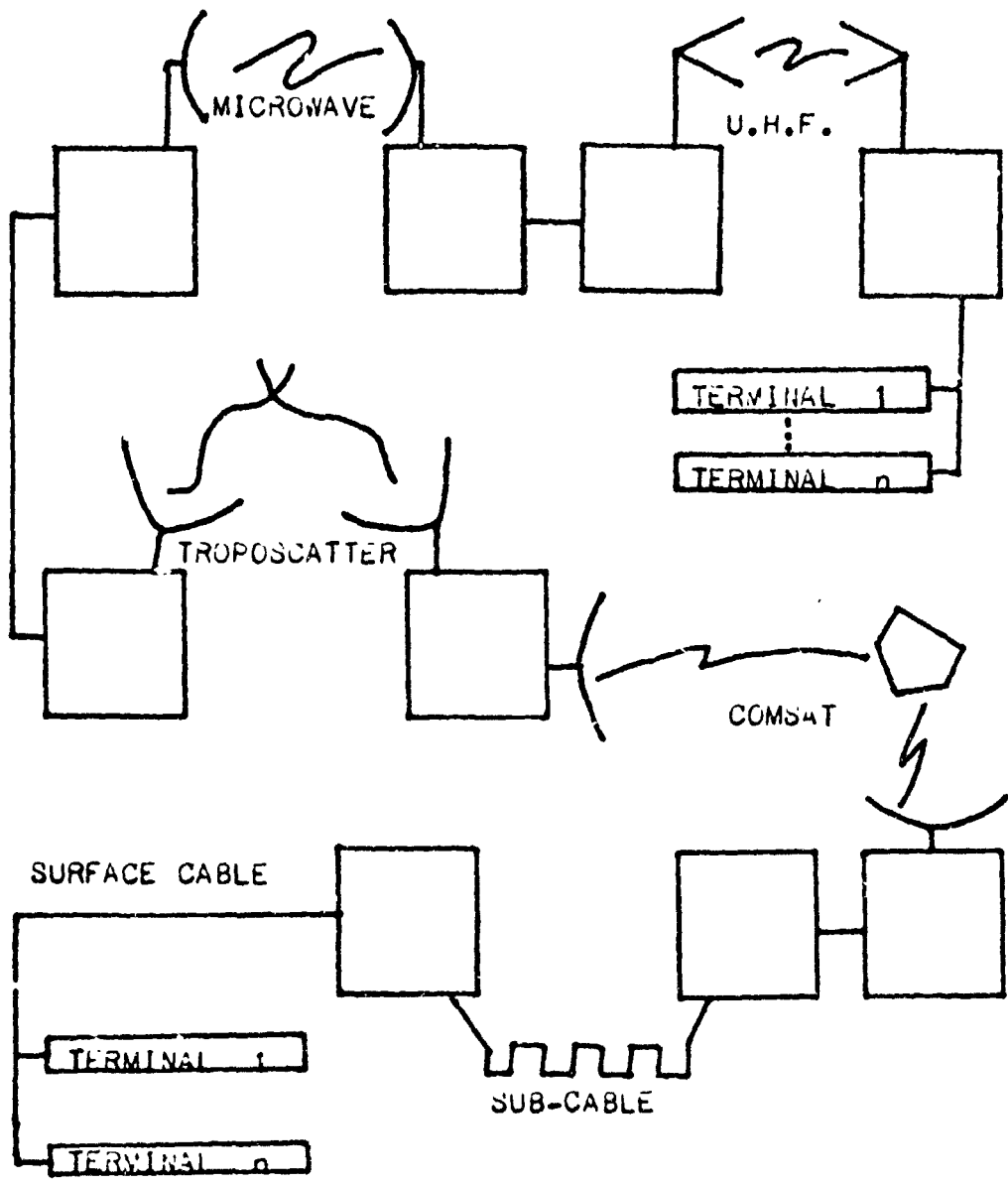
Figure 1- Typical Military Communications System ( Long-Haul, Wide-Band, Multi-Channel )
