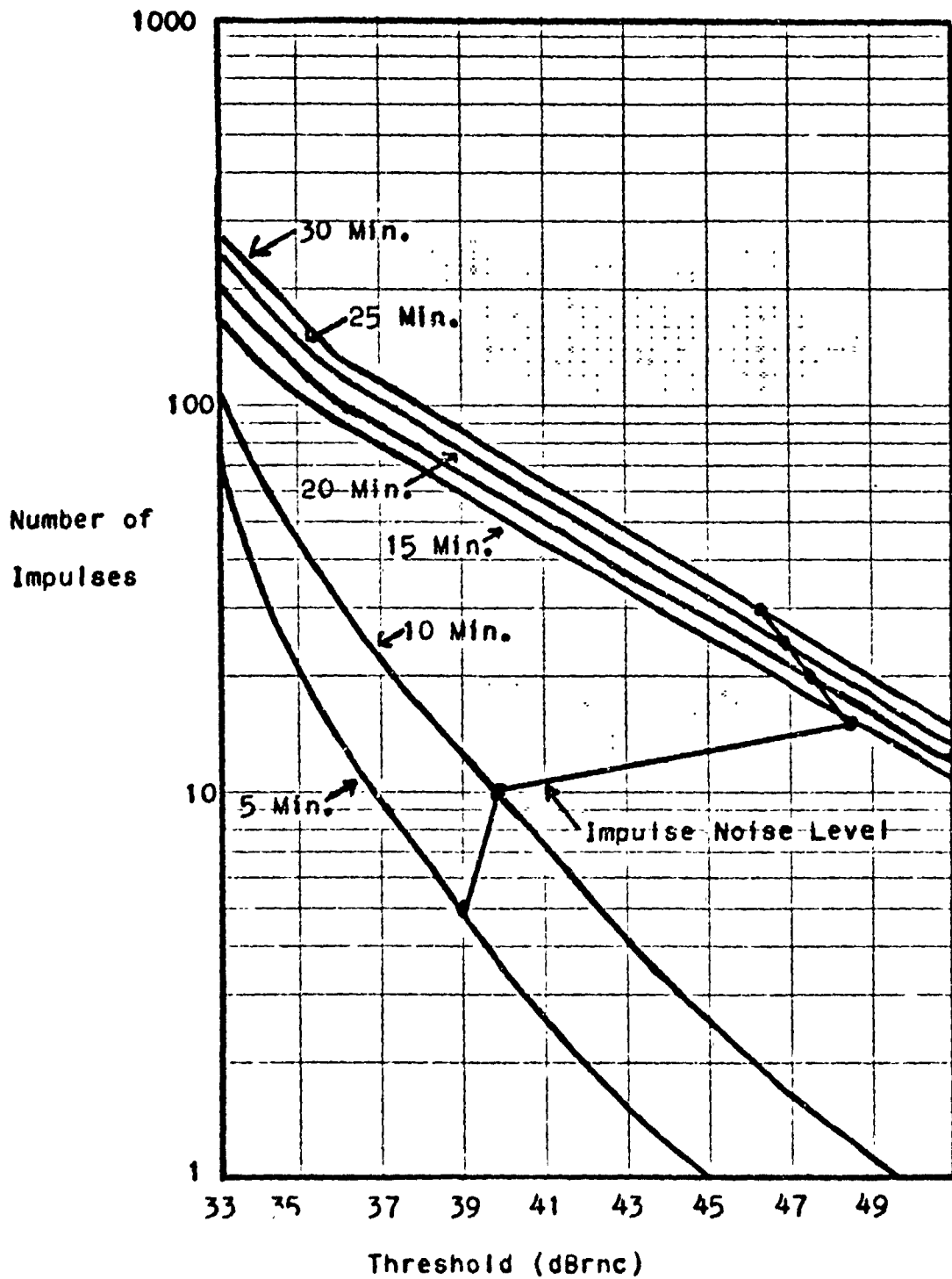
Figure 21- Cumulative Distributions of Impulse Noise Peaks In Successive Intervals From 5 to 30 Minutes.
