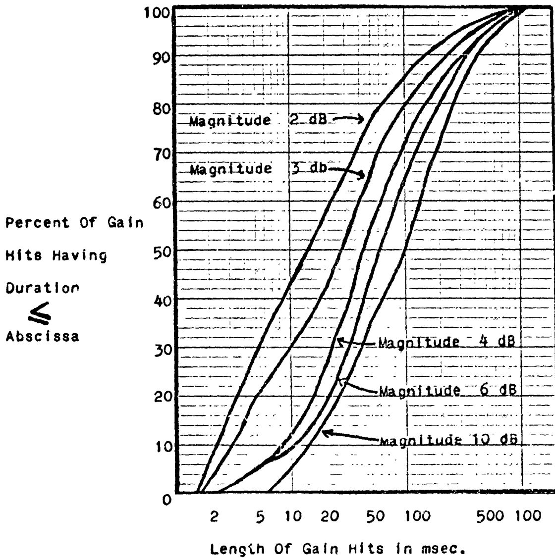
Figure 43- Distribution Of Length Of Gain Hits.
