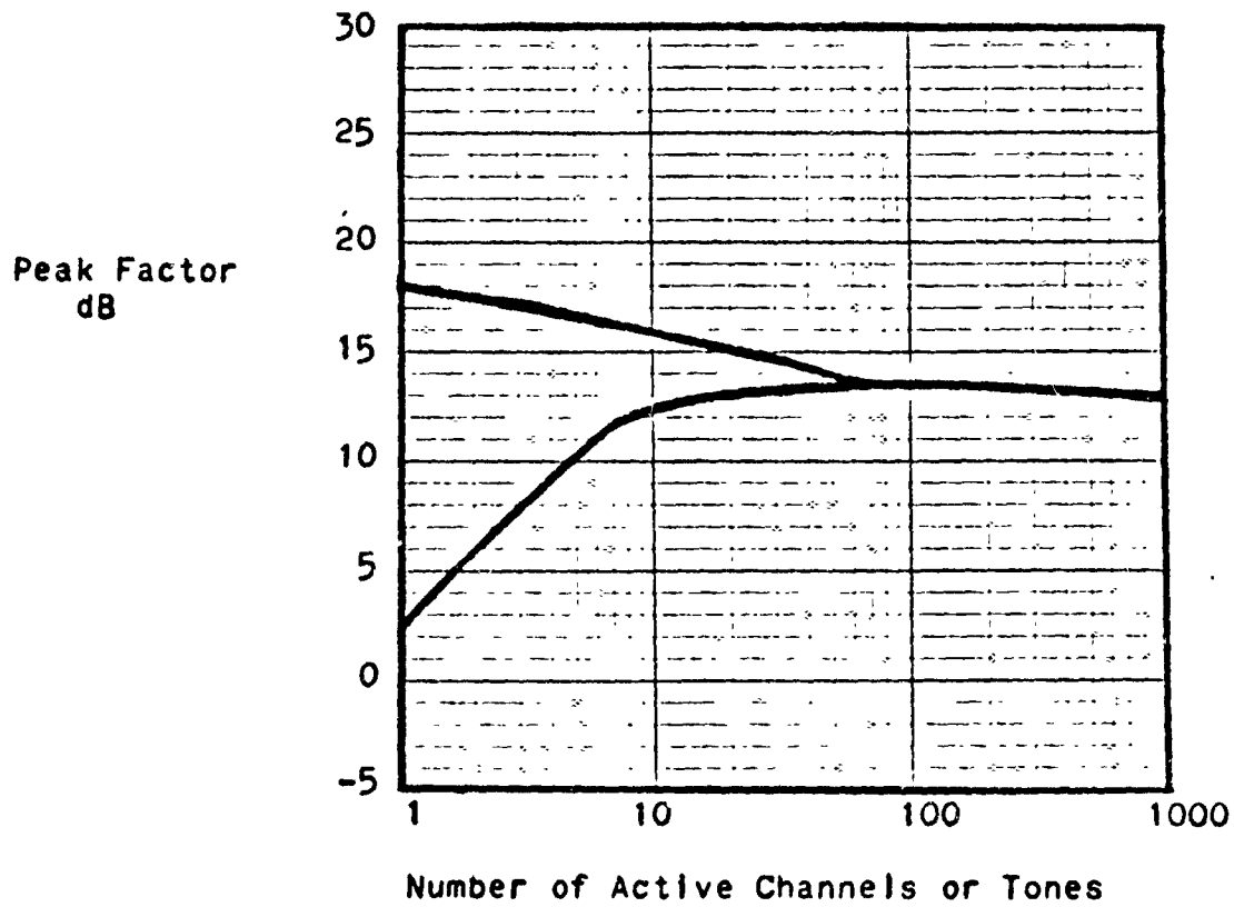
Figure 18- Multichannel Peak Factor. Values of Signal Peaks (above RMS) Exceeded Only 1% of the Busiest Hour.
