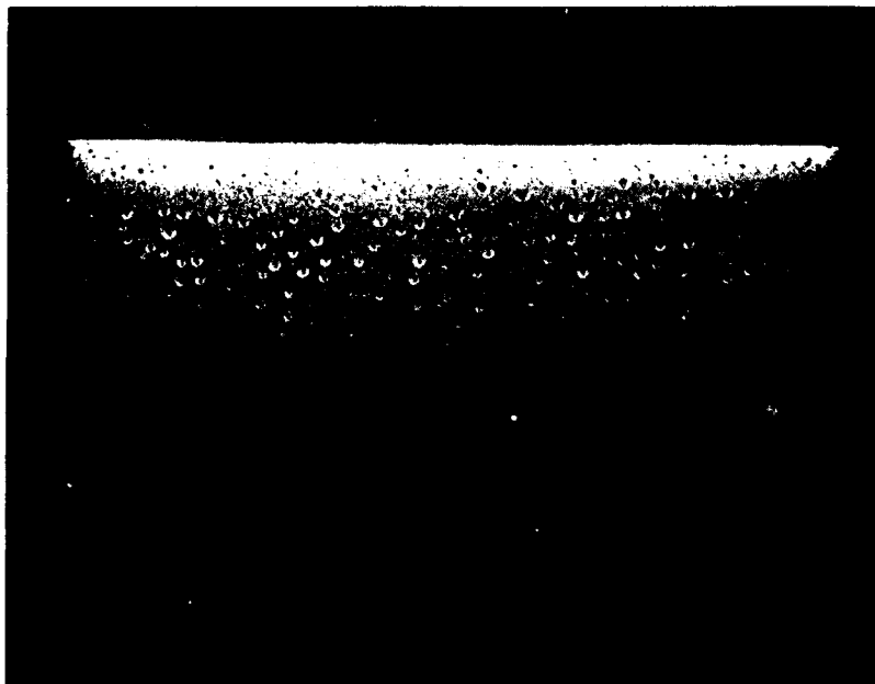
Figure 9. SEM micrograph of unexposed galvanized wire surface. This shows that the zinc outer layer is pitted prior to exposure.
