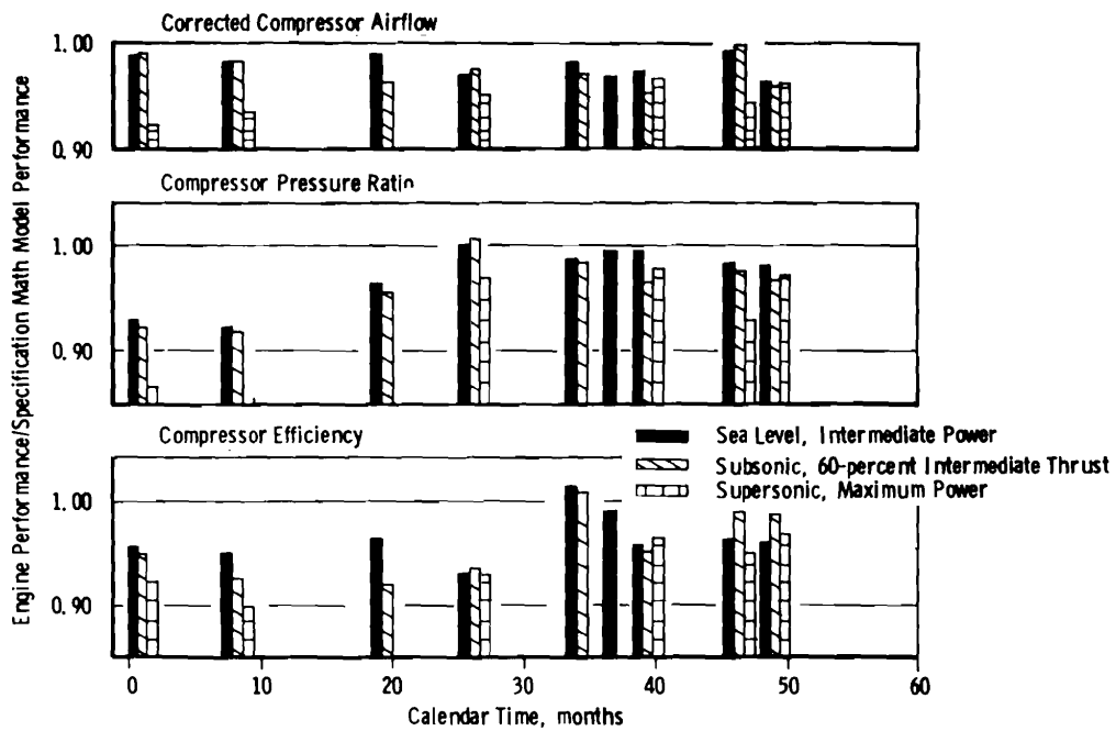
c. High-pressure compressor performance Figure 9. Continued.
