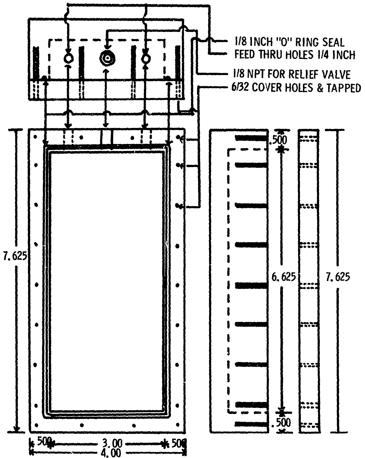
CELL CASE USED FOR EXPERIMENTAL CELL STUDIES
