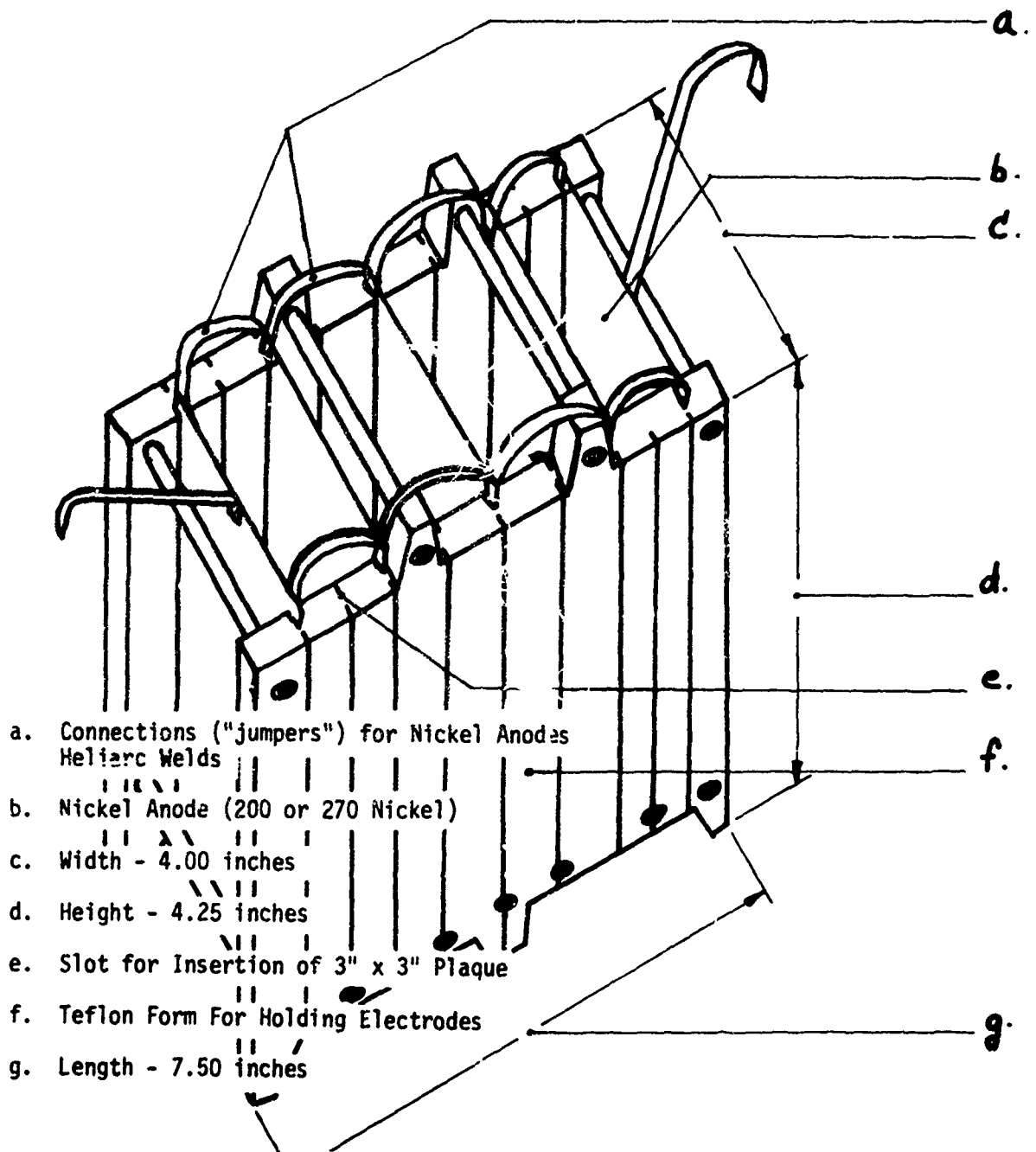
ANNODE ASSEMBLY FOR MULTIPLY PLAQUE IMPREGNATIONS
