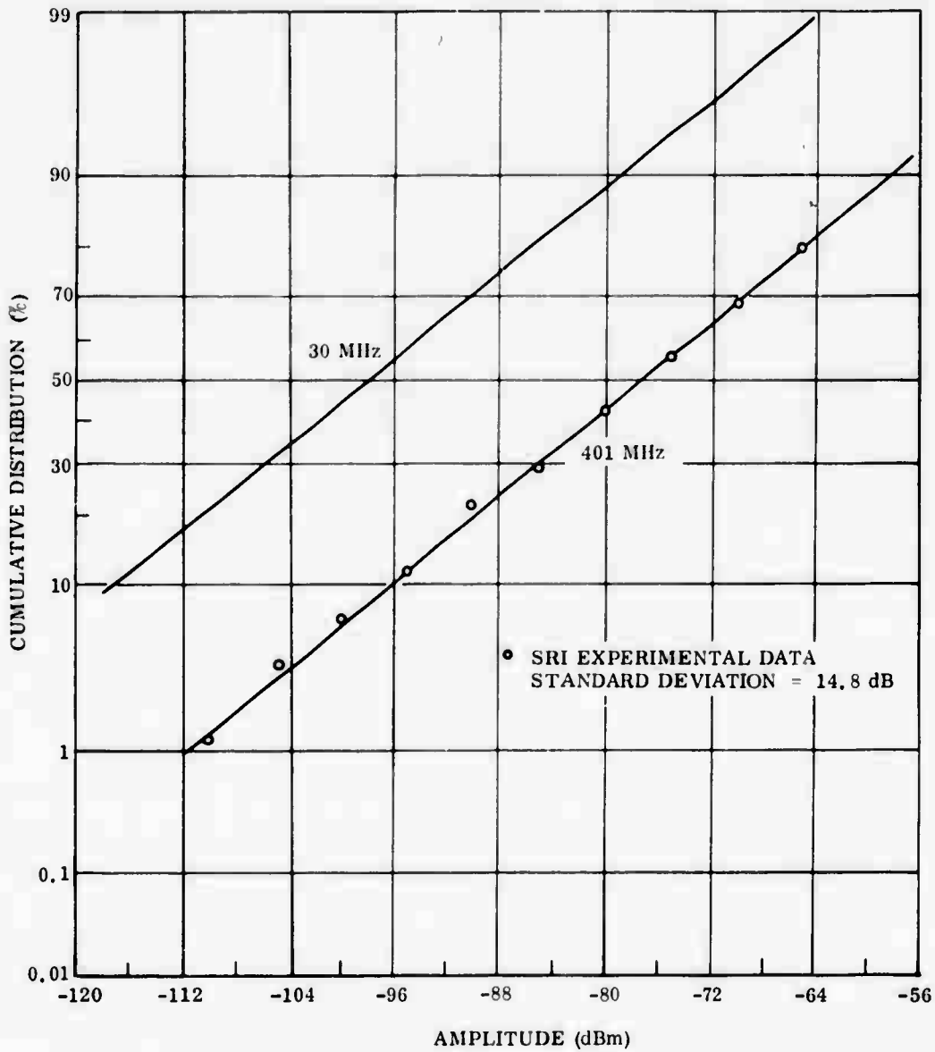
Figure 3-4. Cumulative Distribution Function of SRI Scotland Radar-Auroral Data
