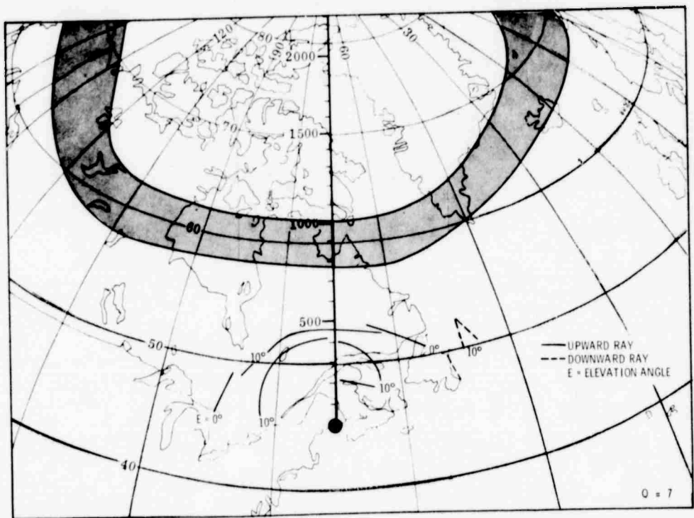
Figure 2-6. Contours of Zero-Degree Aspect Angle for 10 MHz E-Layer Echoes as Viewed from a Midlatitude Location, with the Feldstein-Starkov Auroral Belt Model for Various Levels of Magnetic Activity at 1200 Hours Local Time, Daytime Ionospheric Model B
