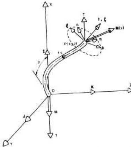
Fig. 1 — Coordinate systems and free-body diagram of cable section OP
