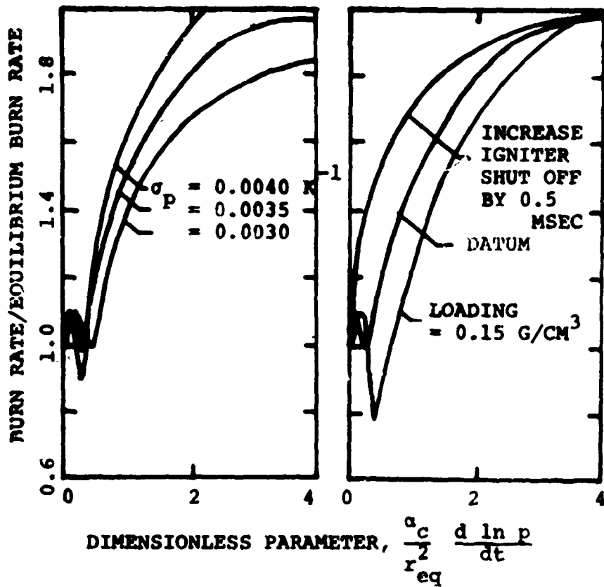
Fig. 9 Dynamic burning rates are not single valued with respect to a widely used dimensionless p parameter.
