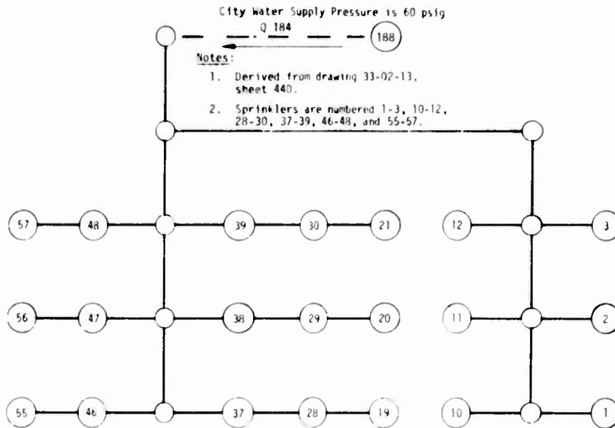
Figure 10. Sprinkler System in Air Materiels Command Warehouses at Robins Air Force Base
