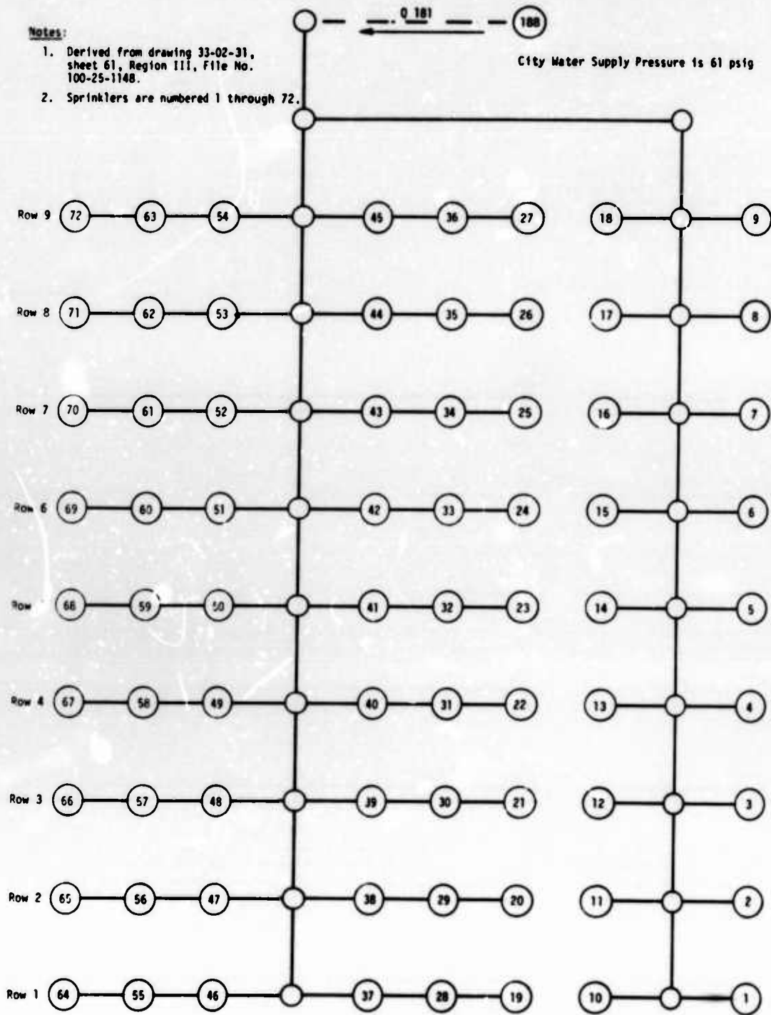
Figure 5. Sprinkler System in Building 786 at McClellan Air Force Base
