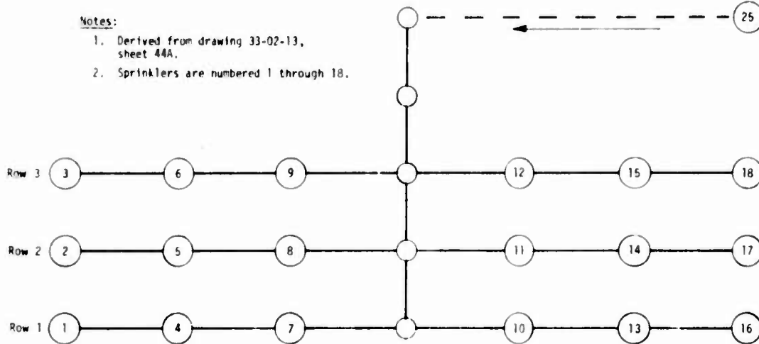
Figure 8. Small Sprinkler System in Buildings 350, 368, and 660 at Robins Air Force Base
