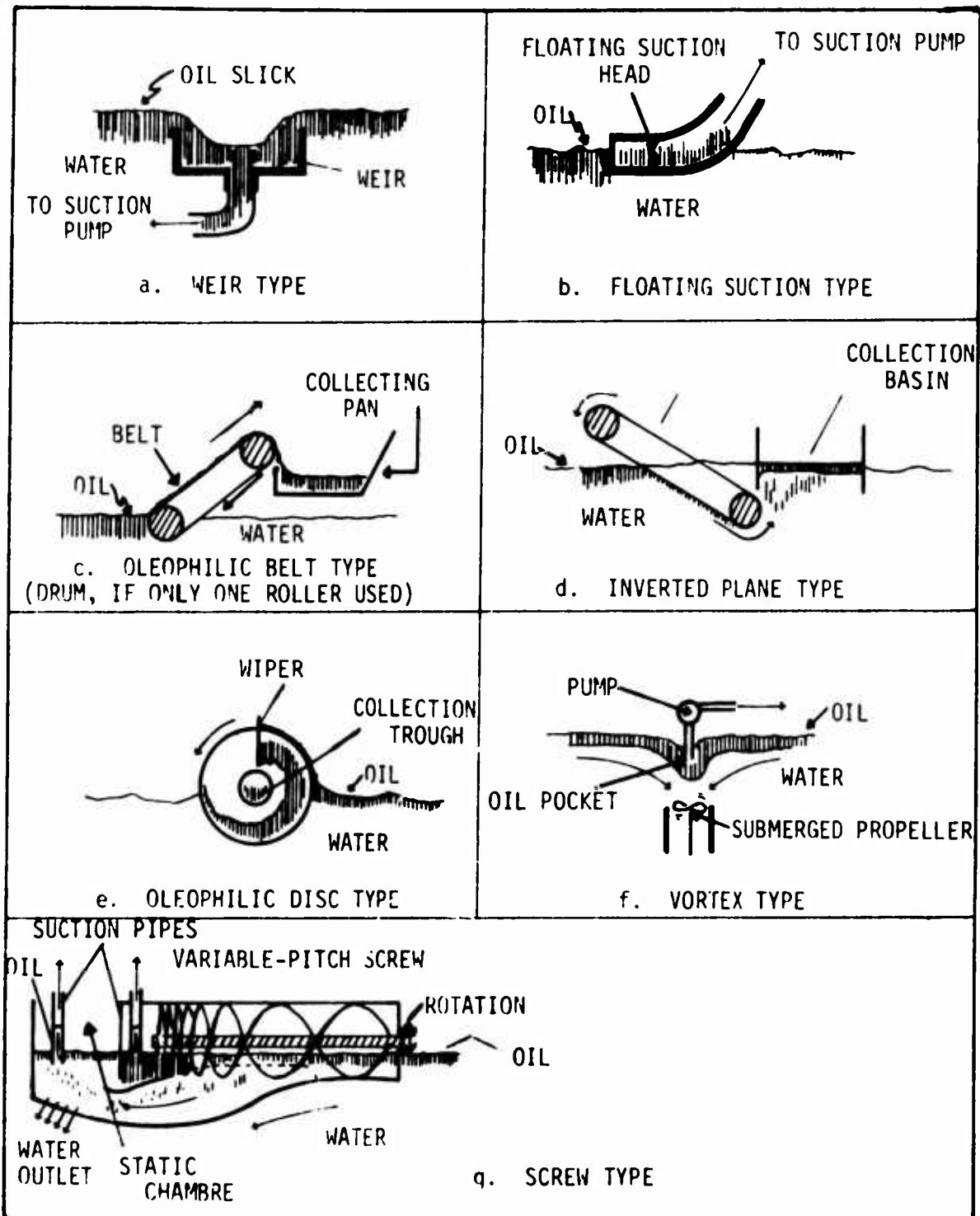
FIGURE 6-5. CLEANUP DEVICE TYPES
