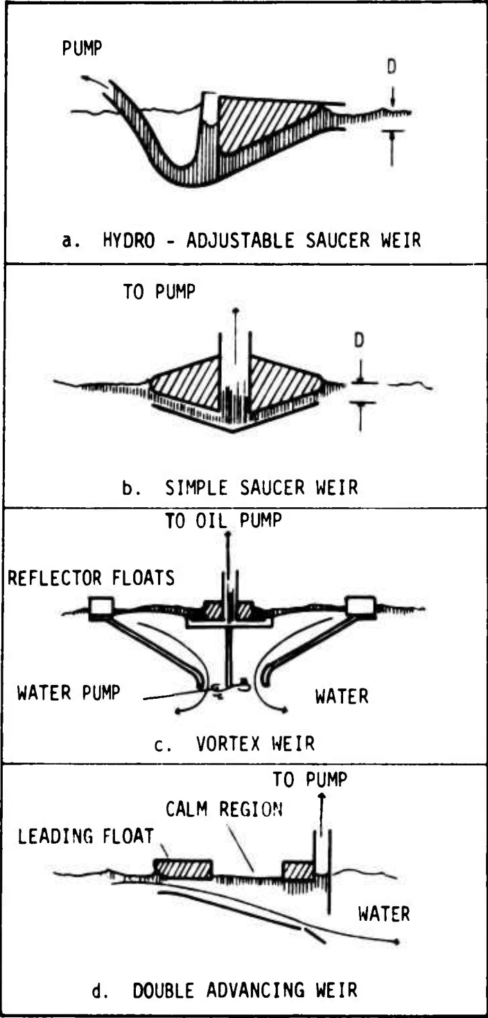
FIGURE 6-6 . WEIR TYPE VARIATIONS
