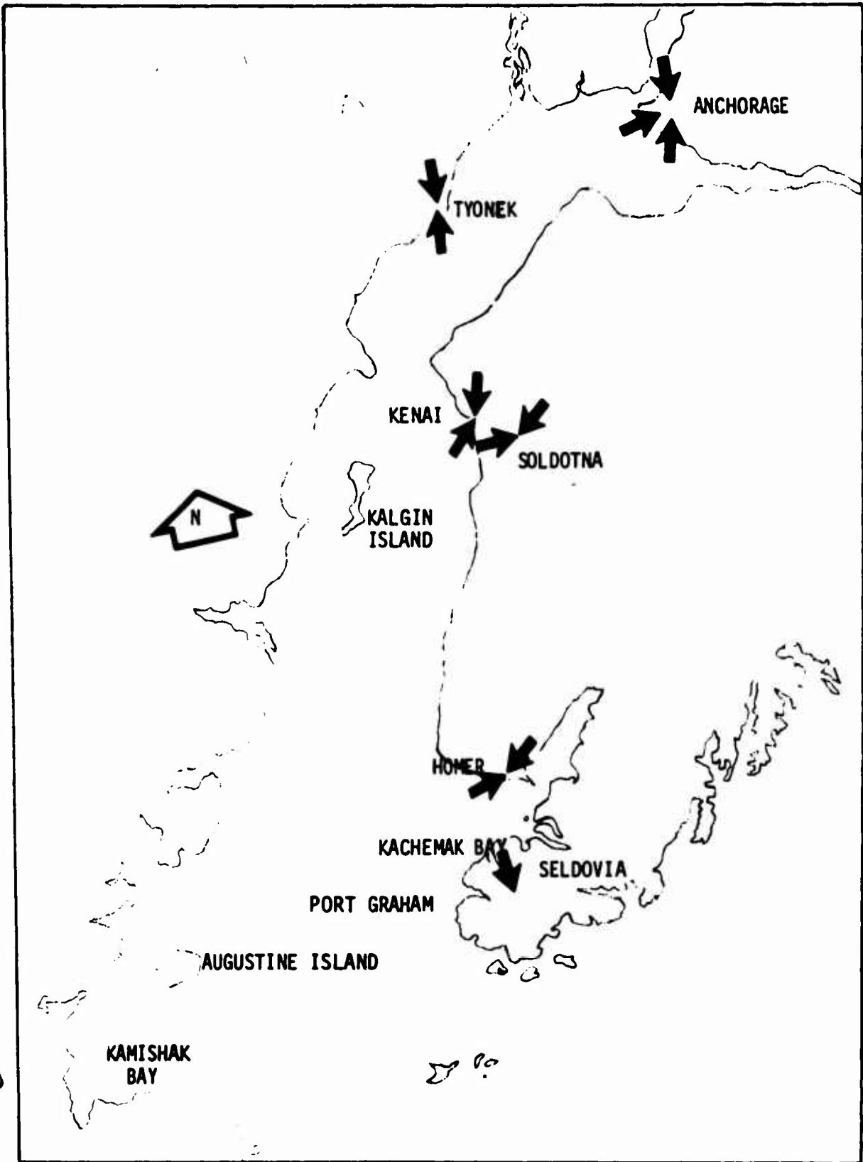
FIGURE 8-6. COOK INLET PREDOMINANT SURFACE WINDS
