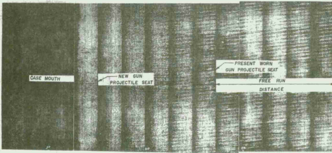
PHD-0828-4-74 FIGURE 4 5" MK 18-O S/N 7, AFTER 1500 RDS. OF PYRD. EXTREMELY WORN GUN
