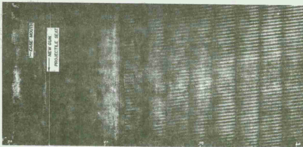
PHD-0828-4-74 FIGURE 3 6"/54 MK 18-4 S/N 868, AFTER 3000 RDS. OF HACO FIRING SCHEDULE 5 RPM FOR 600 RDS. WORST CASE HACO WEAR BUT ONLY SLIGHTLY WORN BY NORMAL STANDARDS.
