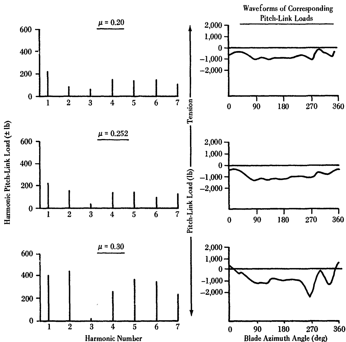
Figure 9. Stall Effects on Harmonic Pitch-Link Loads With a Damper Rate of 500 Lb-Sec/In. ( C_T/\bar{\sigma} = 0.105 ).
