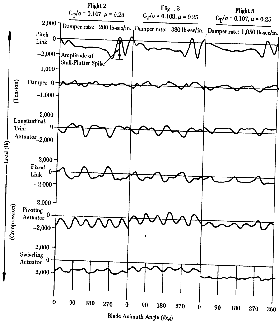
Figure 11. Aft-Rotor Control and Damper Loads for Three Damper Configurations.
