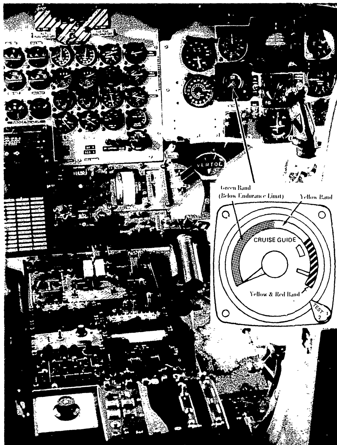
Figure 7. Cockpit Instrument Panel of Test Aircraft With Cruise-Guide Indicator Installed.
