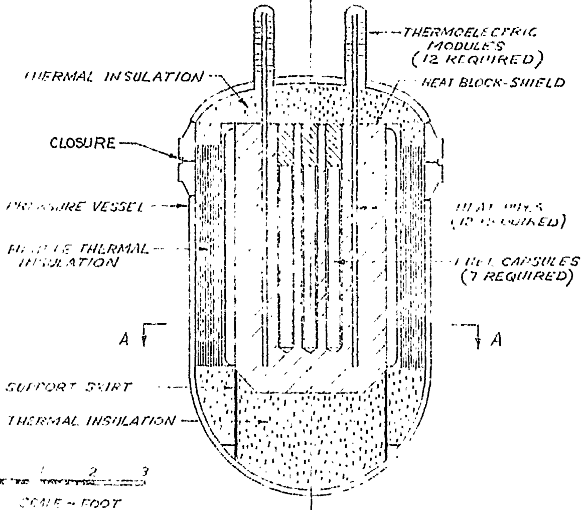
FIGURE 1.1 REFERENCE DESIGN
