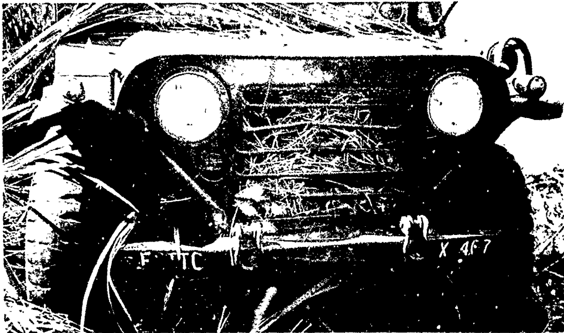
Figure 15. Grass Embedded in Radiator of M151A1, ¼-Ton Truck.
