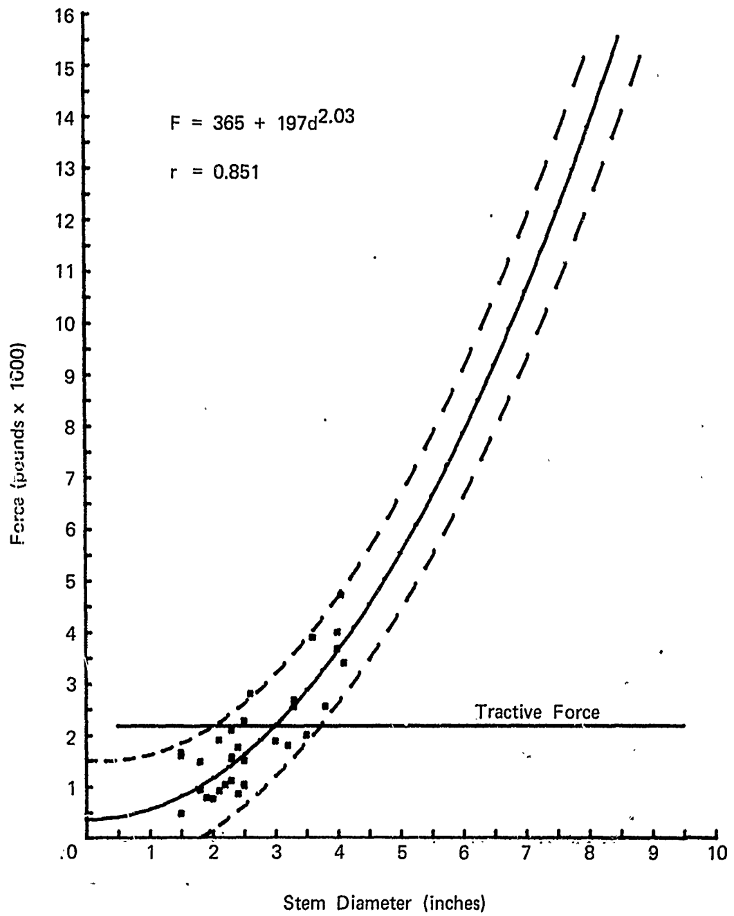
Figure 16. Force Required to Fail a Tree with M151A1; 1/4-Ton Truck.
