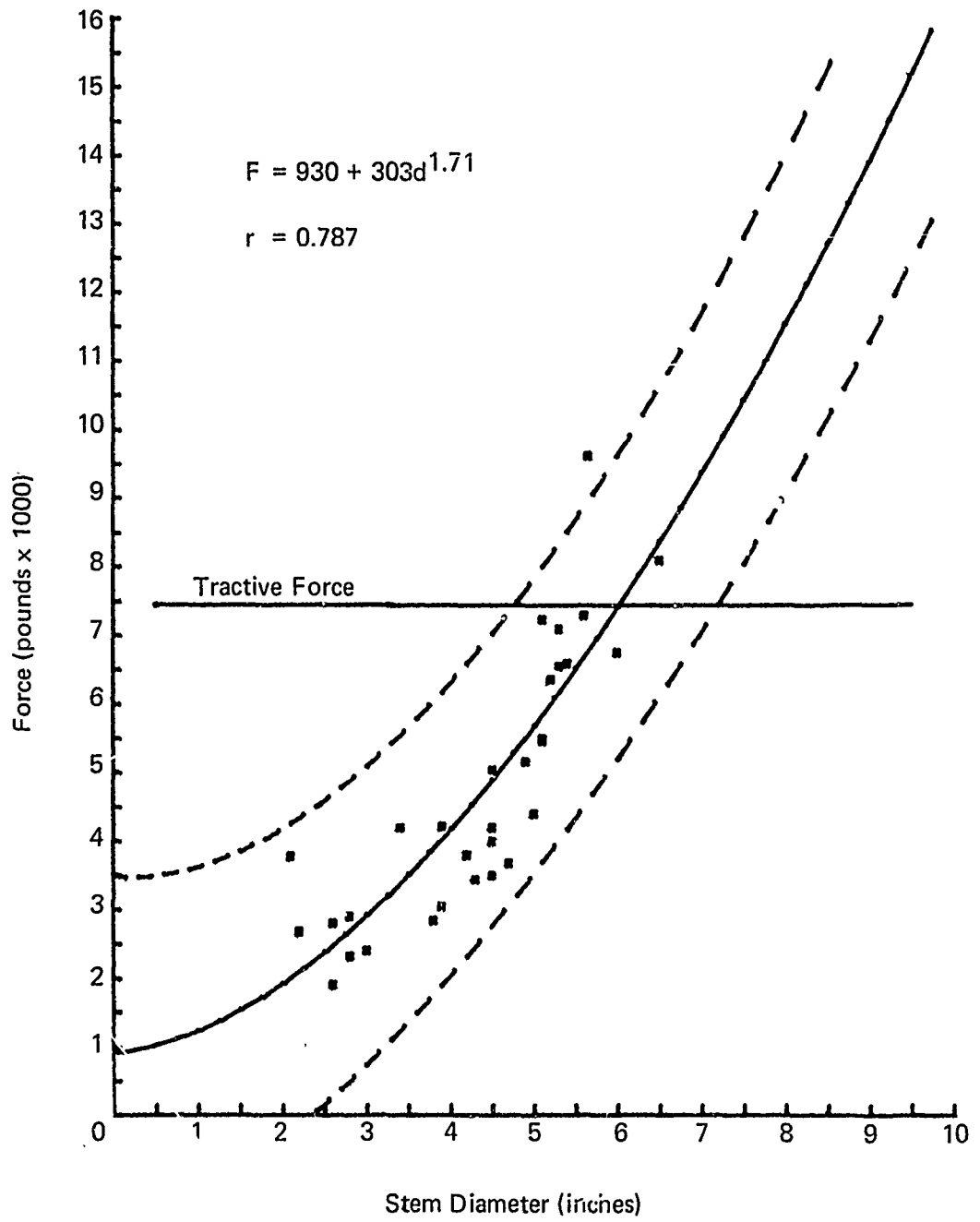
Figure 23. Force Required to Fail and Override a Tree with M715, 5/4-Ton Truck.
