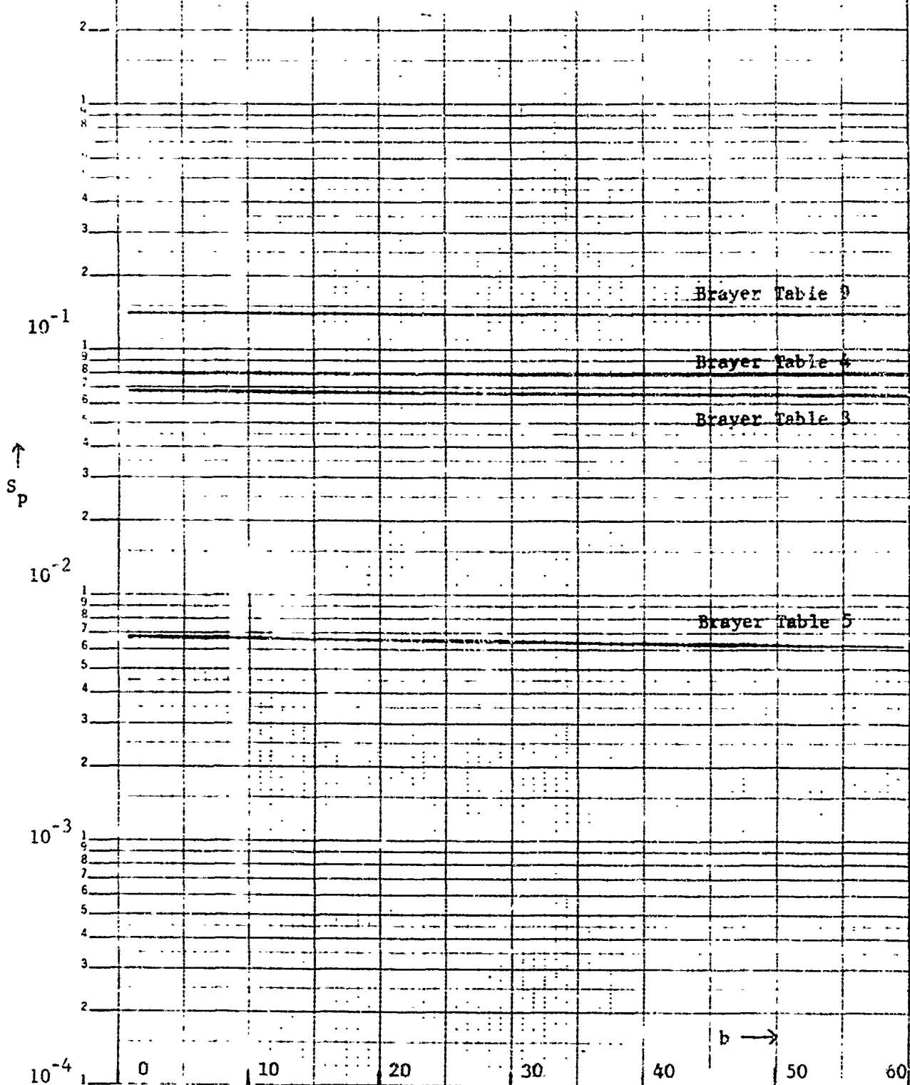
Figure A.20. S_p(b, 2000) versus b for models as noted on the curves
