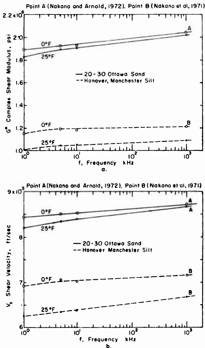
Figure 19. The effect of frequency on complex shear modulus and on shear velocity at a dynamic stress of 0.1 psi.
