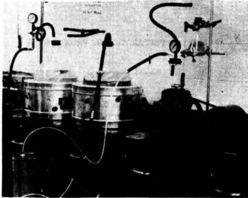
Figure C2. Saturation apparatus.
