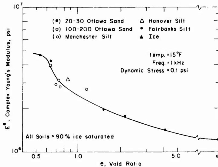
Figure 14. The effect of void ratio on complex Young's modulus.
