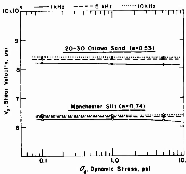
Figure 22. The effect of dynamic stress and frequency on shear velocity.
