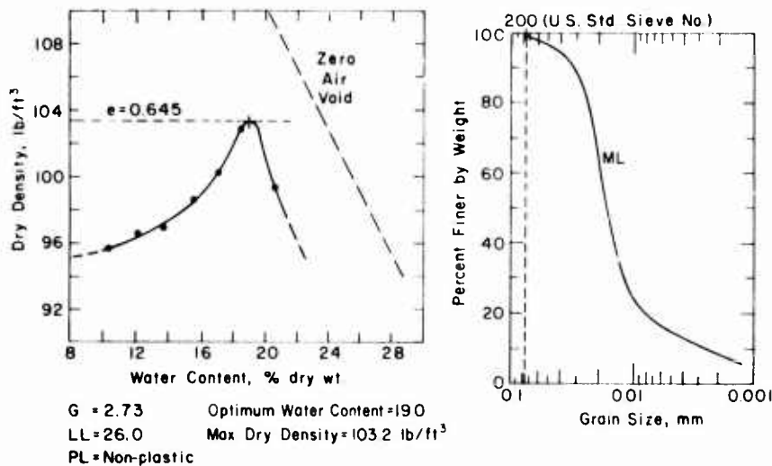
Figure 10. Manchester silt compaction test results.
