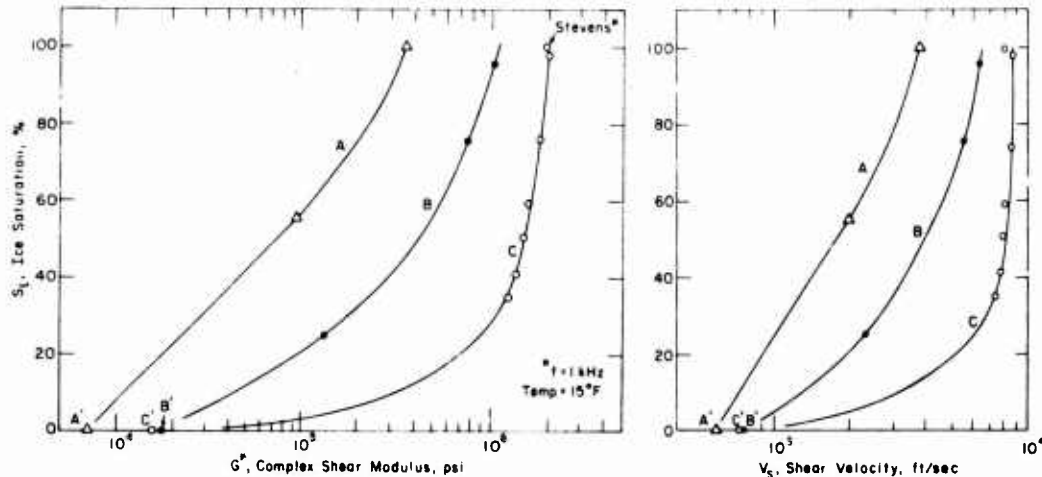
Figure 12. The effect of ice saturation on complex shear modulus and shear velocity.
