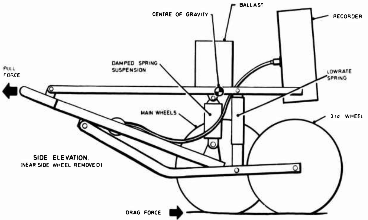
FIGURE A-3. DIAGRAMMATIC LAYOUT OF MU METER
