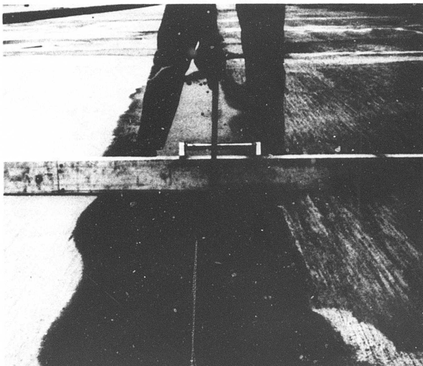
Photo 25. Collection of water along longitudinal construction joint
