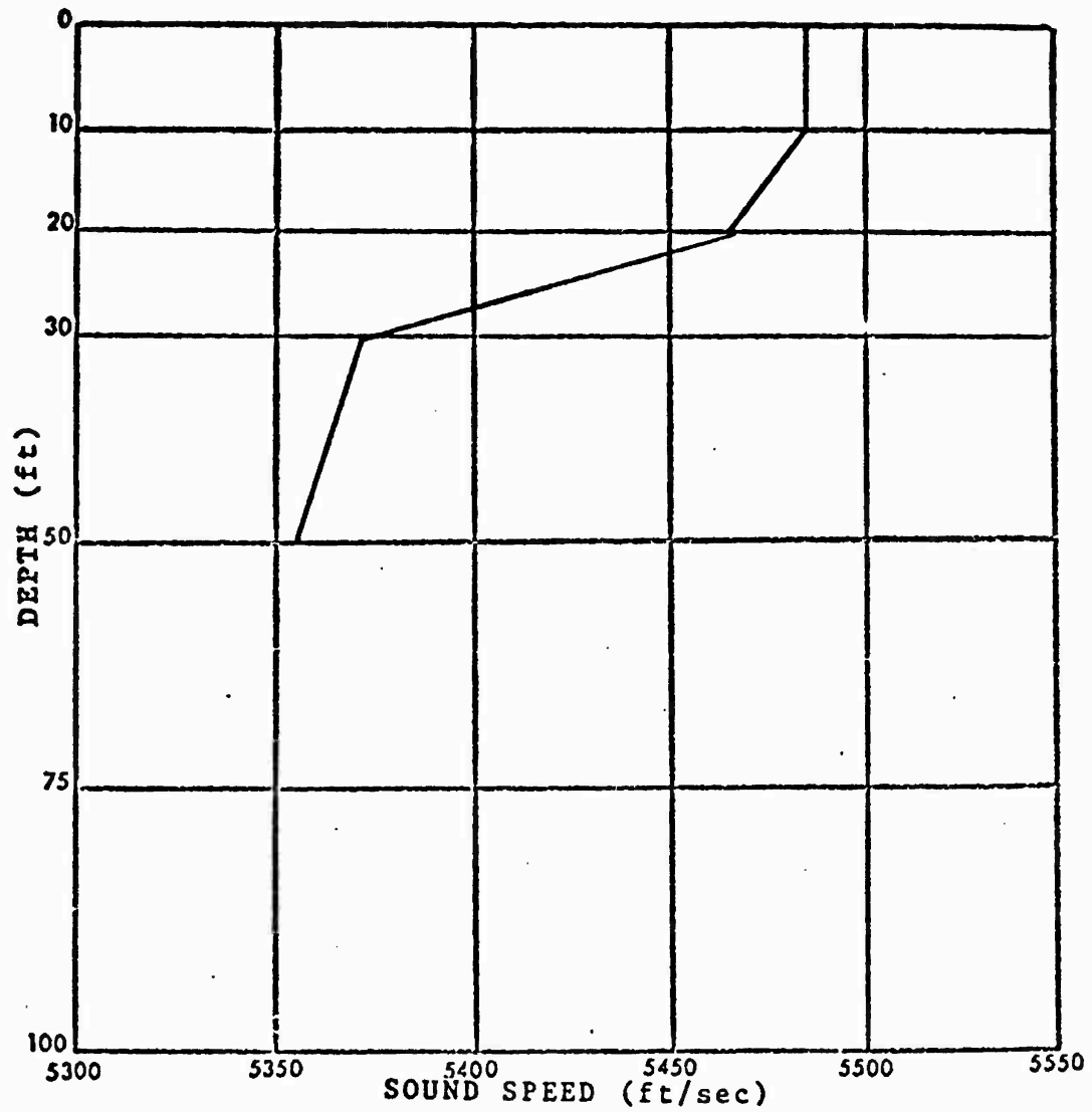
Figure D-9 . Sound speed profile, summer, area I
