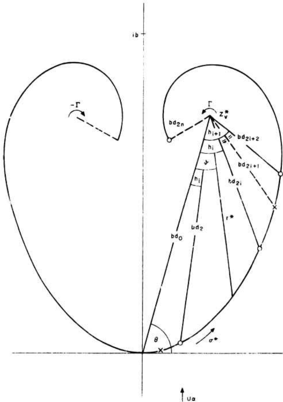
Figure 1B. Configuration in transformed plane, Z^* = y^* + iz^* \circ , Pivotal points; \times , intermediate points. [after Smith (1960)].
