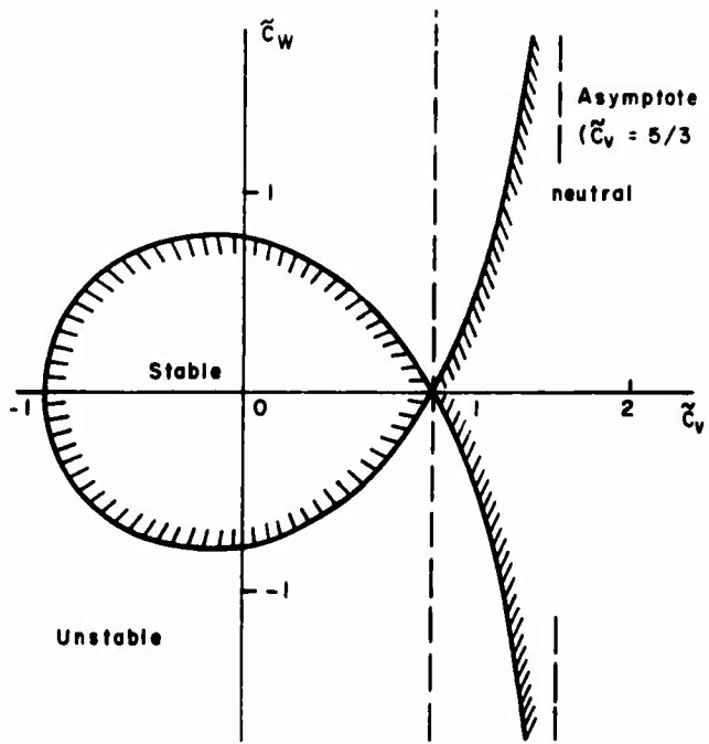
Figure 7. Stable and unstable regions in the \tilde{\zeta}_w, \tilde{\zeta}_v Plane [after Ludwig (1961)].
