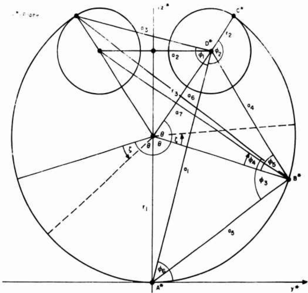
Figure 15. Notation in transformed plane [after Mangler and Smith (1957)].
