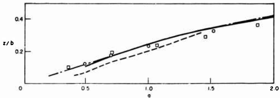
Figure 21. Vortex sheet shape (top), horizontal (middle) and vertical (bottom) position of vortex center [after Pullin (1973)].
