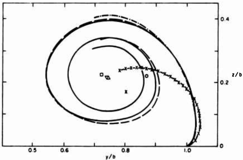
Figure 19. Vortex sheet shapes and isolated vortex positions for a = 0.91 . o, Brown & Michael (1954); x and —x—, Mangler & Smith (1959); □ and —□—, present calculation, n = 14 ; Δ and —Δ—, present calculation, n = 21 ; ▽ and —▽—, present calculation, n = 39 [after Smith (1968)].
