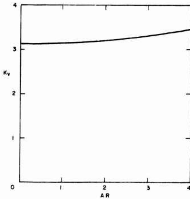
Figure 28. Variation of K_p (top) and K_v (bottom) with aspect ratio [after Polhamus (1966)].
