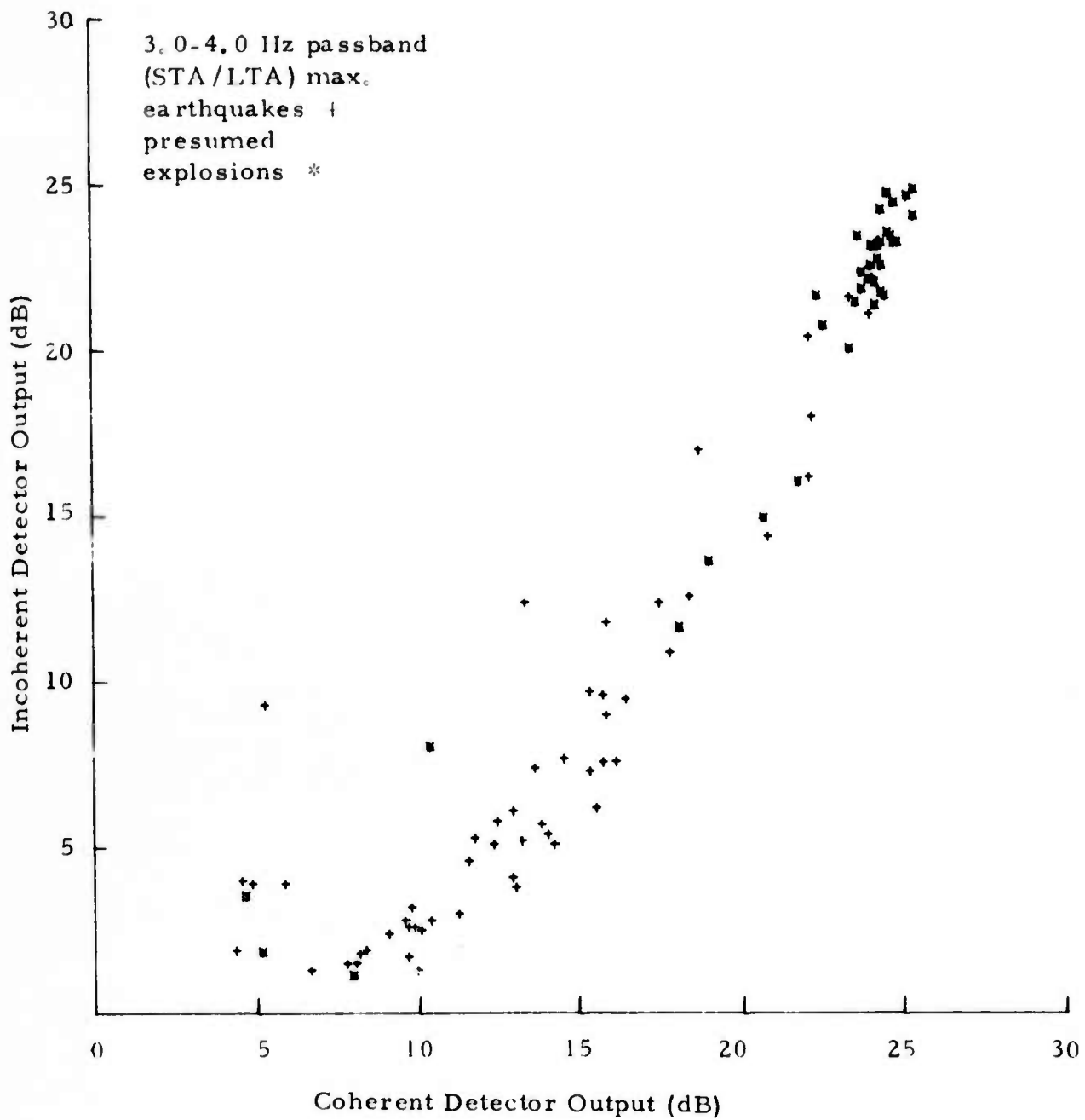
FIGURE IV-18 COHERENT ADJUSTED-DELAY DETECTOR OUTPUT VERSUS INCOHERENT DETECTOR OUTPUT ( (STA/LTA) max IN THE 3.0-4.0 Hz PASSBAND)
