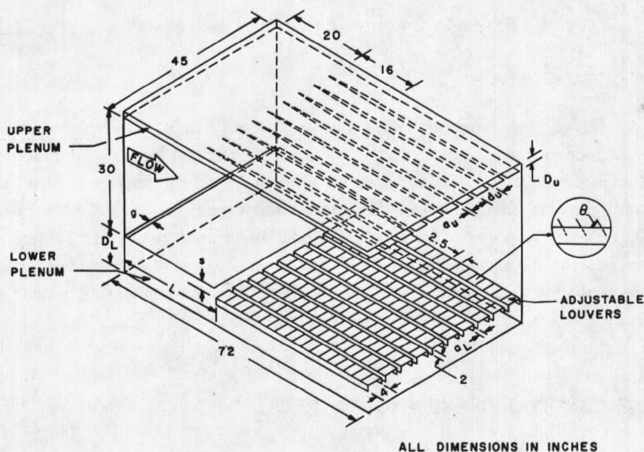
Figure 3. Basic stepped configuration.
