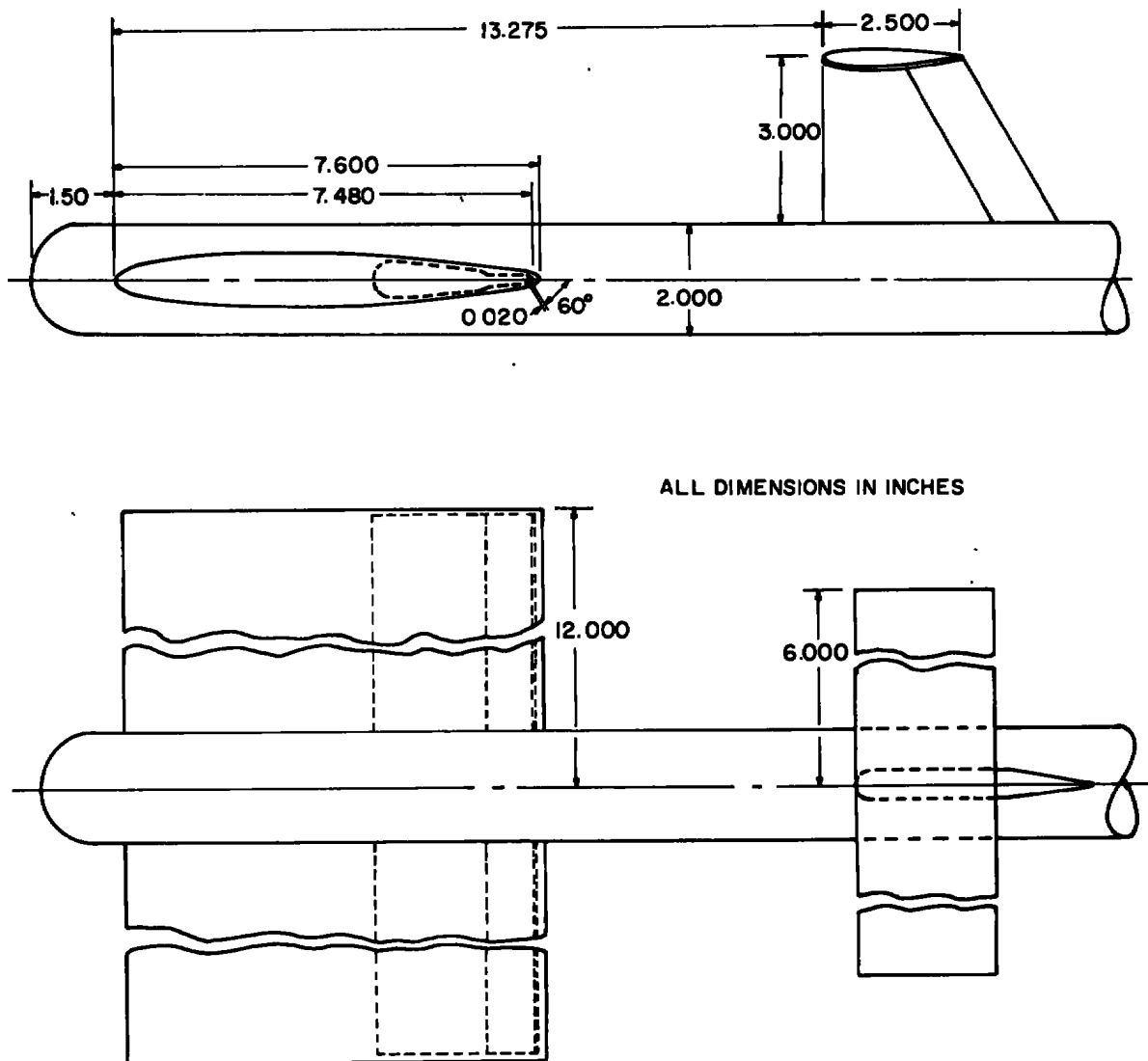
a. Jet-flap model Figure 2. Model dimensions.
