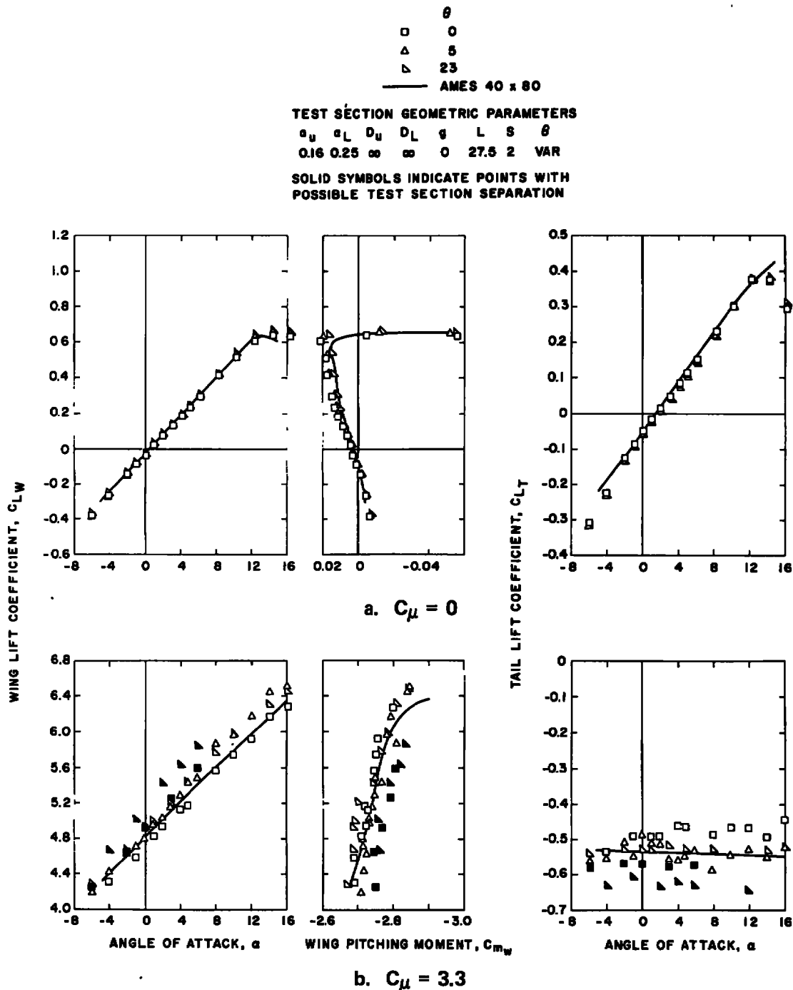
Figure 10. Effect of louver angle on the jet-flap model forces.
