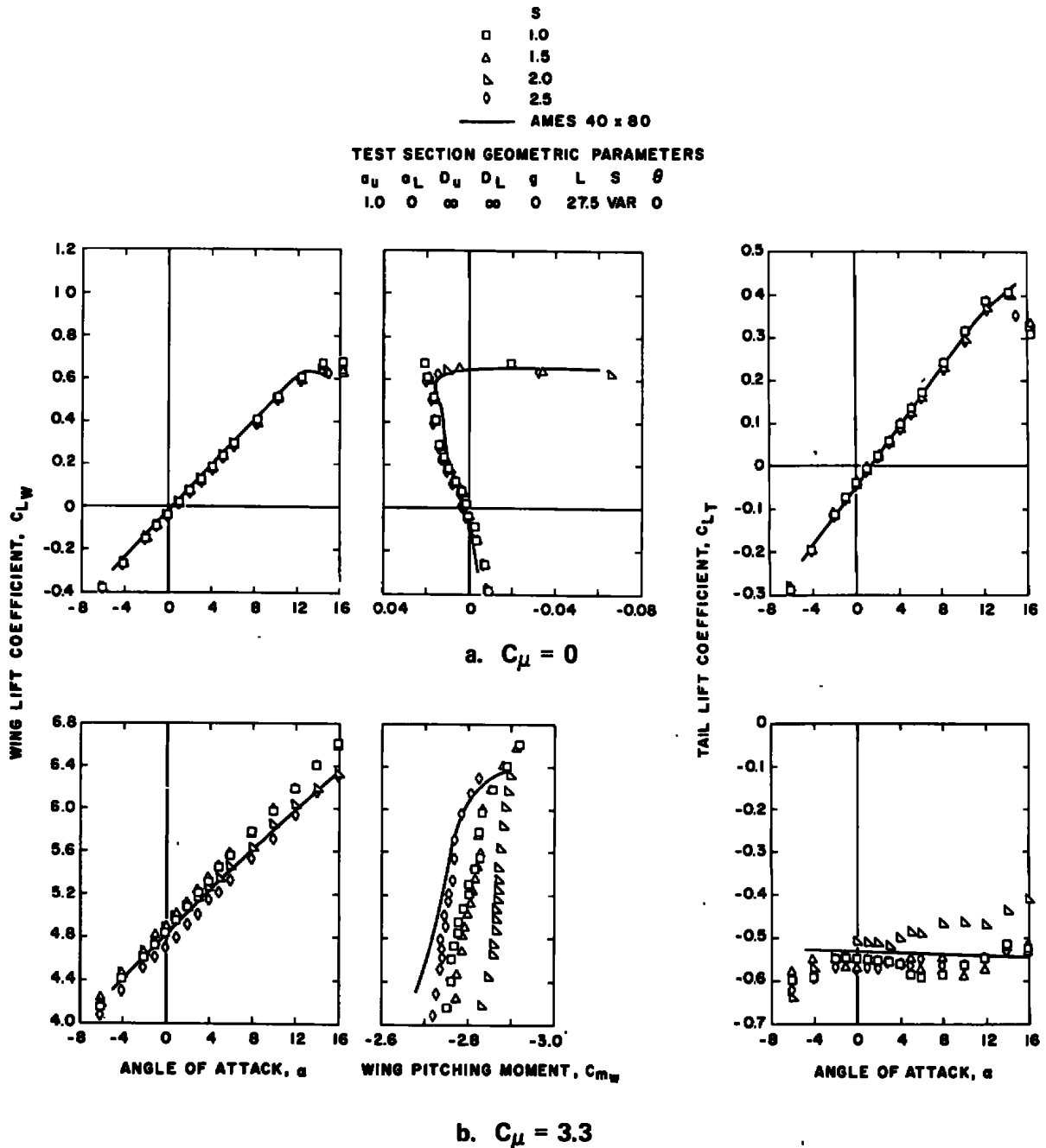
Figure 8. Effect of bottom wall step height on the jet-flap model forces.
