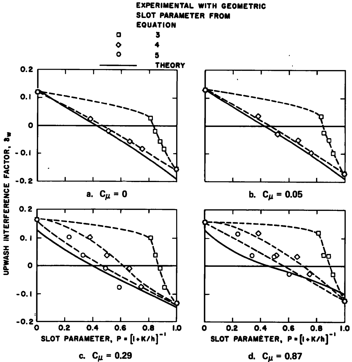
Figure 5. Comparison of experiment and theory.
