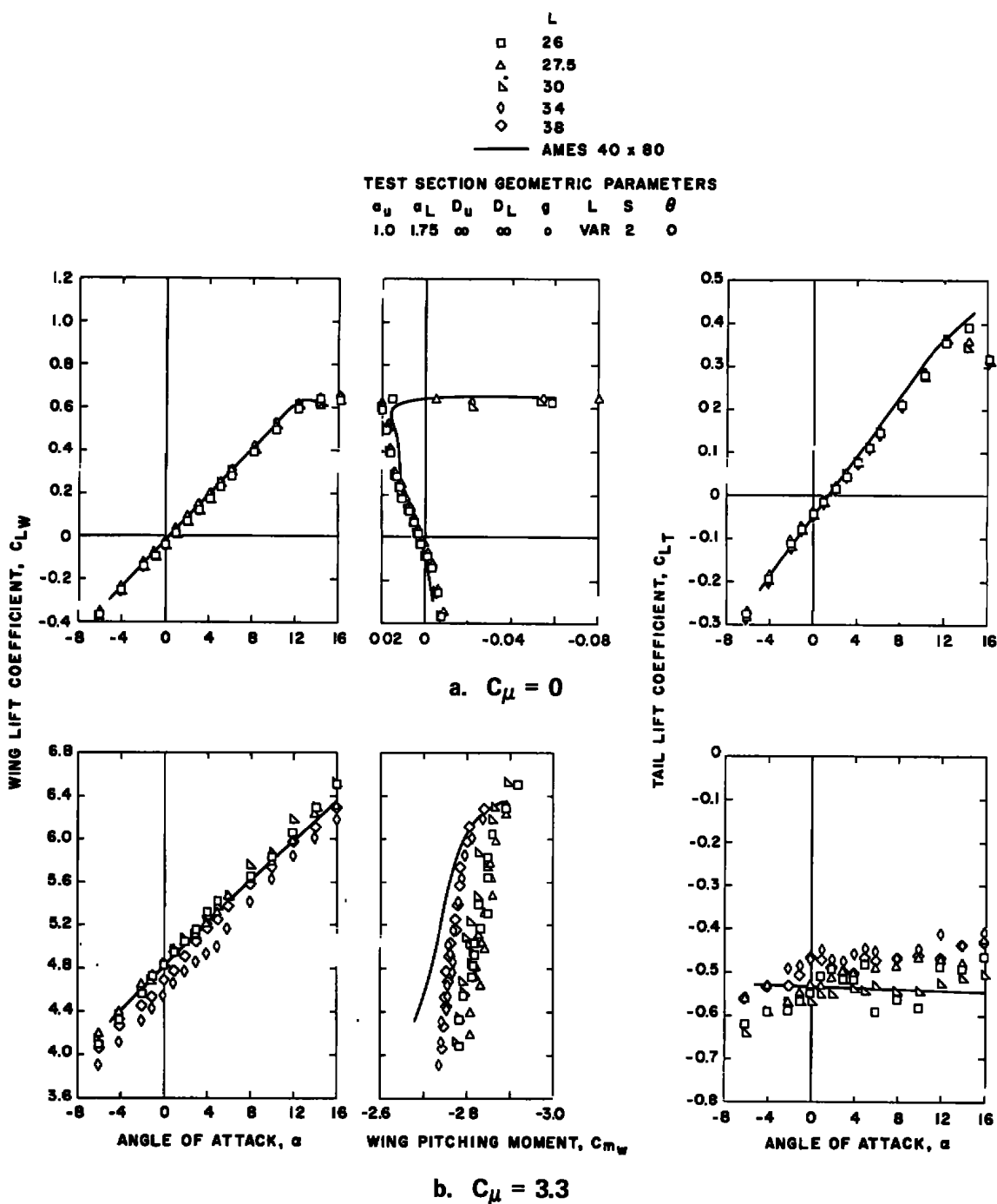
Figure 9. Effect of bottom wall step location on the jet-flap model forces.
