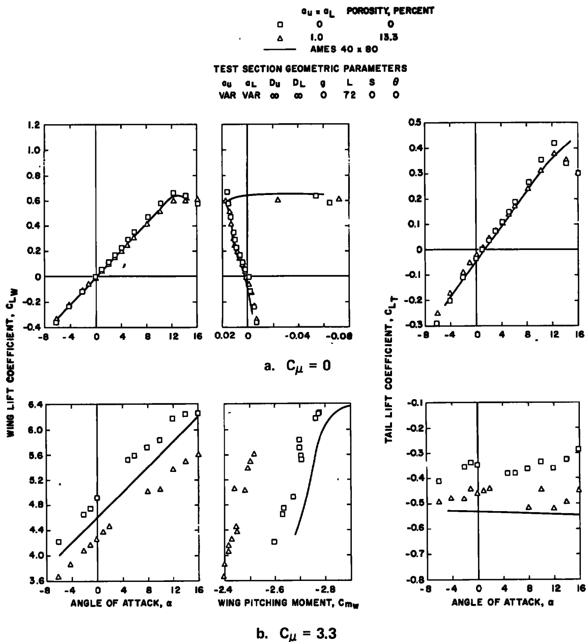
Figure 7. Interference on the jet-flap model with 10 uniform slots in each horizontal wall.
