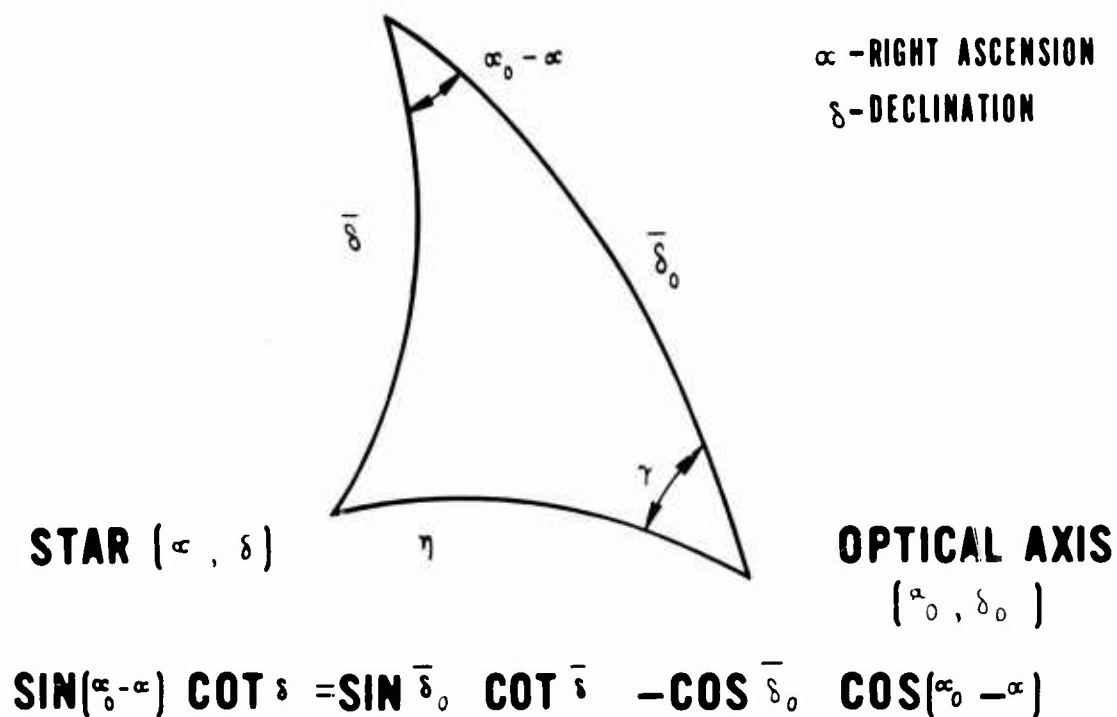
Figure 2. AAPS Geometry
