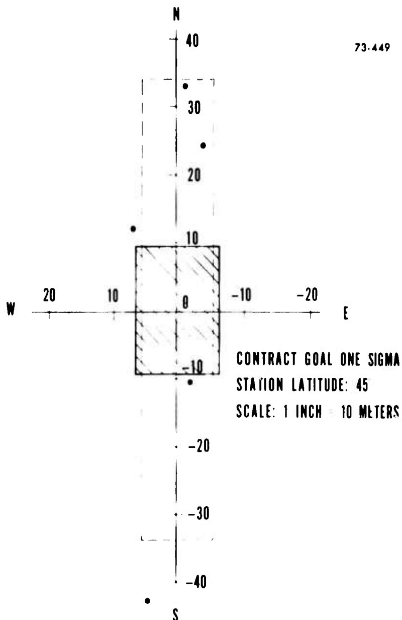
Figure 10. AAPS First Order Position Difference
