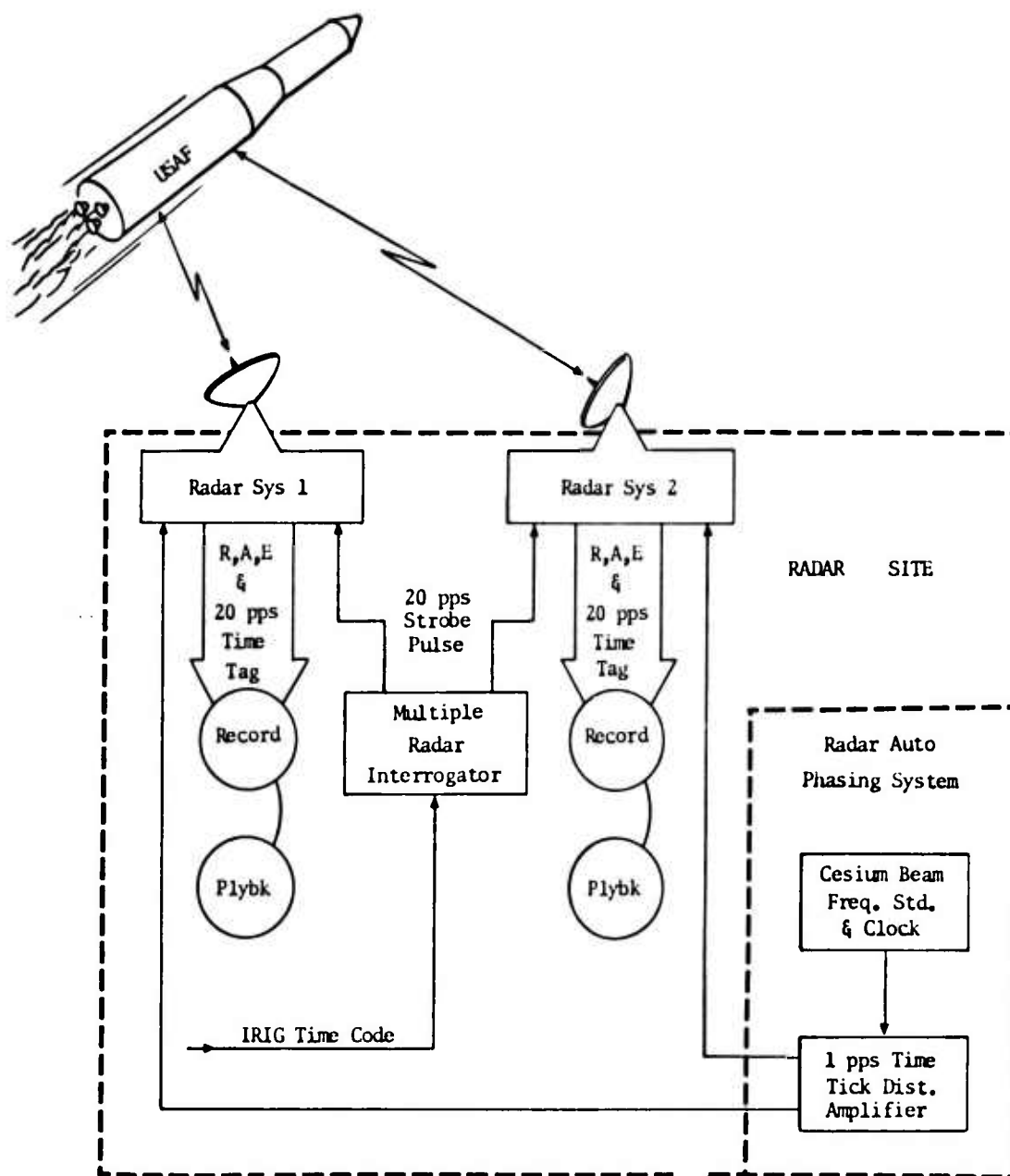
Figure 4. Multiple Radar Interrogator Time Tag Data Synchronization
