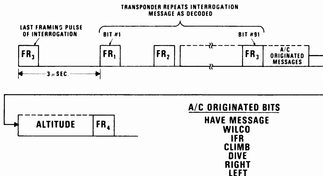
Figure 5. Aircraft Response to DABS Interrogation
