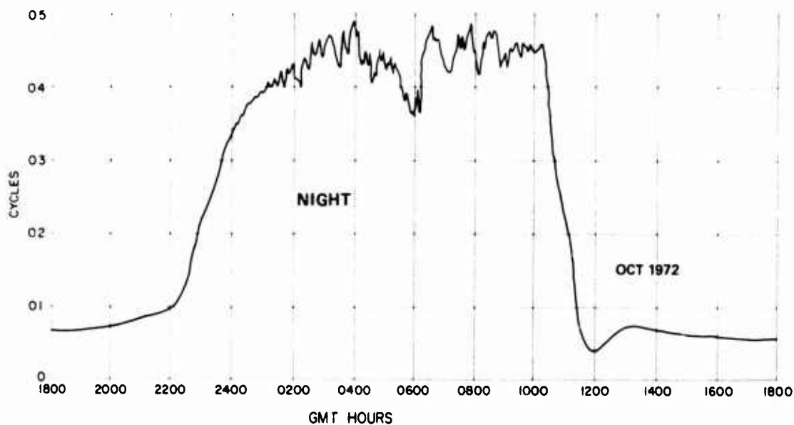
Figure 9. 13.1 KHz Signal from N. Dakota to NELC, San Diego, Ca.
