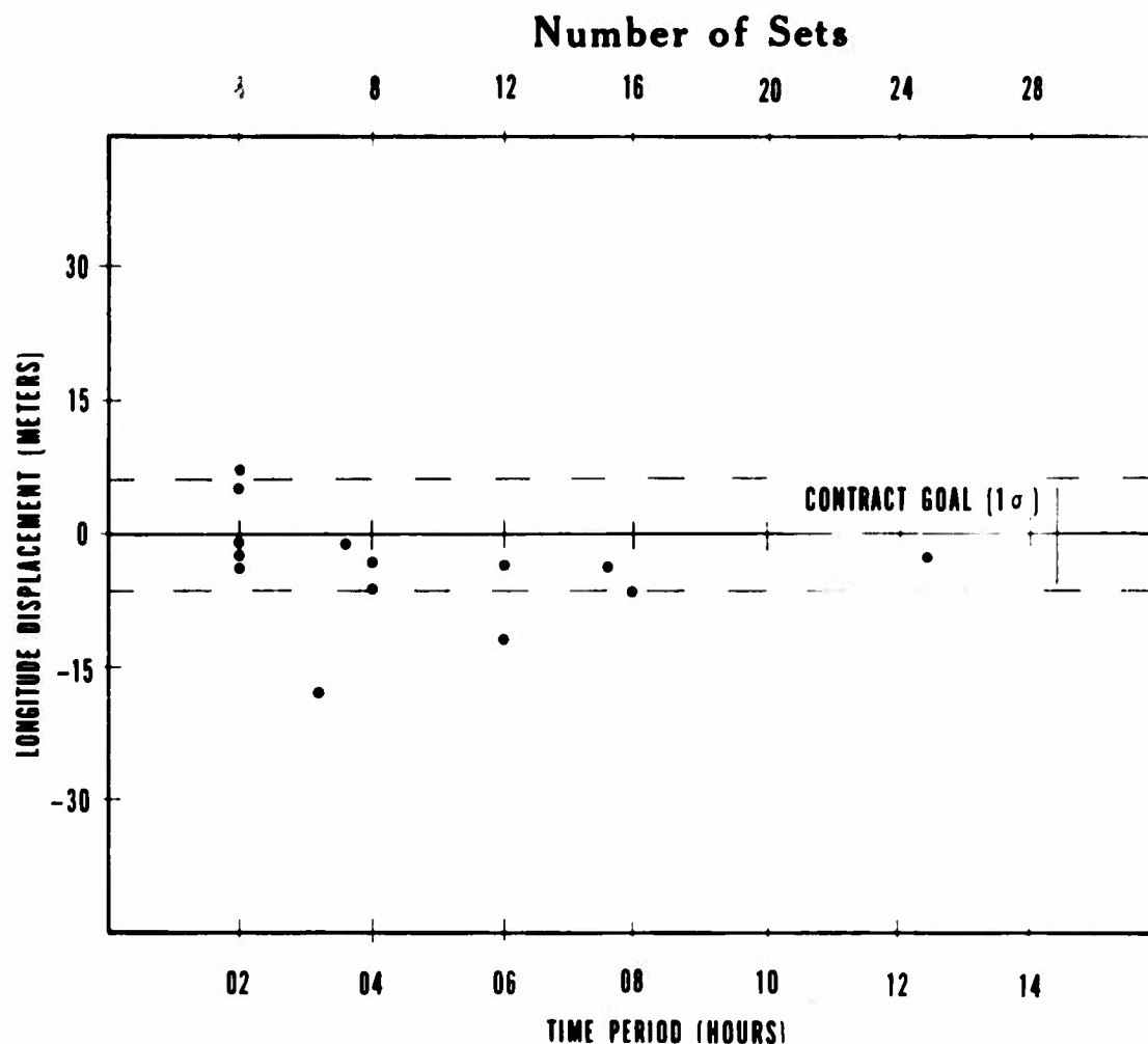
Figure 12. AAPS Accuracy Relative to a Standard
