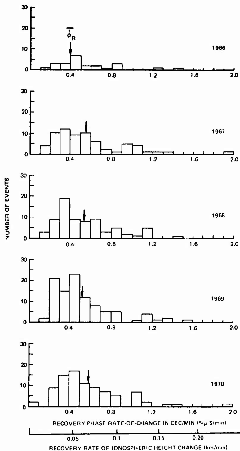
Figure 6. Recovery Phase Rate-of-Change Distributions Observed During SPA Events on Hawaii to New York Path at 10.2 kHz
