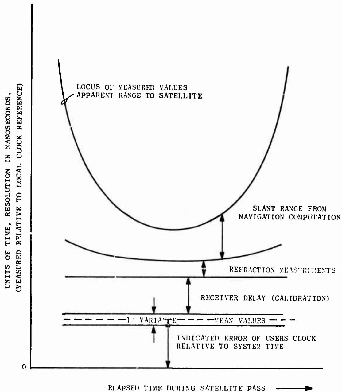
Figure 1. User's Process for Time Calibration of His Local Clock
