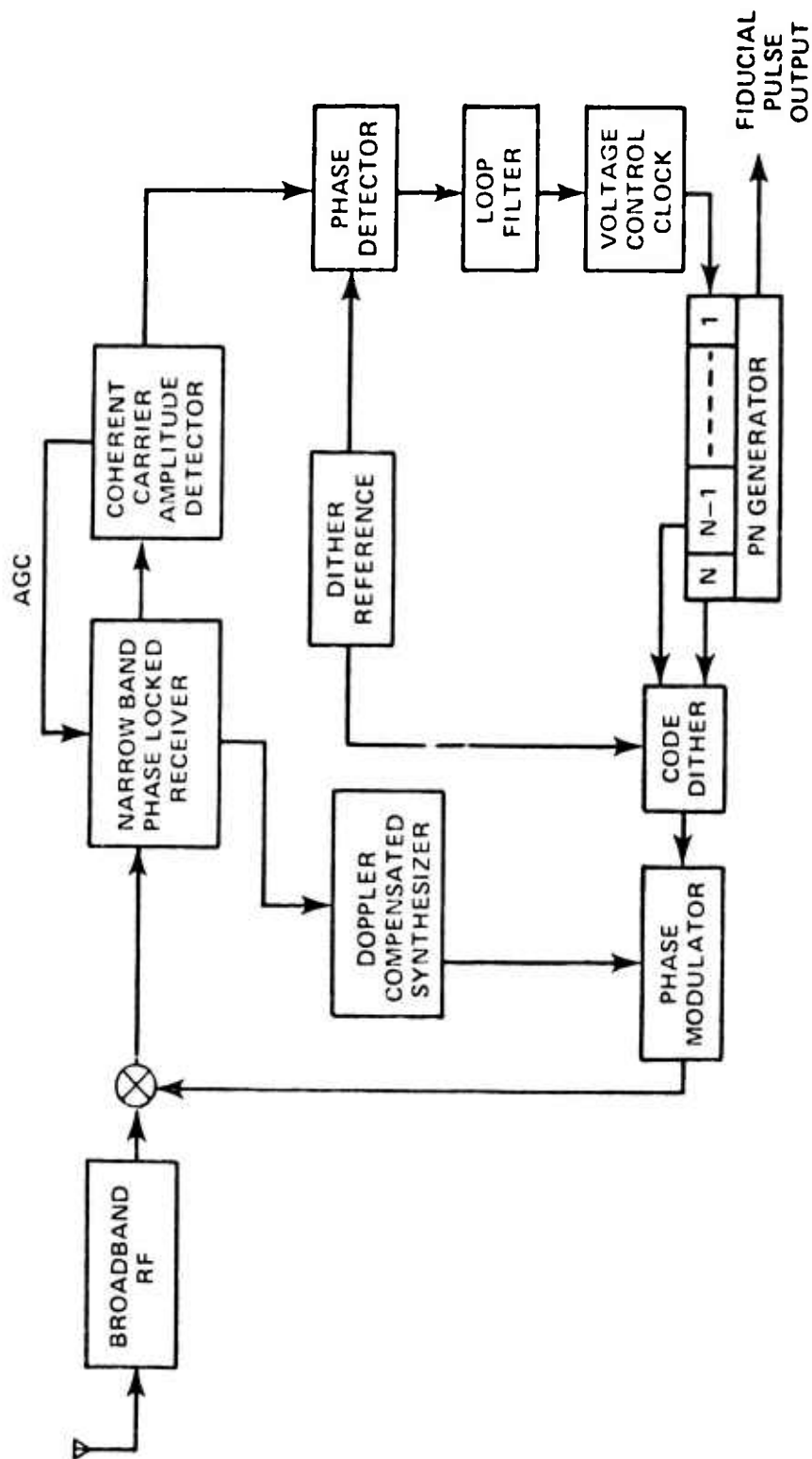
Figure 6. Amplitude Dithered Delay-Locked Receiver for PN Reception
