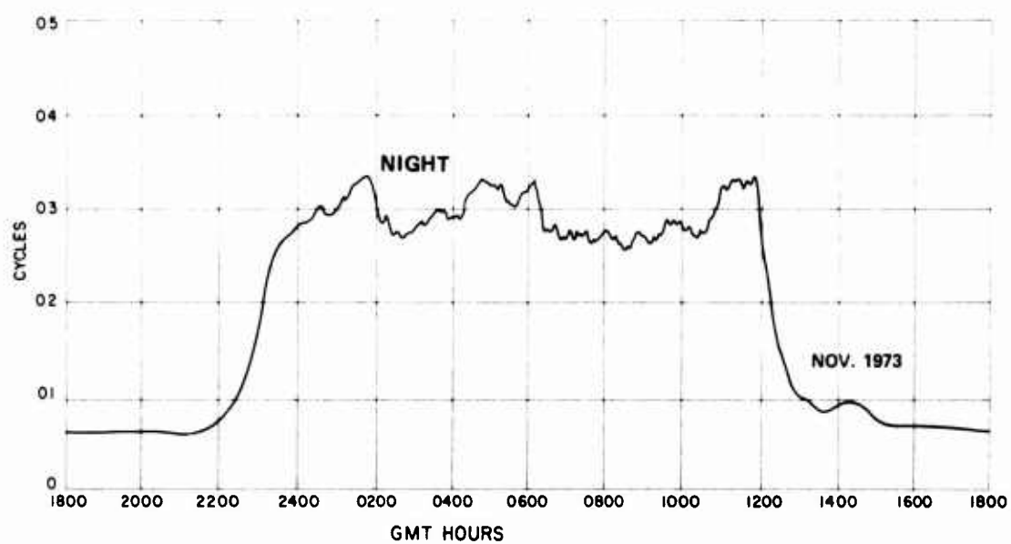
Figure 7. 12.85 KHz Signal from N. Dakota to Rosman, N. C.
