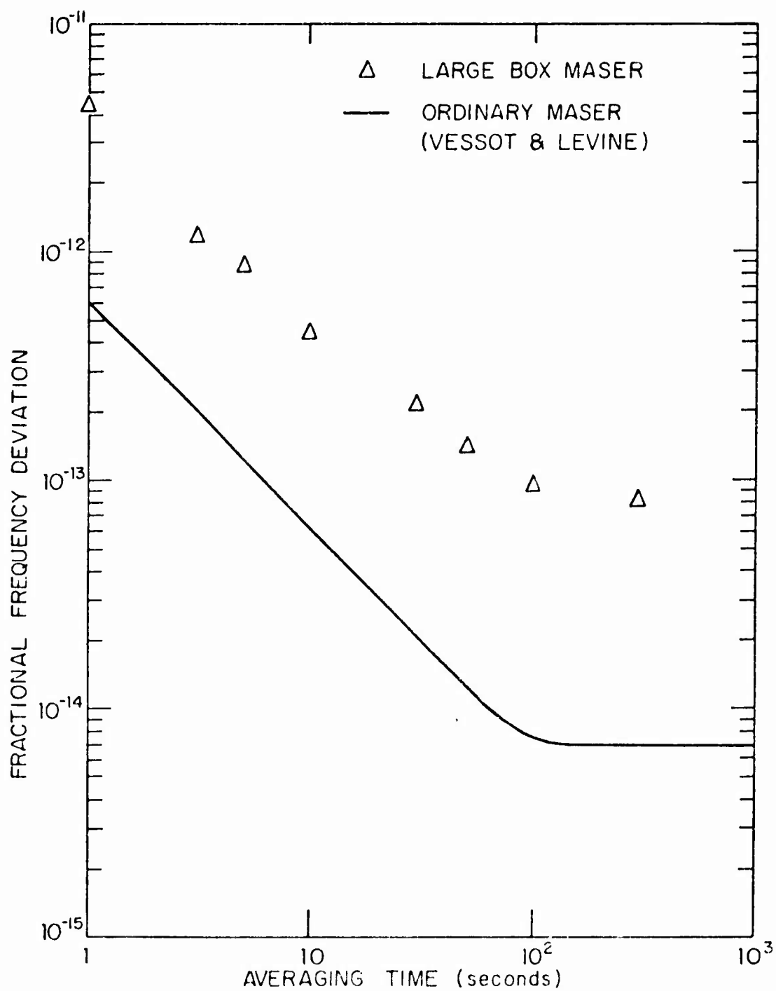
Figure 5. Fractional Frequency Deviations of Large Storage Box Maser (cone out, low flux, \nu_L = 15 kHz)
