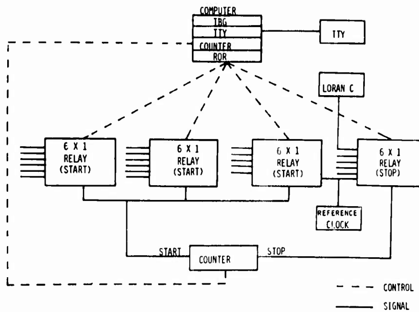
Figure 3. Automatic Time Measurement System
