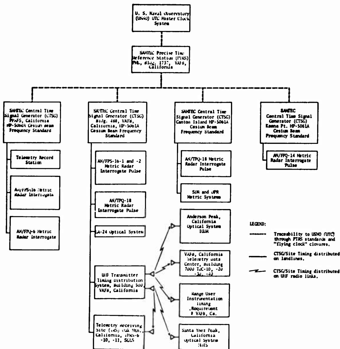
Figure 1. SAMTEC Instrumentation Systems UTC/IRIG Timing and Frequency Accuracy Traceability to USNO
