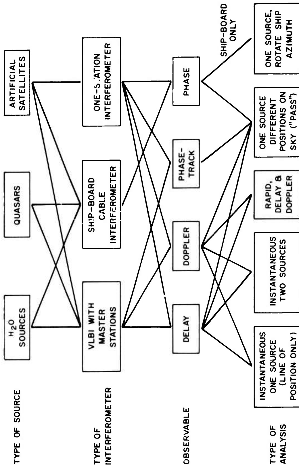
Figure 2. Interferometer Navigation System Operating Modes
