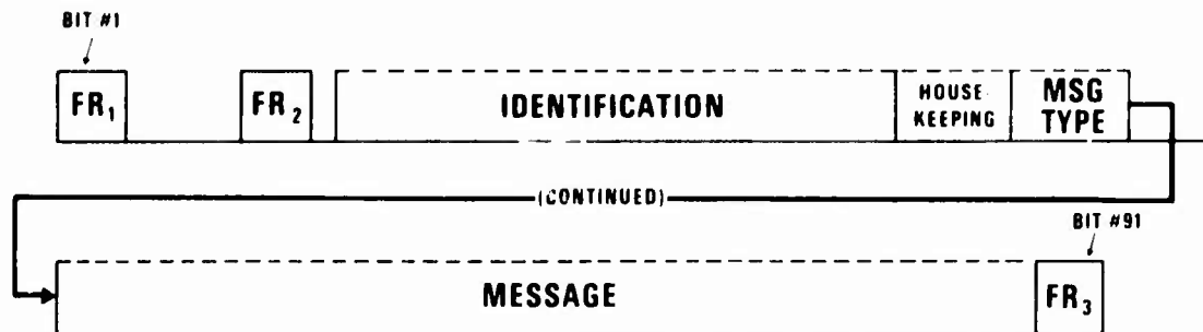
Figure 4. SYNCHRO-DABS Interrogation
