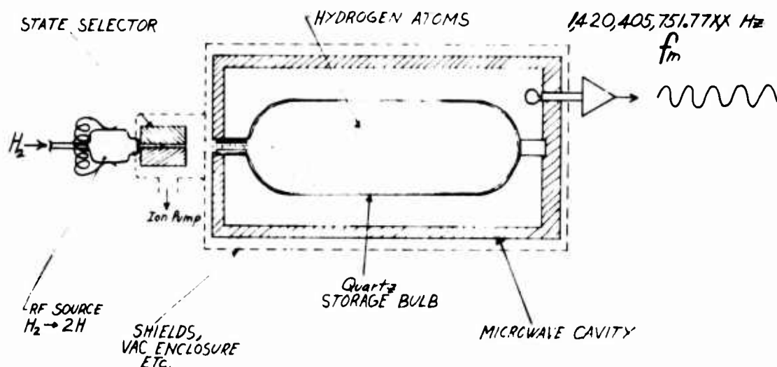
Figure 1. Atomic Hydrogen Maser Schematic
