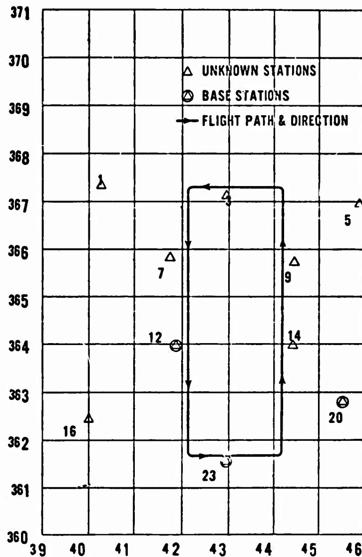
Figure 4. LRPDS Station and Flight Geometry
