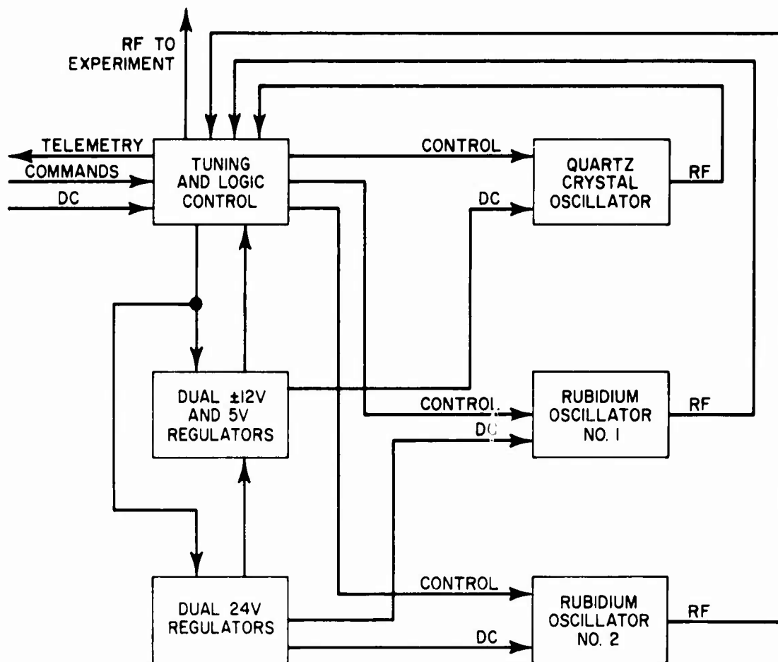
Figure 2. Frequency Standard System Block Diagram
