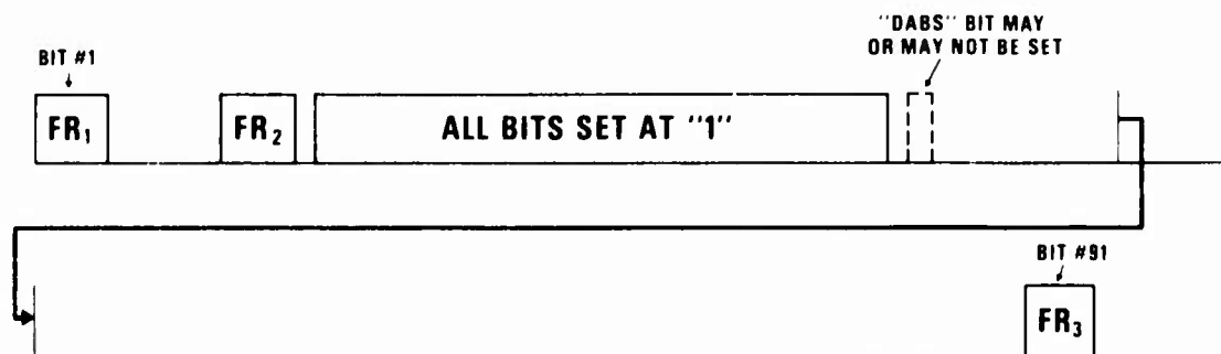
Figure 6. General Call Message Format
