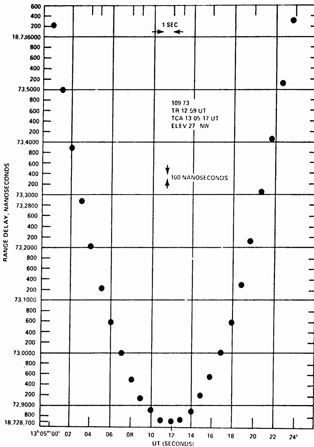
Figure 15. Propagation Delay During Satellite Pass
