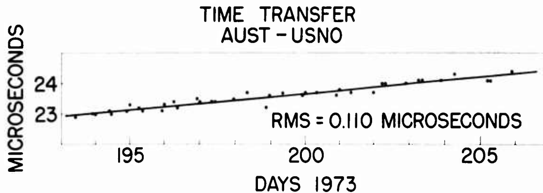
Figure 11. Time Differences Obtained from Figure 10
