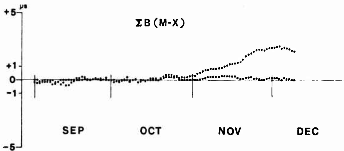
Figure 2. Theoretical and real relative time scales between the Master Station (Simeri Crichi) and X slave station (Lampedusa) as received at the Cagliari Monitor Station.
