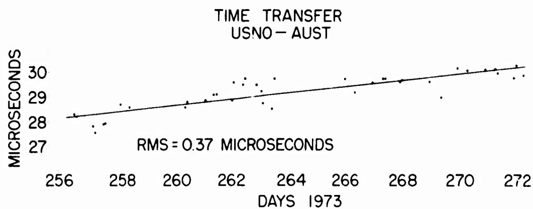
Figure 13. Time Differences Obtained from Figure 12
