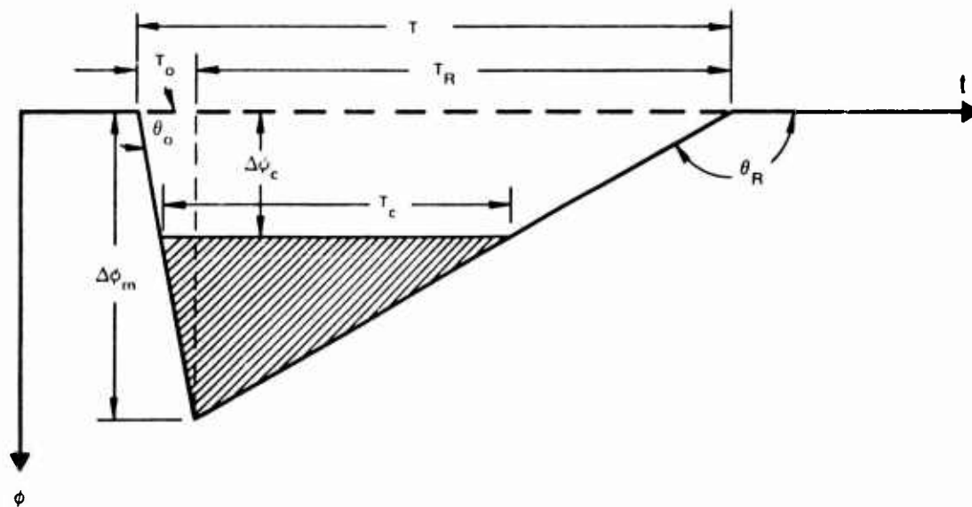
Figure 7. Idealized SPA Shape With Reference Level
