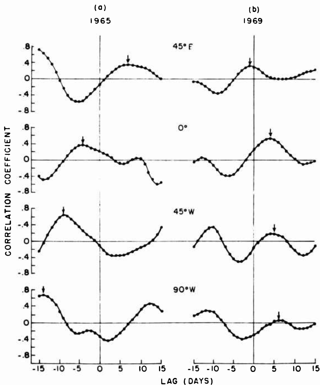
Figure 6. Correlations Between (a) the GBR-APL Phase Variations and the 10 mb Geopotential Height Data in 1965 and (b) the GBR-USNO Phase Variations and 10 mb Geopotential Height Data in 1969 for Several Longitudes.
