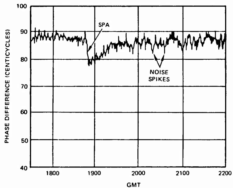
Figure 1. Typical VLF Phase Disturbance Caused by Solar X-ray Flare
