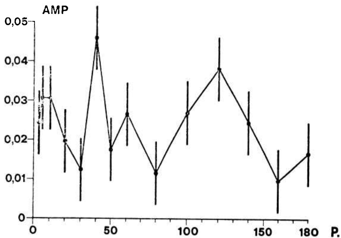
Figure 6. Spectral Analysis of the daily relative frequency rates B (M - Z) versus period in days.
