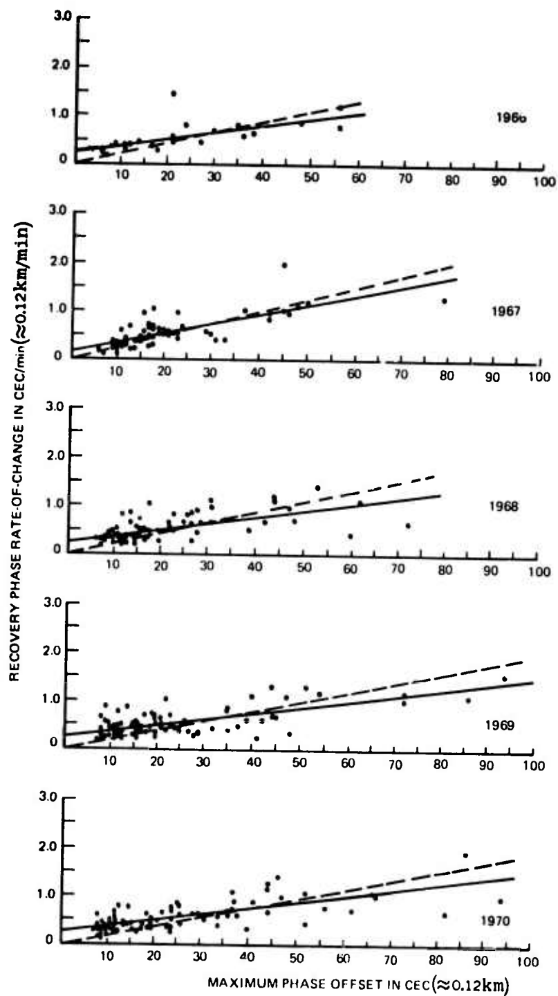
Figure 13. Recovery Phase Rate-or-Change vs. Maximum Phase Offset for SPA Events on Hawaii to New York Path at 10.2 kHz
