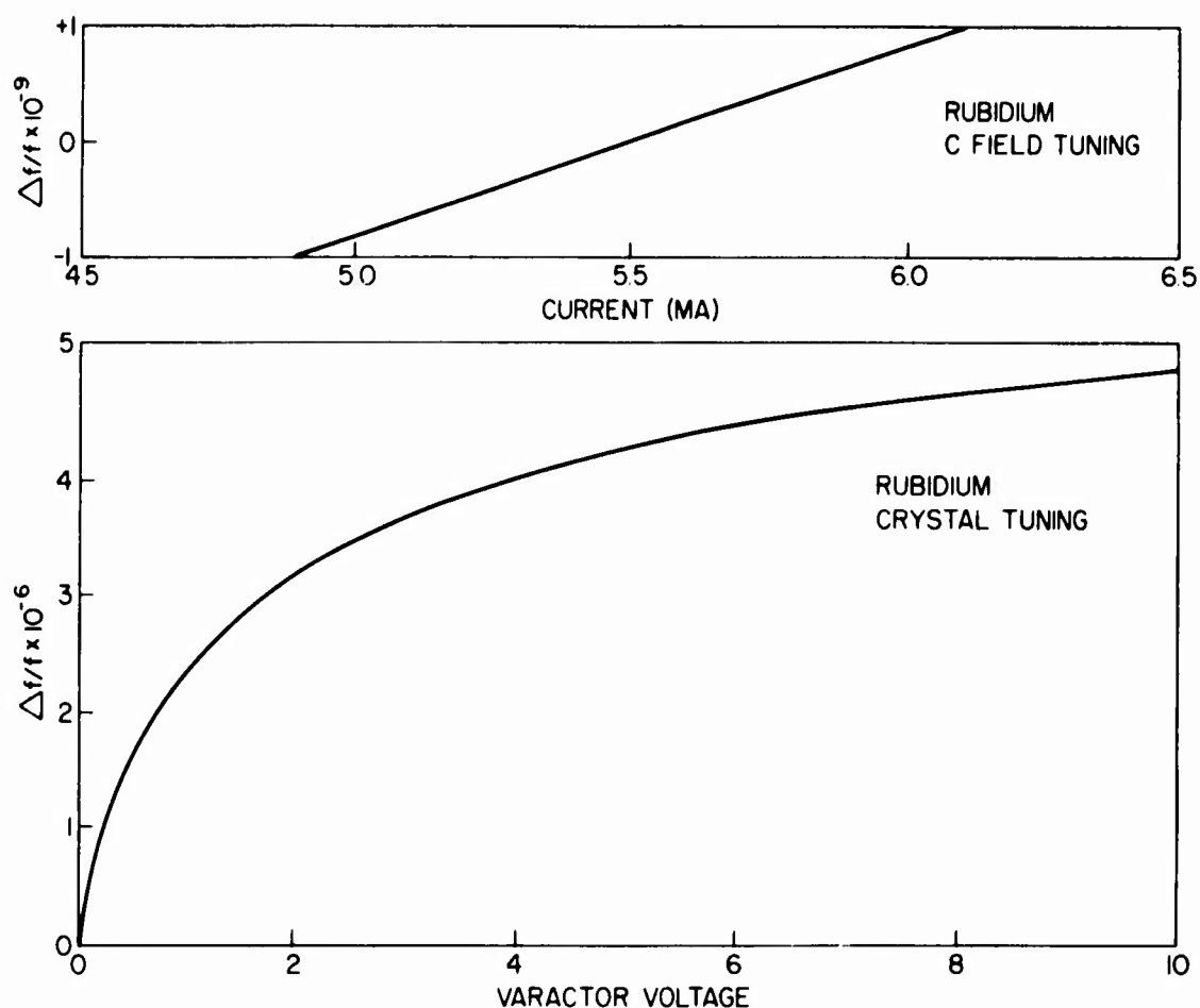
Figure 10. Rubidium Tuning Curves
