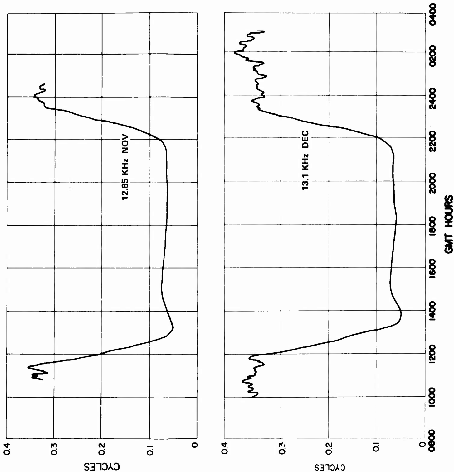
Figure 5. Daytime Seasonal Variations of the Omega Signals from North Dakota to Greenbelt, Maryland (GSFC), June through December 1973
