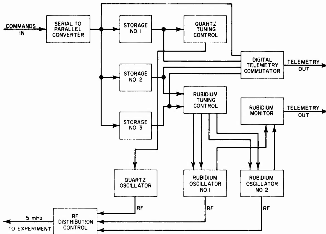
Figure 4. Logic and Tuning Control Block Diagram
