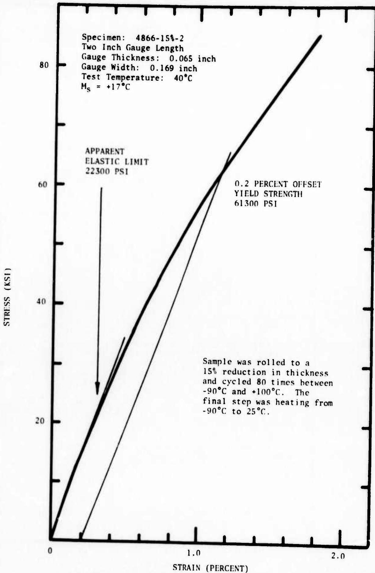
Figure 25. Stress-Strain Curve for 55 w/o Ni-45 w/o Ti at 40°C after Cold Work and Cycling.
