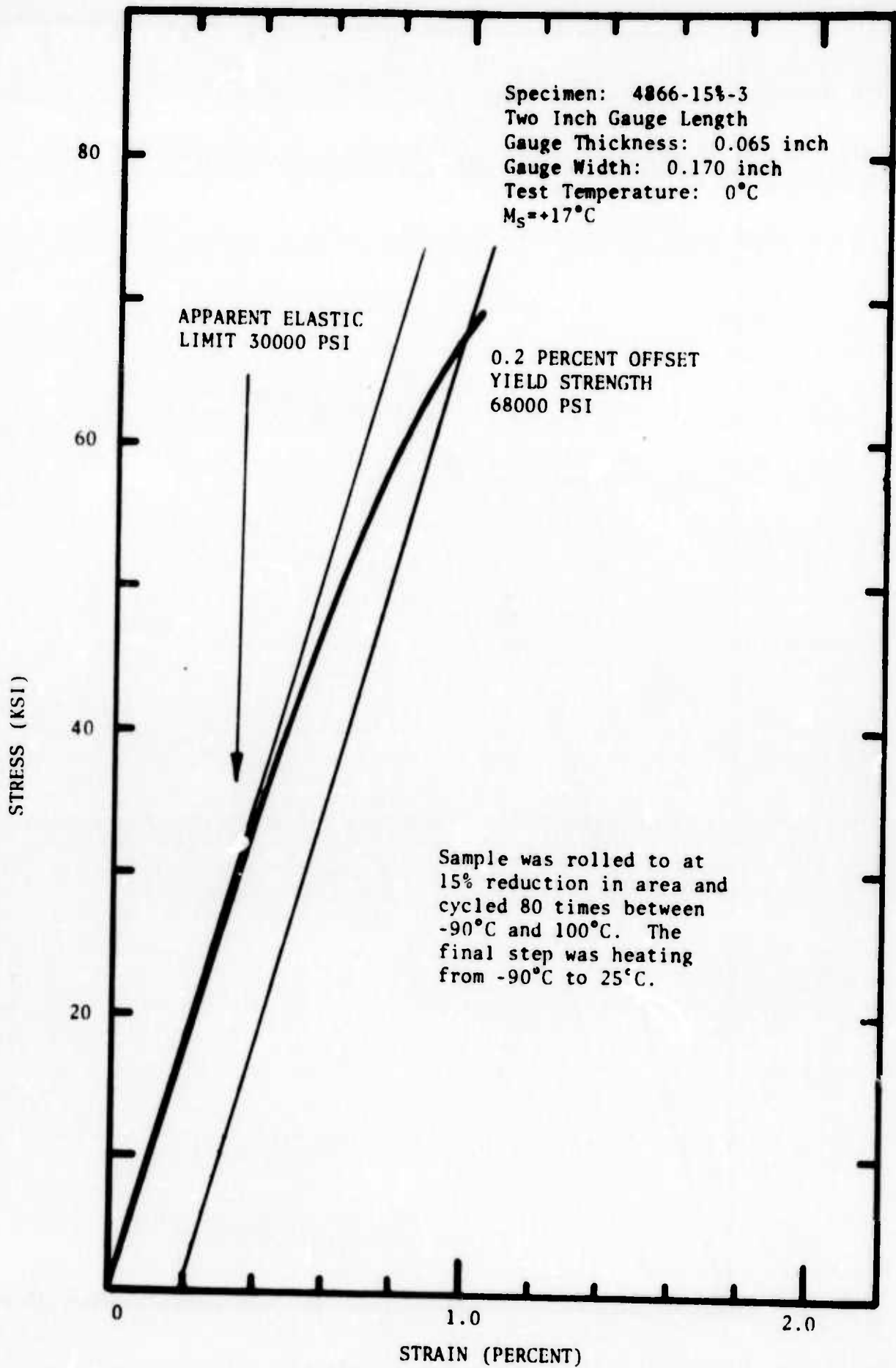
Figure 23. Stress-Strain Curve for 55 w/o Ni-45 w/o Ti at 0°C after Cold Work and Cycling.
