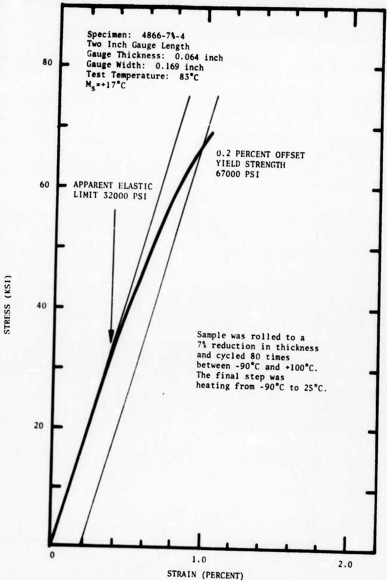
Figure 22. Stress-Strain Curve for 55 w/o Ni-45 w/o Ti at 83°C after Cold Work and Cycling.
