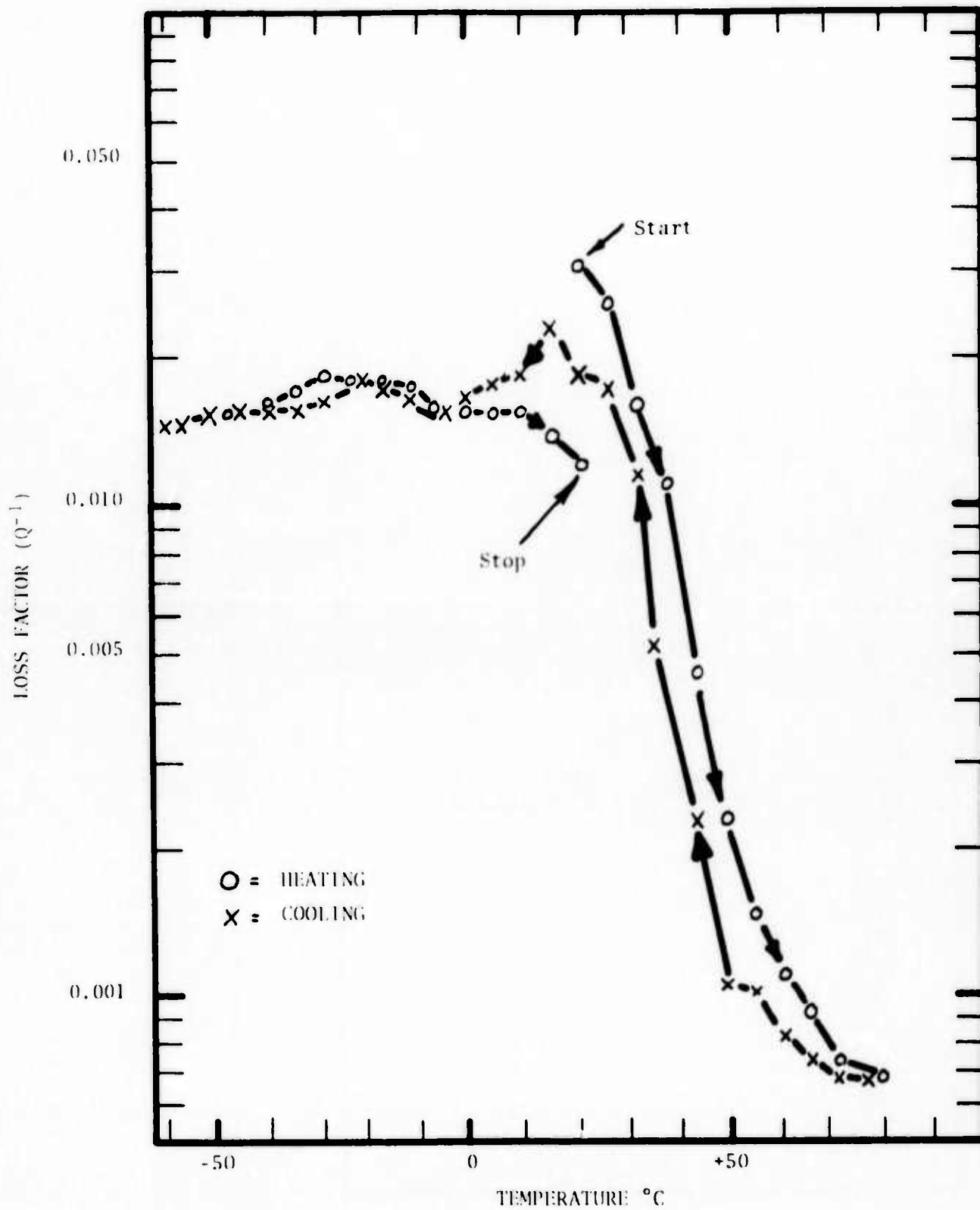
Figure 41. Loss Factor vs. Temperature Curve for a Sample of 55 w/o Ni-45 w/o Ti measured at 160-190 Hertz and a Stress of 2000 psi. The sample was cycled 80 times between -90°C and +100°C prior to testing. The final cycle ended by heating from -90°C to 25°C. The M_g is at +17°C.
