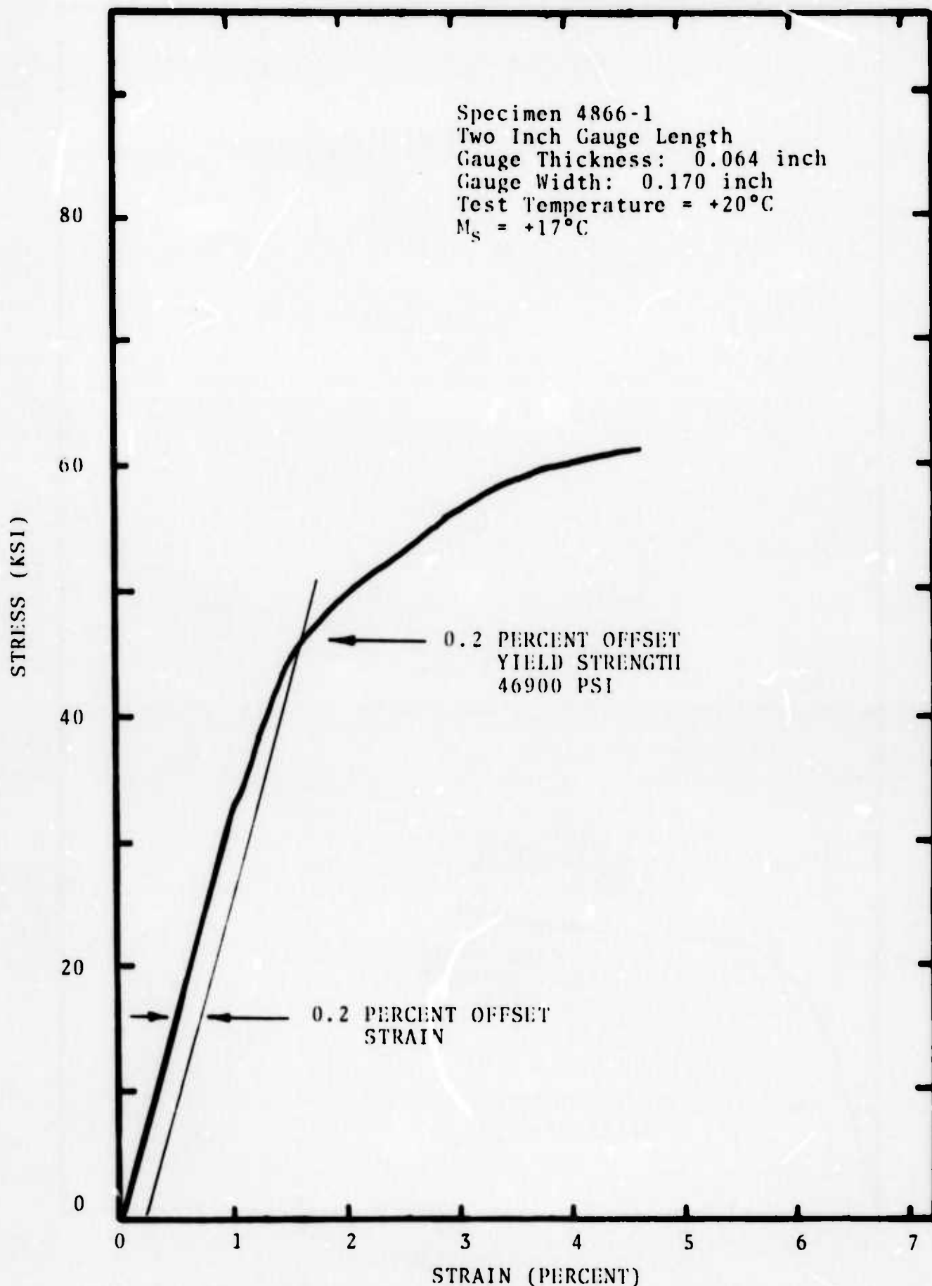
Figure 11. Stress-strain curve for 55 w/o Ni-45 w/o TI Alloy at +20°C after 50 temperature cycles between -65°C and +90°C. The final step was heating from -65°C to 25°C.
