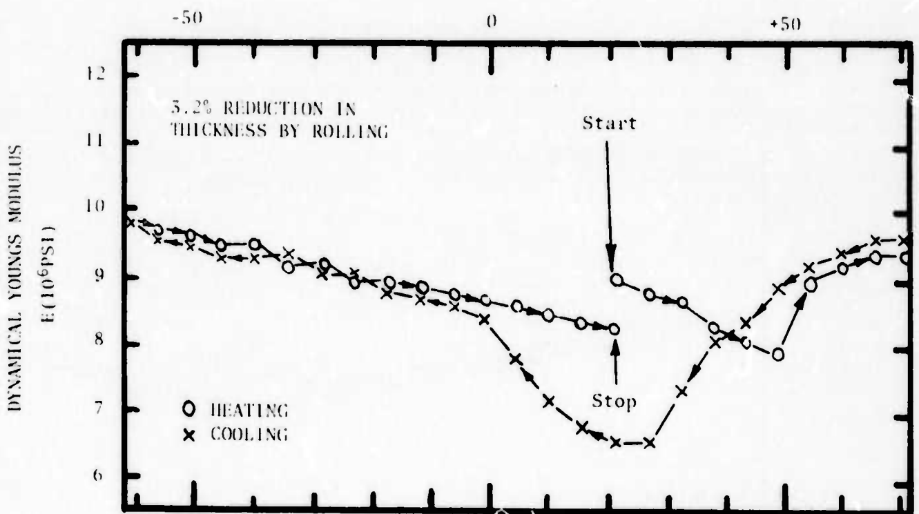
Figure 45. Dynamical Youngs Modulus vs. Temperature for 55 w/o Ni-45 w/oTi measured at 145-190 Hertz at a Stress of 2000 psi. The lower sample was deformed 3.2% by rolling prior to 80 cycles between -90°C and +100°C before testing. The final cycle ended by heating from -90°C to 25°C. The M_s is at +17°C.
