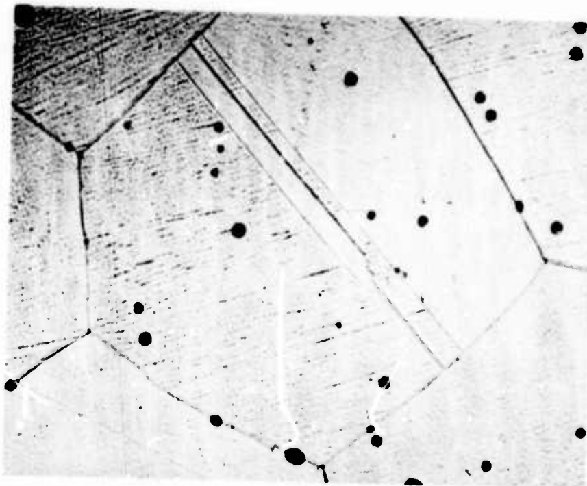
Figure 54. 82 w/o Co-13 w/o Fe Alloy Annealed at 1000°C Air Cooled to 25°C. Etched in 5% Nital. Photomicrograph Shows Twinned Austenitic Structure (X1000).
