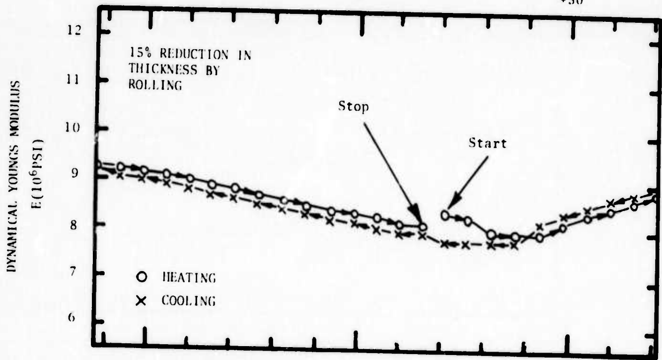
Figure 46. Dynamical Youngs Modulus vs. Temperature for 55 w/o Ni-45 w/o Ti measured at 155-190 Hertz at a Stress of 2000 psi. Both samples were deformed by rolling prior to 80 cycles between -90°C and +100°C before testing. The final cycle ended by heating from -90°C to 20°C. The M_s is at +17°C.
