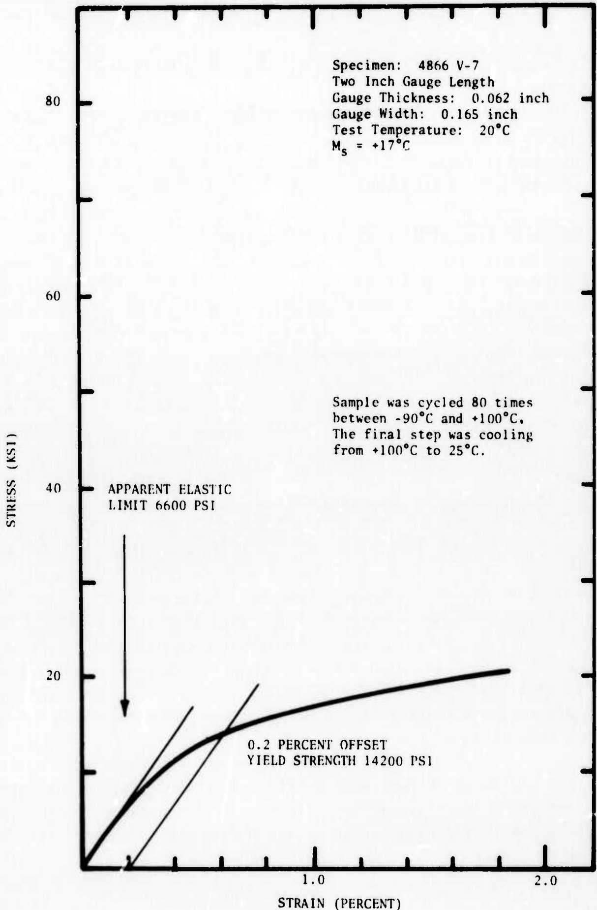
Figure 15. Stress-Strain Curve for 55 w/o Ni-45 w/o Ti at 20°C after Cycling.
