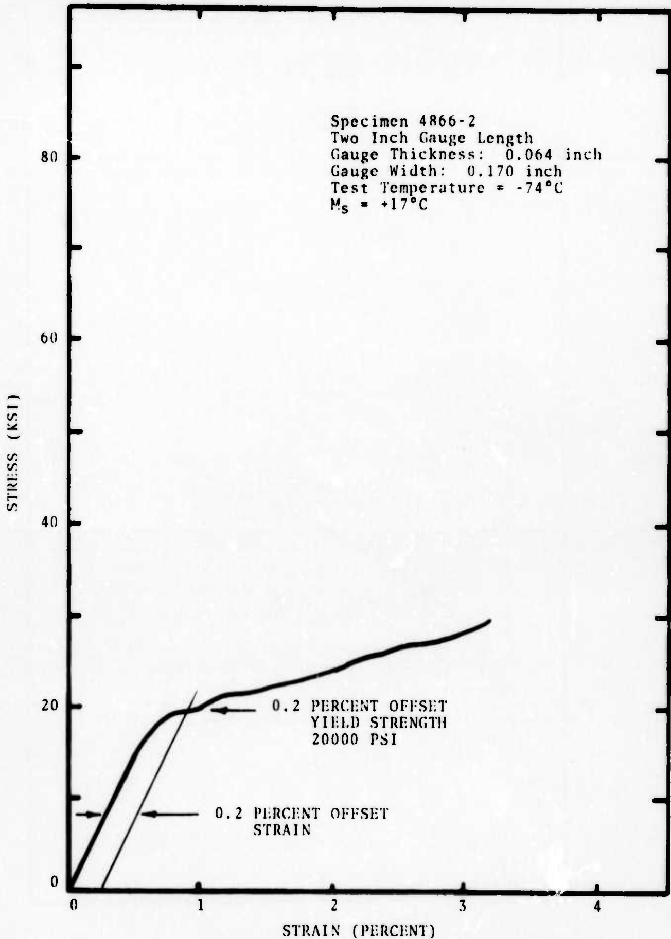
Figure 13. Stress-strain curve for 55 w/o Ni-45 w/o Ti Alloy at -74°C after 50 temperature cycles between -65°C and +90°C. The final step was heating from -65°C to 25°C.
