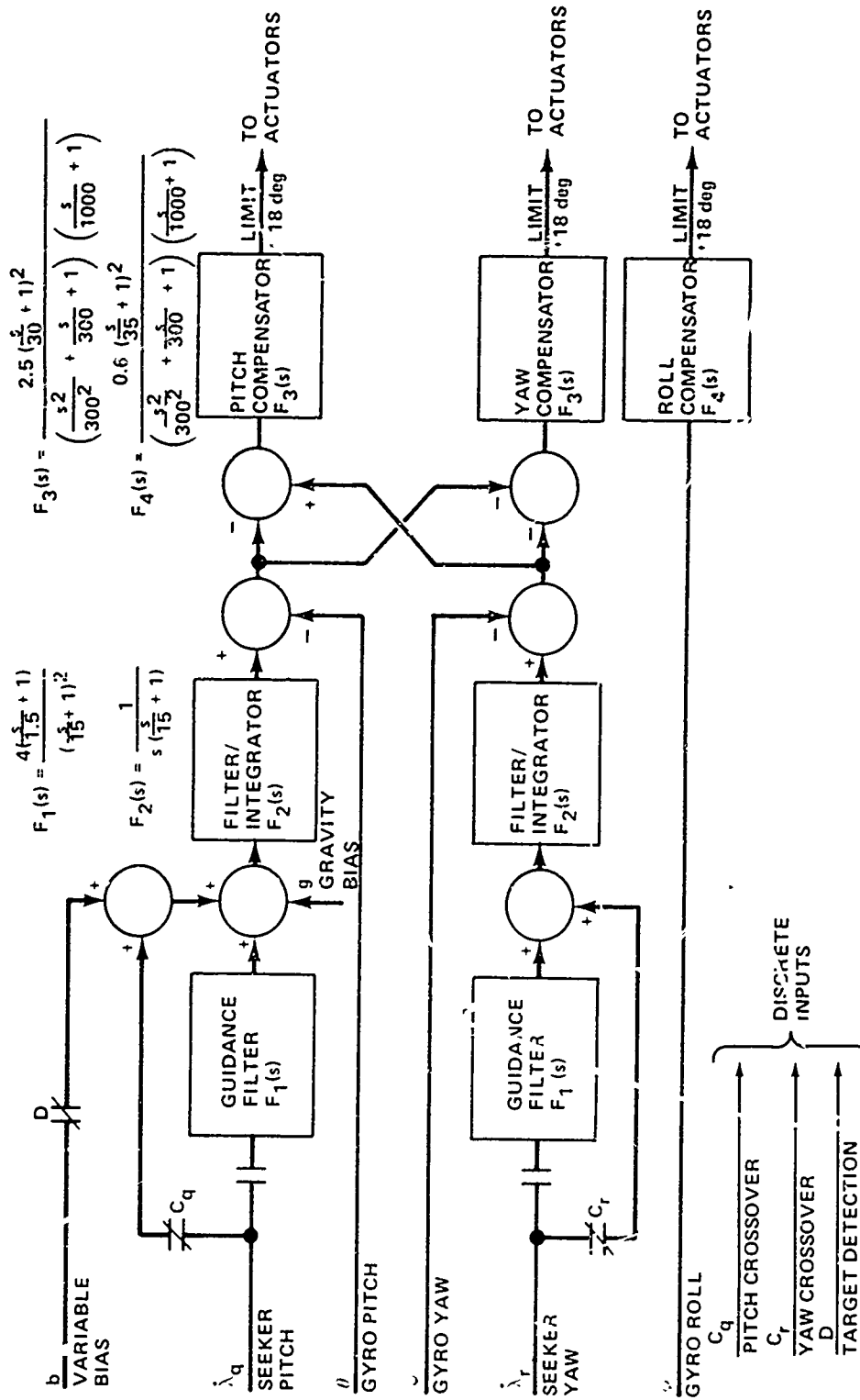
Figure A-1. Analog functions to be implemented digitally.
