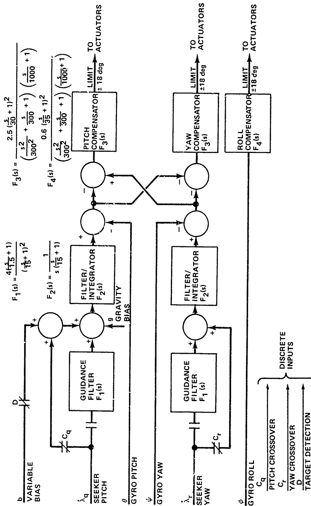
Figure 1. Analog functions to be implemented digitally.
