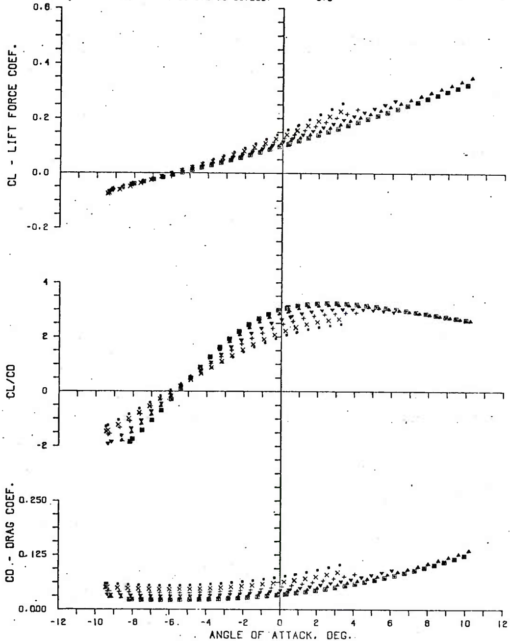
Figure A7. Concluded
