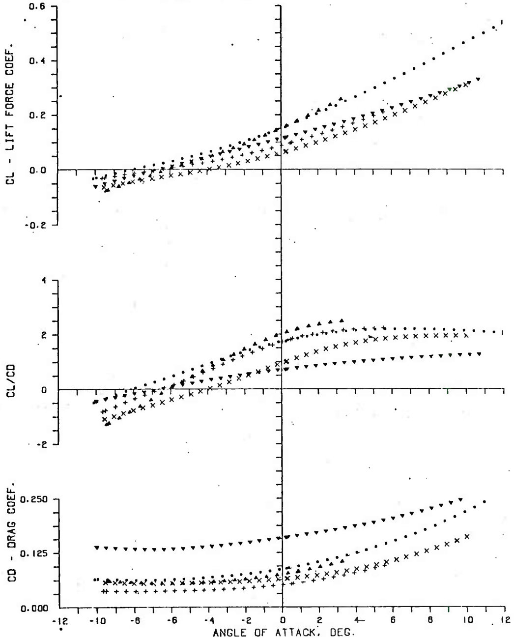
Figure A6. Variation of C_L , C_D , C_L/C_D With Configuration at Constant Mach Number
