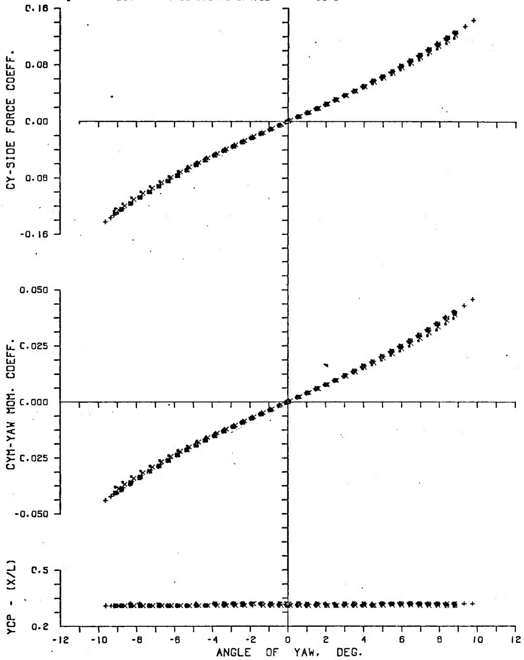
Figure A4. Continued e. Configuration 972.8
