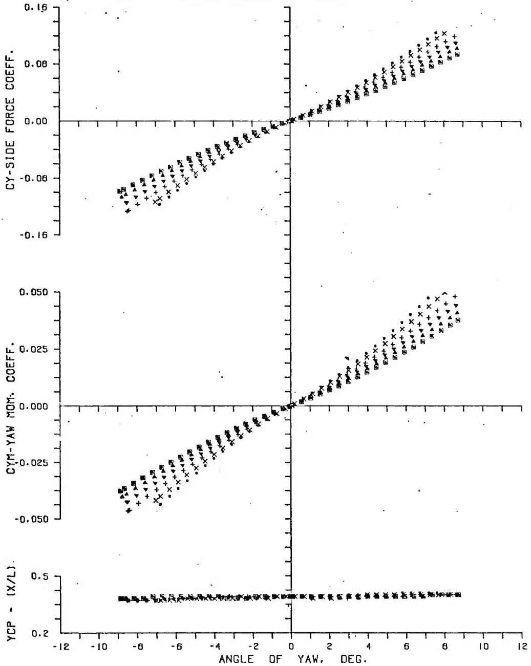
Figure A4. Continued d. Configuration 972.7
