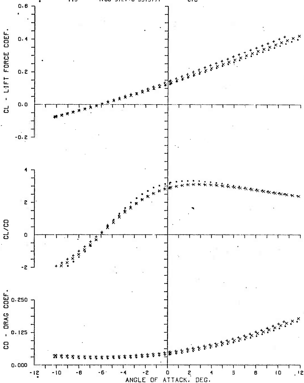
Figure A7. Continued b. Configuration 972.1
