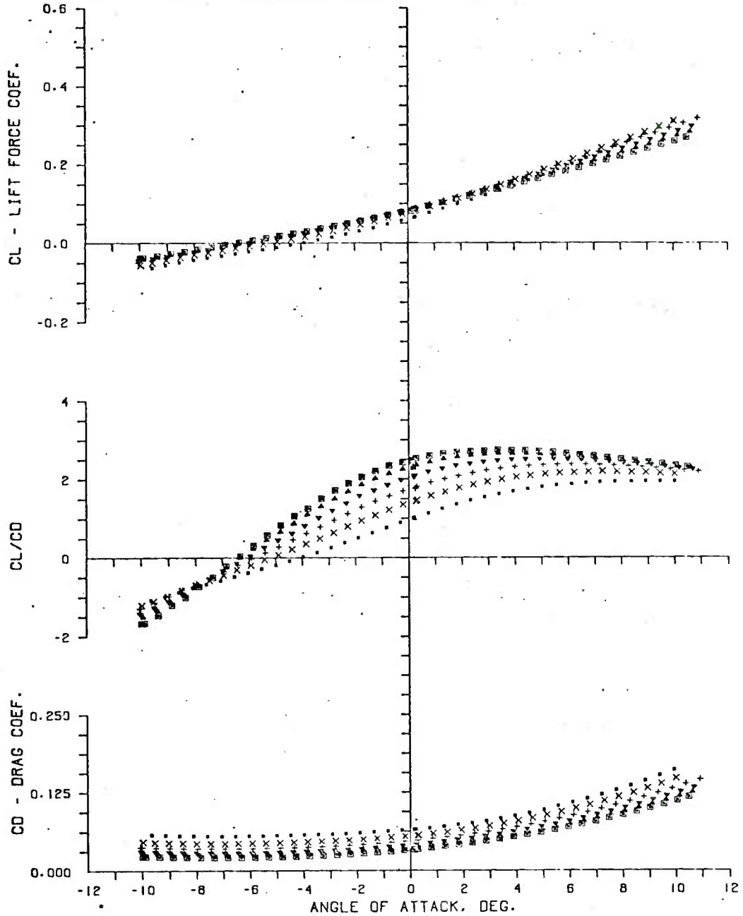
Figure A7. Continued c. Configuration 972.6
