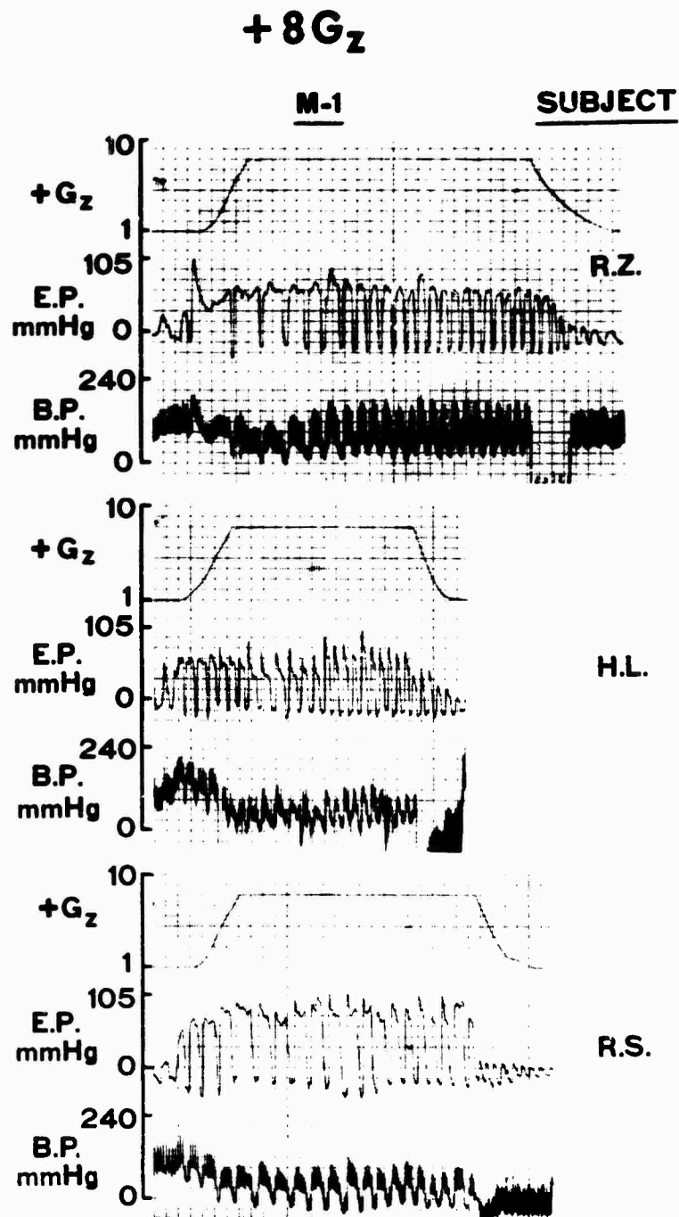
Figure 23. Physiologic changes at +8 G z while subjects are positive-pressure breathing (PPB, 30 mm Hg), or using the M-1 maneuver. Esophageal pressure (E.P.) is used as an indication of straining required to maintain vision. Note that changes in E.P. are reflected in changes in eye-level blood pressure (B.P.). (From Burton, Leverett, and Michaelson, 1974)
