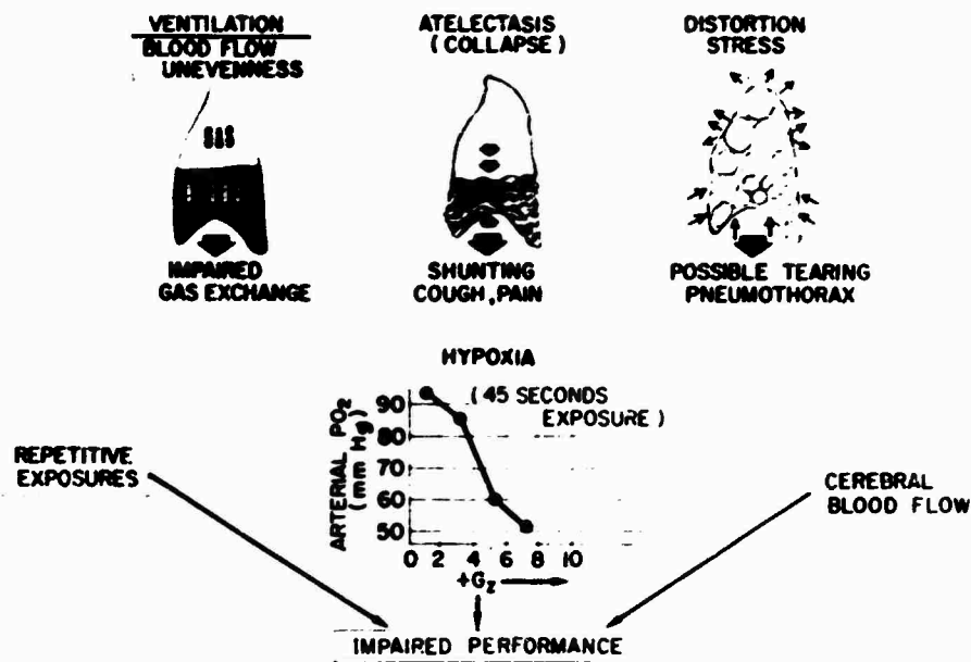
Figure 10. Effects of +G z on the lung.
