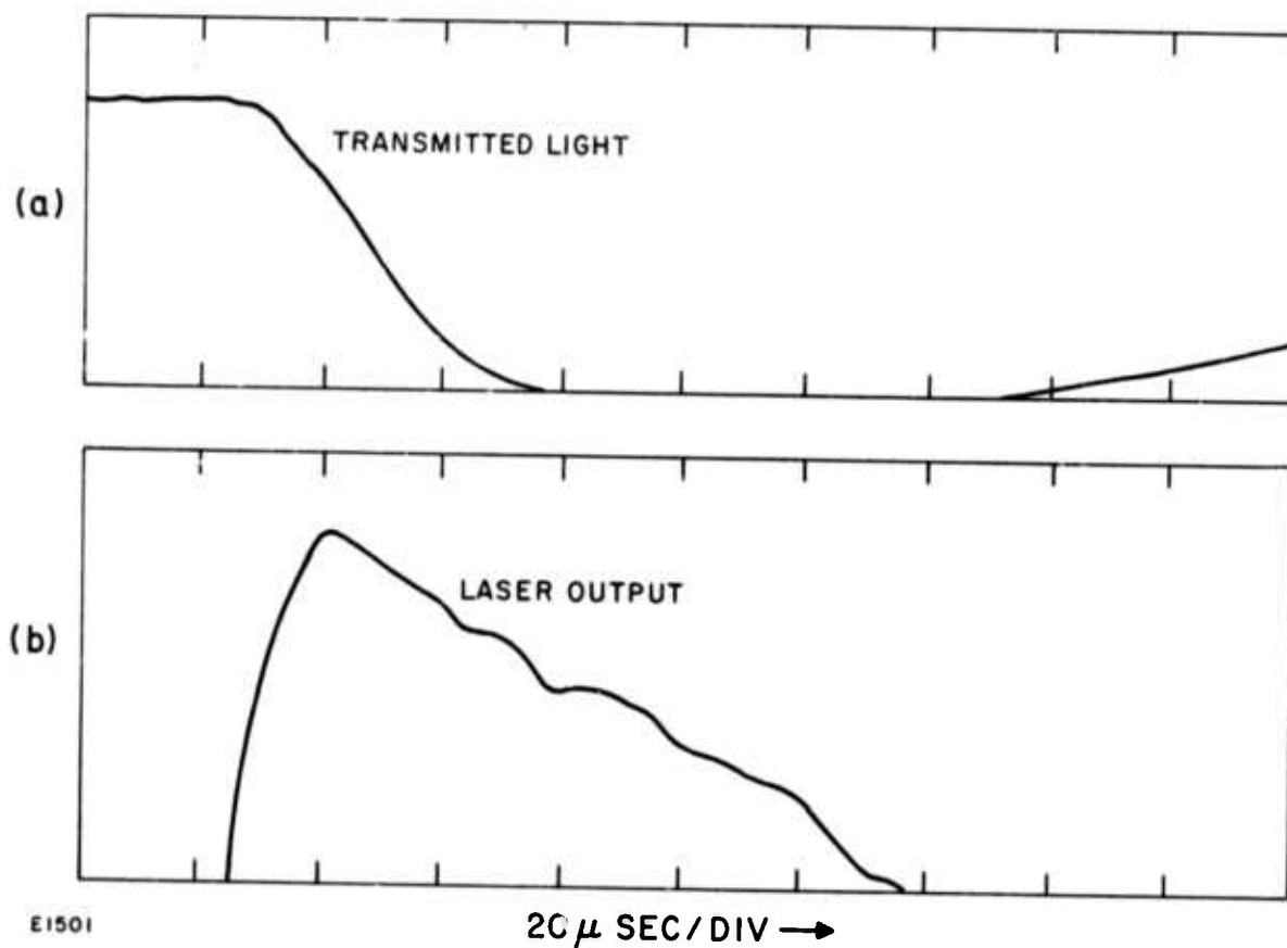
Fig. 6 (a) Transmission of 3093 \text{\AA} Al Light above a Ti Target (b) Laser Output
