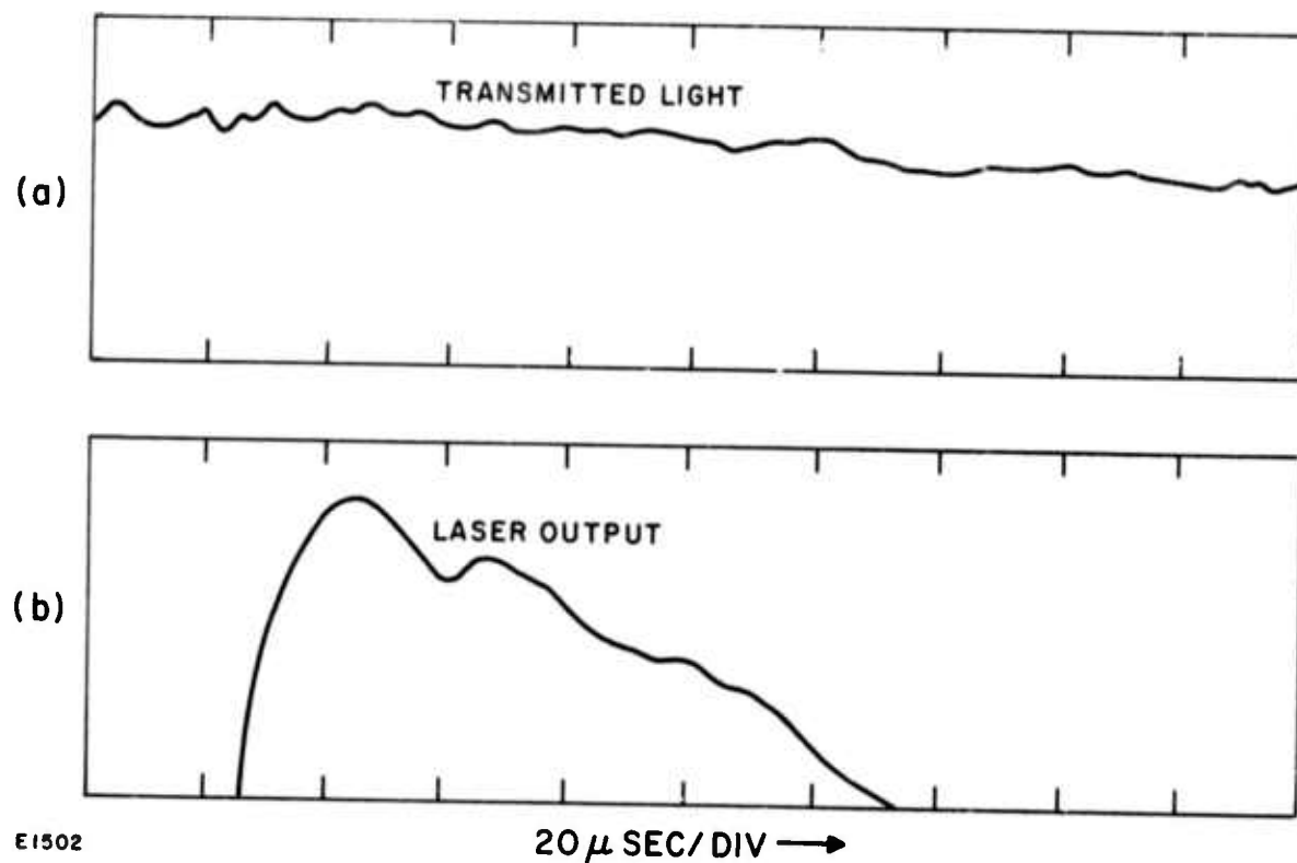
Fig. 5 (a) Transmission of 3076 \text{ \AA} Zn Light above a Ti Target (b) Laser Output
