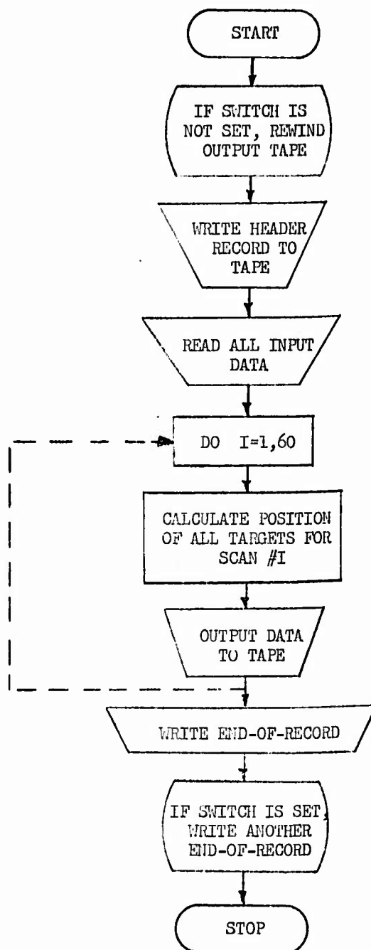
Fig. 8. Tape Generation Program Block Diagram
